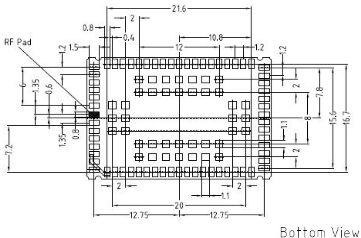
Figure 8: Dimensions of EMS31-V (all dimensions in mm) - bottom view
