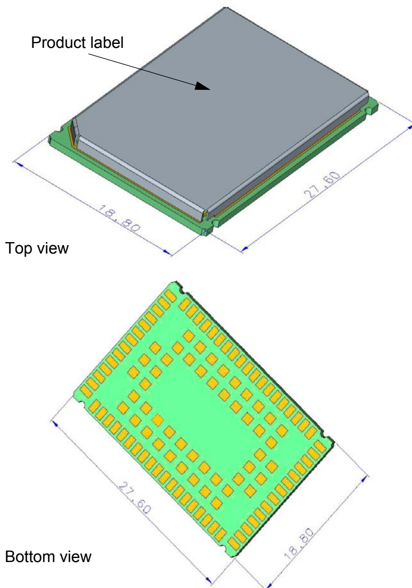
Figure 6: EMS31-V - top and bottom view
