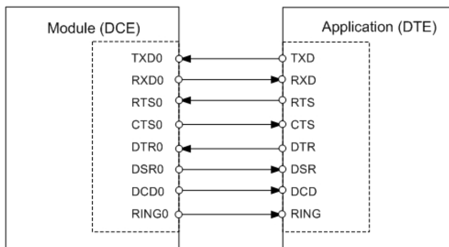
Figure 2: Serial interface ASC0
