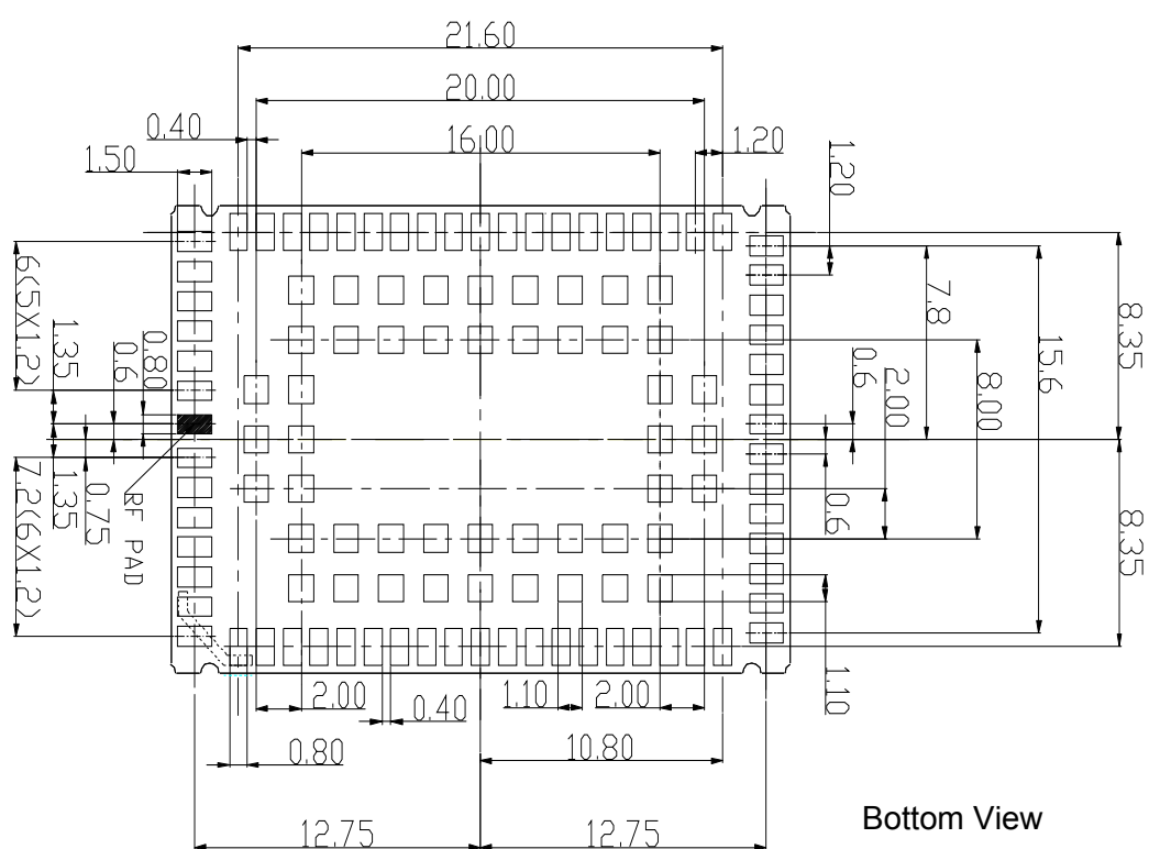
Figure 8: Dimensions of EMS31-X (all dimensions in mm, with tolerance +/-0.1mm) - bottom view
