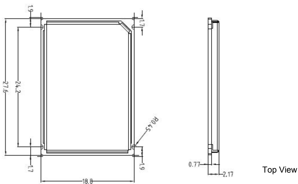
Figure 7: Dimensions of EMS31-X (all dimensions in mm, with tolerance +0.19/-0.1mm)
