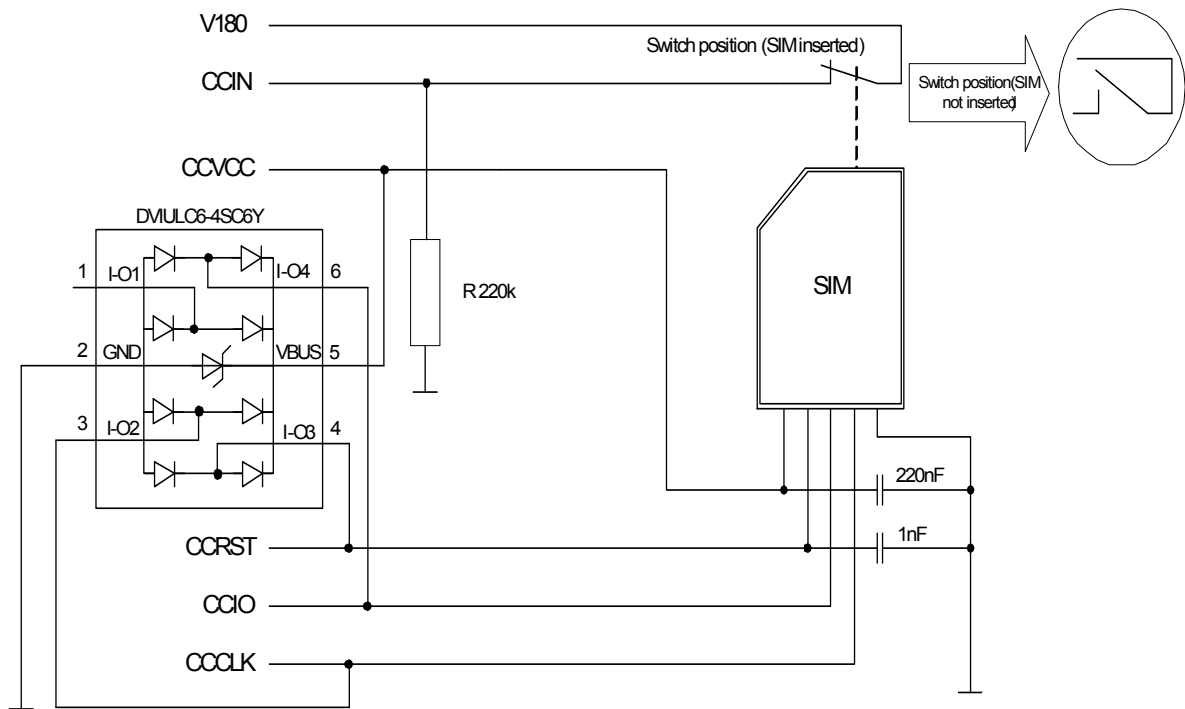
Figure 4: External UICC/SIM/USIM card holder circuit
