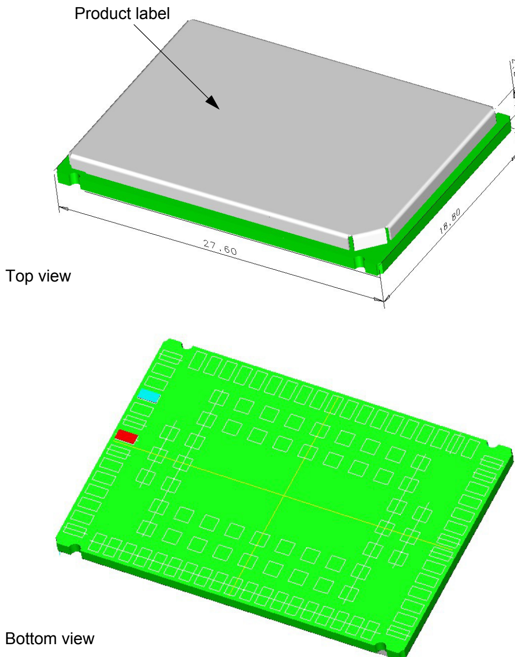
Figure 14: EXS82-W – top and bottom view
