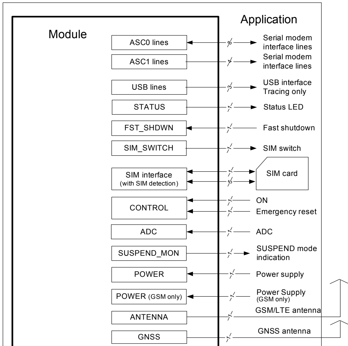
Figure 1: EXS82-W system overview
