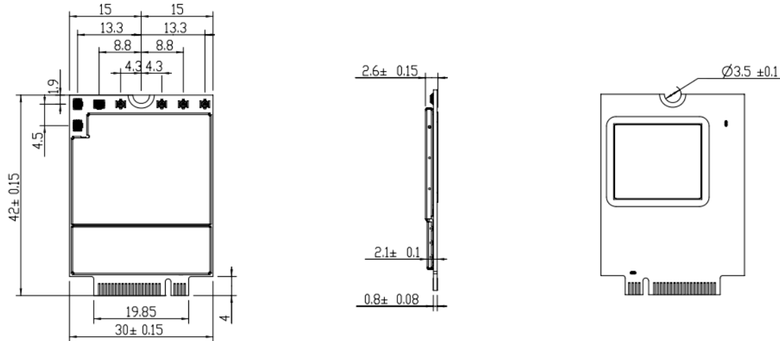
Figure 4: 5G M.2 Data Card MV31-W Dimensions
