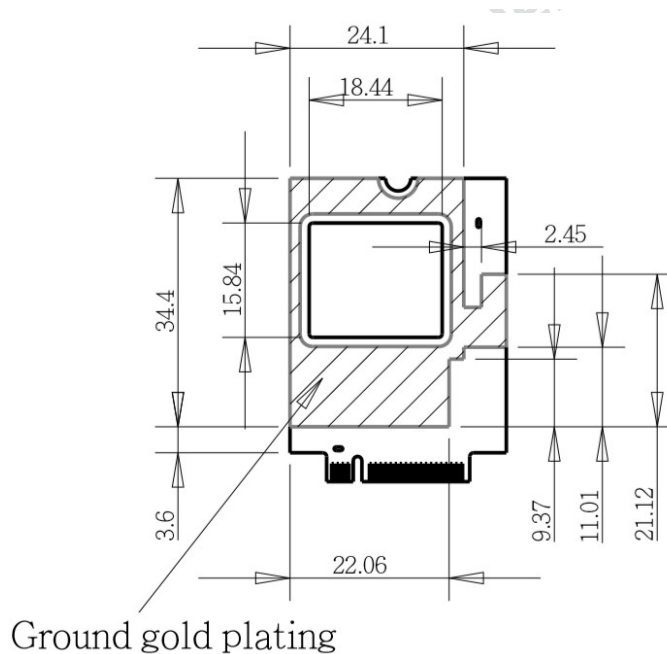
Figure 5: 5G M.2 Data Card MV31-W Ground area (with gold plating) on bottom side
