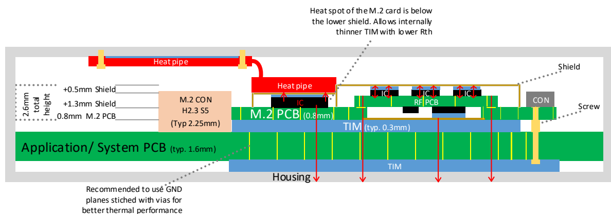
Figure 23: Option 4 - Heat pipe and small application housing
