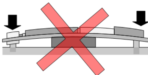
Figure 34: Mounting Advice
