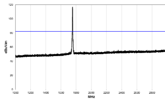
WCDMA – 1752.6MHz
