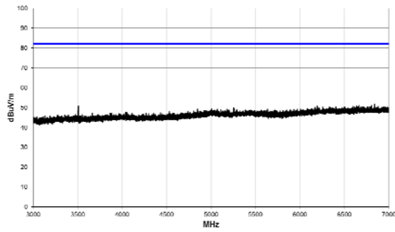
3 GHz – 7 GHz
