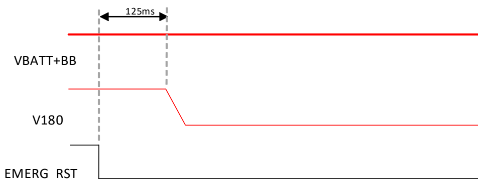
Figure 27: Emergency reset timing
