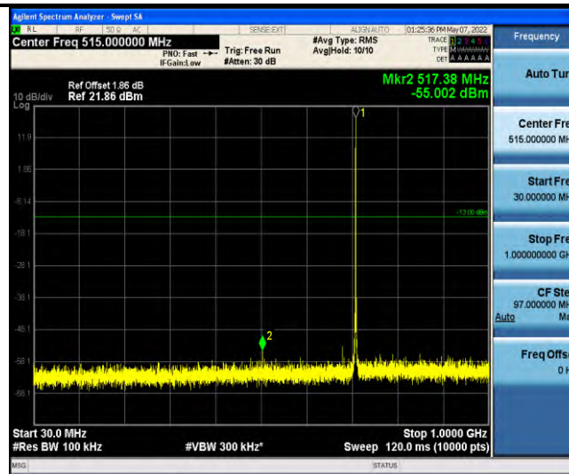
Band12-Stand-Alone-NaN-QPSK-23178-1@0-3.75kHz-30-1000-30~1000MHz@-55dBm--13-PASS
