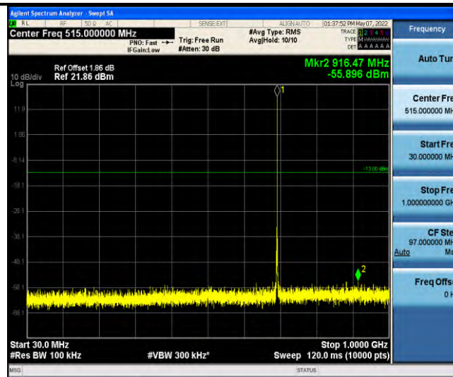
Band12-Stand-Alone-NaB-BPSK-23012-1@11-15kHz-30-1000-30~1000MHz@-55.9dBm--13-PASS
