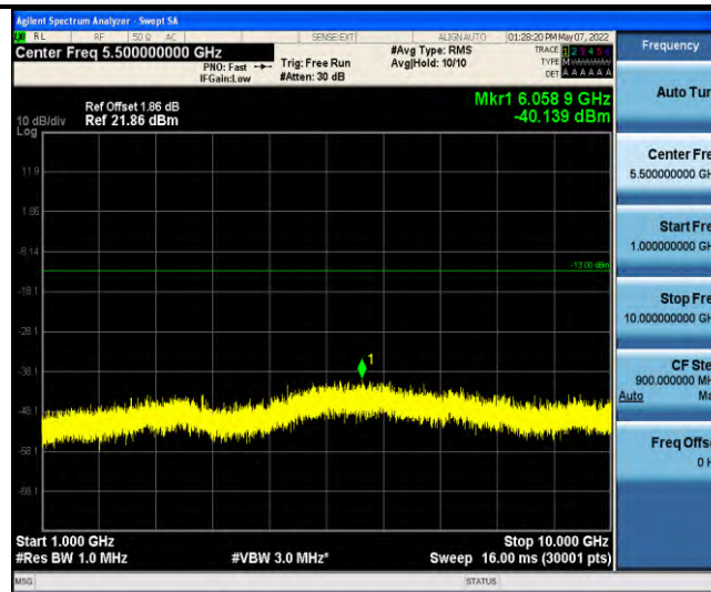
Band12-Stand-Alone-NaN-QPSK-23012-12@0-15kHz-1000-10000-1000~10000MHz@-40.14dBm--13-PASS
