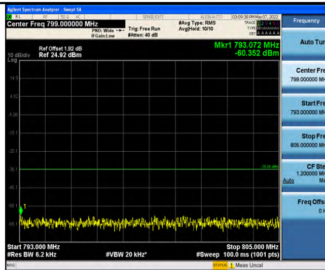
Band13-Stand-Alone-NaN-BPSK-23278-1@11-15kHz-793-805-793~805MHz@-60.35dBm--35-PASS
