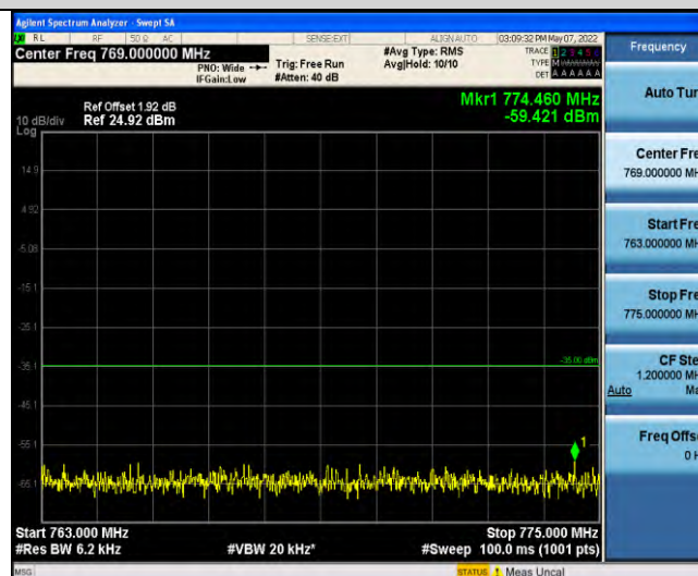
Band13-Stand-Alone-NaN-BPSK-23278-1@11-15kHz-763-775-763~775MHz@-59.42dBm--35-PASS
