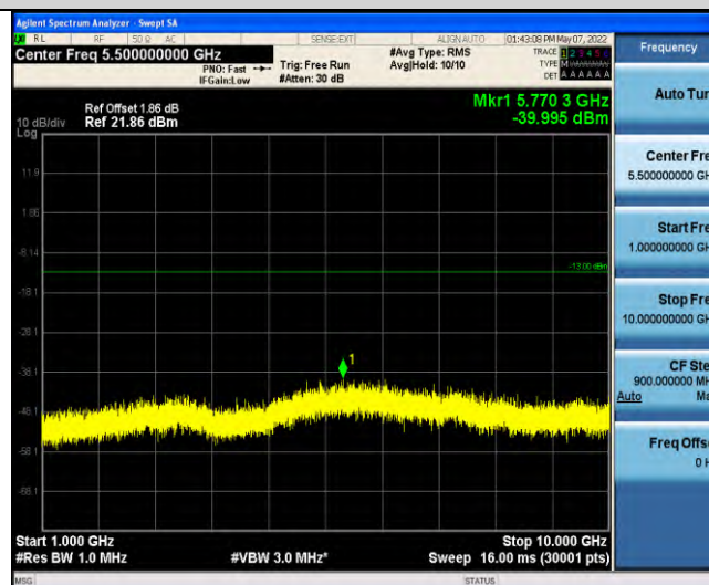
Band12-Stand-Alone-NaN-BPSK-23178-1@11-15kHz-1000-10000-1000~10000MHz@-40dBm--13-PASS
