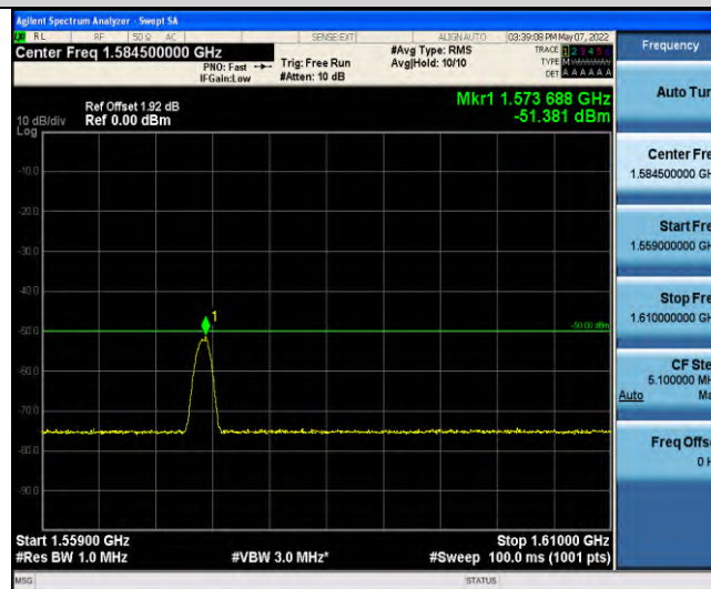
Band13-Stand-Alone-NaN-BPSK-23278-1@0-15kHz-1559-1610-1559~1610MHz@-51.38dBm--50-PASS
