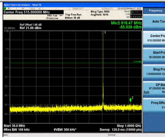
Band12-Stand-Alone-NaN-BPSK-23178-1@11-15kHz-30-1000-30~1000MHz@-55.54dBm--13-PASS
