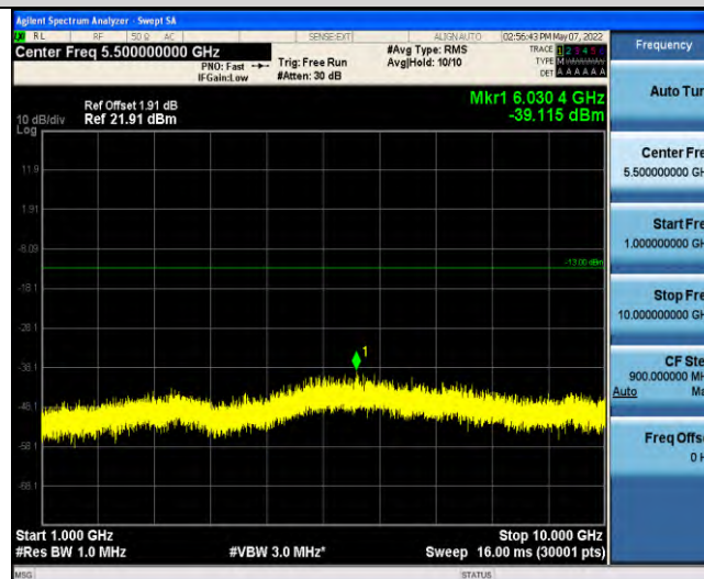
Band13-Stand-Alone-NaN-QPSK-23182-12@0-15kHz-1000-10000-1000~10000MHz@-39.12dBm--13-PASS
