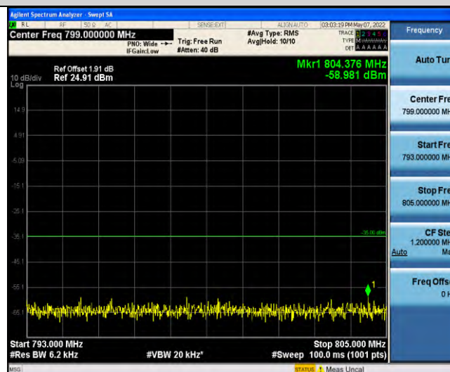
Band13-Stand-Alone-NaN-BPSK-23182-1@11-15kHz-793-805-793~805MHz@-58.98dBm--35-PASS
