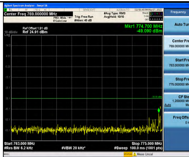
Band13-Stand-Alone-NaN-QPSK-23182-12@0-15kHz-763-775-763~775MHz@-49.09dBm--35-PASS
