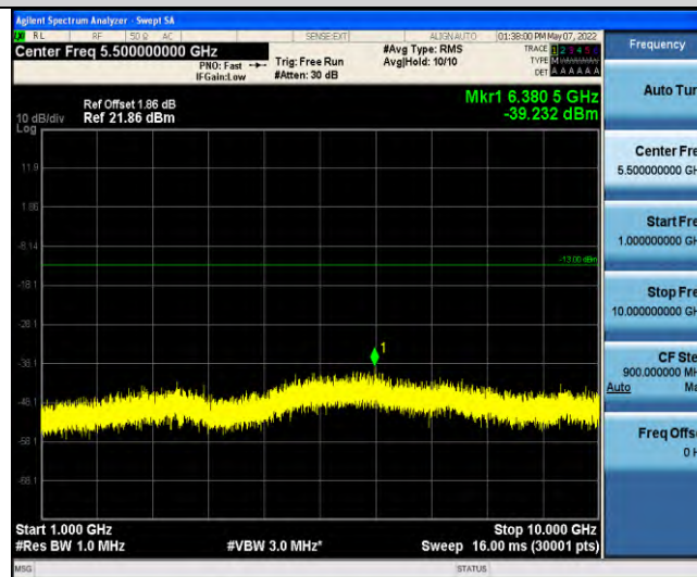
Band12-Stand-Alone-NaB-BPSK-23012-1@11-15kHz-1000-10000-1000~10000MHz@-39.23dBm--13-PASS
