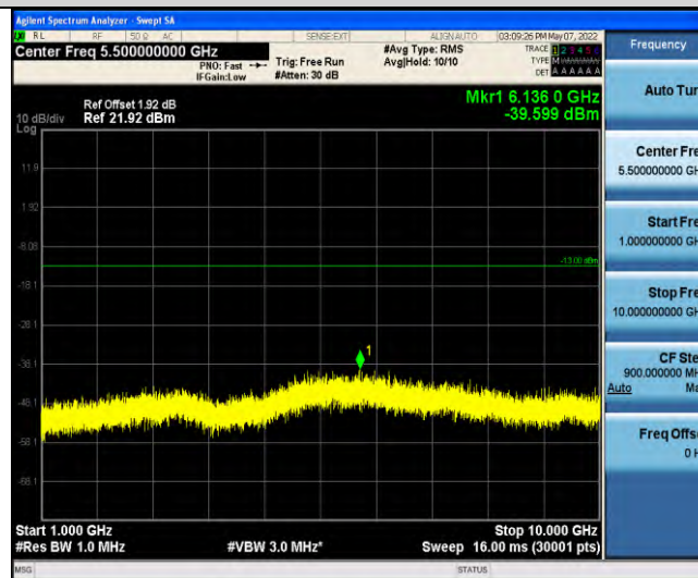
Band13-Stand-Alone-NaN-BPSK-23278-1@11-15kHz-1000-10000-1000~10000MHz@-39.6dBm--13-PASS
