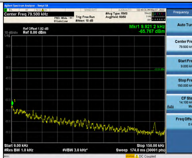
Band13-Stand-Alone-NaN-QPSK-23230-1@0-3.75kHz-0.009-0.15-0.009~0.15MHz@-65.77dBm--33-PASS
