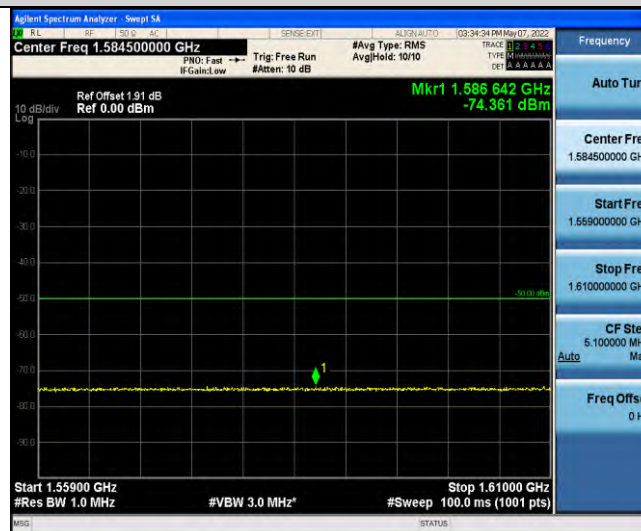
Band13-Stand-Alone-NaN-QPSK-1559-1610-1559~1610MHz@-74.36dBm--50-PASS
