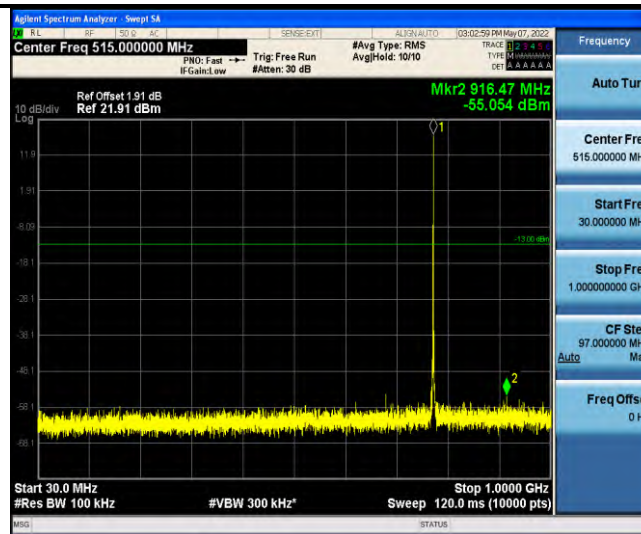
Band13-Stand-Alone-NaN-BPSK-23182-1@11-15kHz-30-1000-30~1000MHz@-55.05dBm--13-PASS
