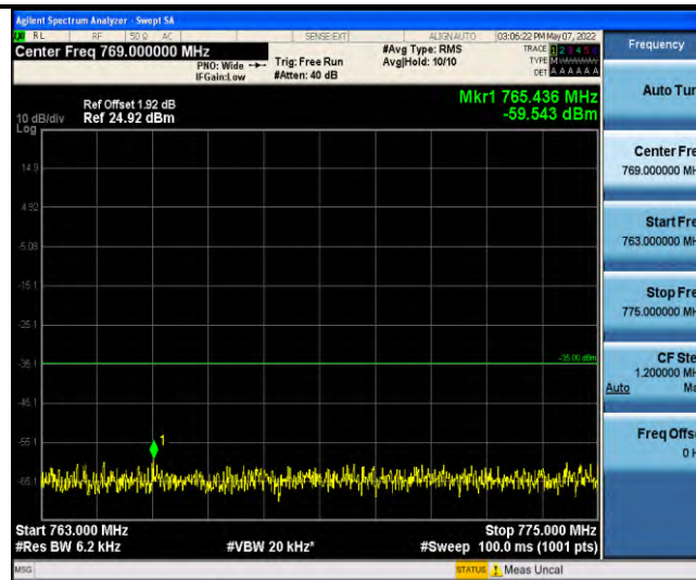
Band13-Stand-Alone-NaB-BPSK-23230-1@11-15kHz-763-775-763-775MHz@-59.54dBm--35-PASS
