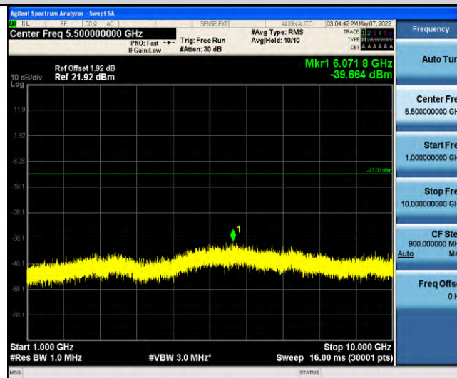
Band13-Stand-Alone-NaN-BPSK-23230-1@0-15kHz-1000-10000-1000~10000MHz@-39.66dBm--13-PASS
