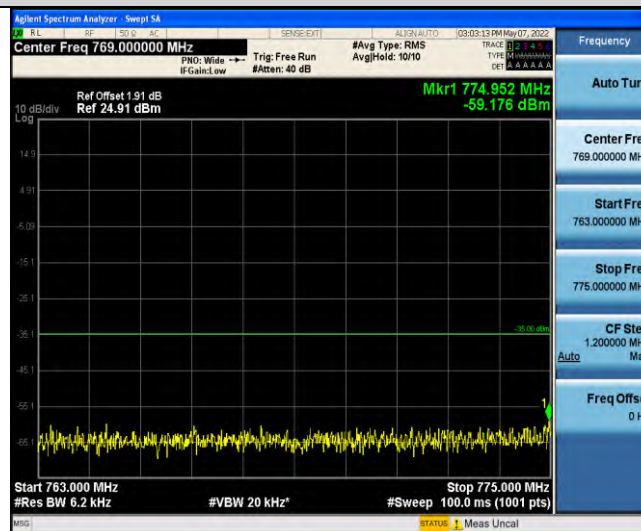
Band13-Stand-Alone-NaN-BPSK-23182-1@11-15kHz-763-775-763~775MHz@-59.18dBm--35-PASS
