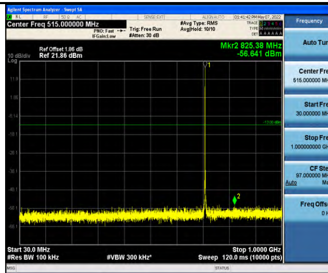
Band12-Stand-Alone-NaN-BPSK-23178-1@0-15kHz-30-1000-30~1000MHz@-56.64dBm--13-PASS
