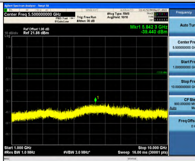
Band12-Stand-Alone-NaN-BPSK-23178-1@0-15kHz-1000-10000-1000~10000MHz@-39.44dBm--13-PASS
