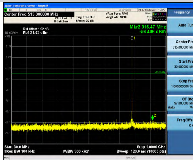
Band13-Stand-Alone-NaN-BPSK-23278-1@11-15kHz-30-1000-30~1000MHz@-56.41dBm--13-PASS
