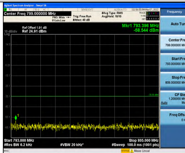
Band13-Stand-Alone-NaN-QPSK-23182-12@0-15kHz-793-805-793~805MHz@-58.54dBm--35-PASS
