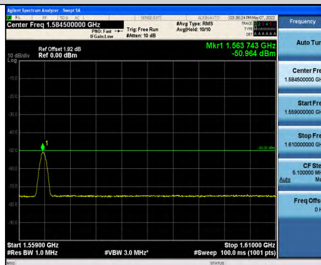
Band13-Stand-Alone-NaN-BPSK-23230-1@0-15kHz-1559-1610-1559~1610MHz@-50.96dBm--50-PASS
