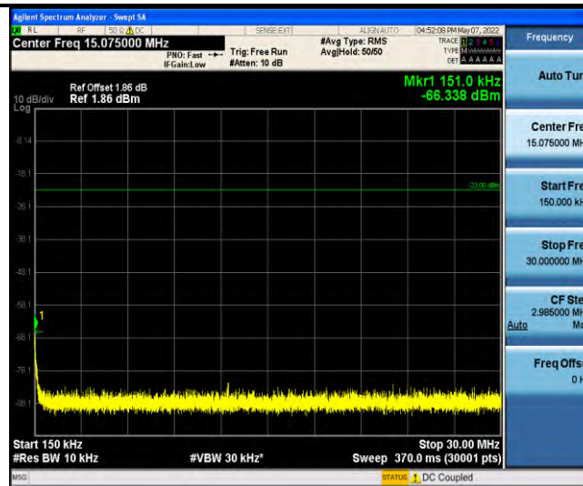
Band17-Stand-Alone-NaN-QPSK-23790-1@0-3.75kHz-0.15-30-0.15-30MHz@-66.34dBm--23-PASS
