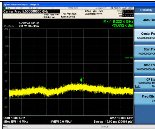
Band12-Stand-Alone-NaN-QPSK-23095-1@47-3.75kHz-1000-10000-1000~10000MHz@-39.69dBm--13-PASS
