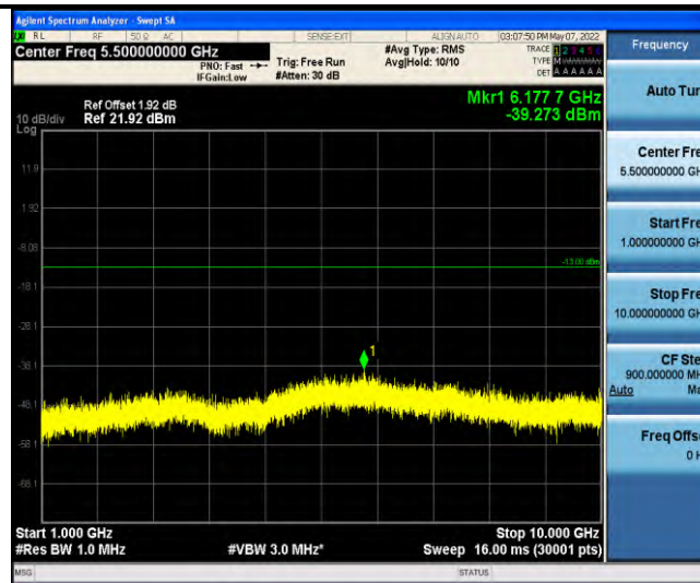
Band13-Stand-Alone-NaN-BPSK-23278-1@0-15kHz-1000-10000-1000~10000MHz@-39.27dBm--13-PASS
