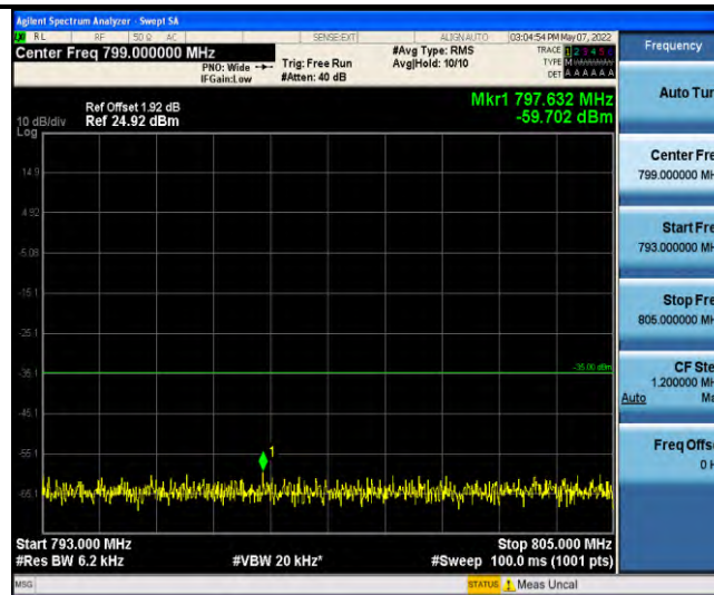
Band13-Stand-Alone-NaN-BPSK-23230-1@0-15kHz-793-805-793~805MHz@-59.7dBm--35-PASS
