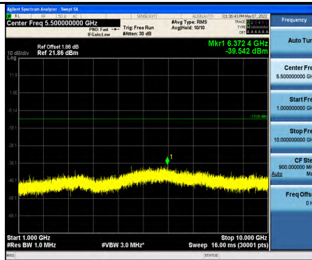
Band12-Stand-Alone-NaN-BPSK-23012-1@0-15kHz-1000-10000-1000~10000MHz@-39.54dBm--13-PASS
