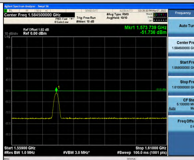
Band13-Stand-Alone-NaN-BPSK-23278-1@11-15kHz-1559-1610-1559~1610MHz@-51.74dBm--50-PASS
