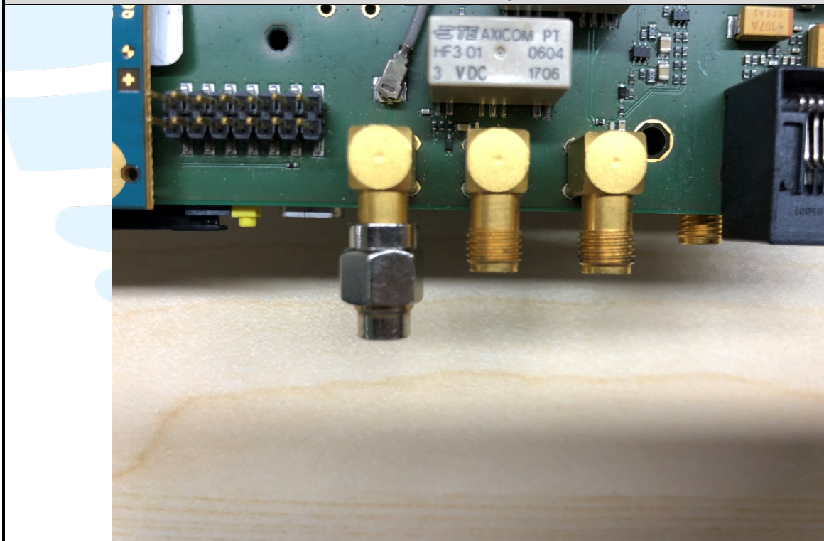
Test Setup
