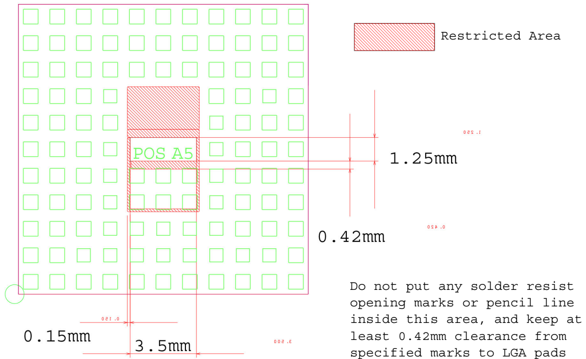
Figure 56: Dimensions of area for possible markings TX82-W, TX62-W-B and TX62-W-C (bottom view)
