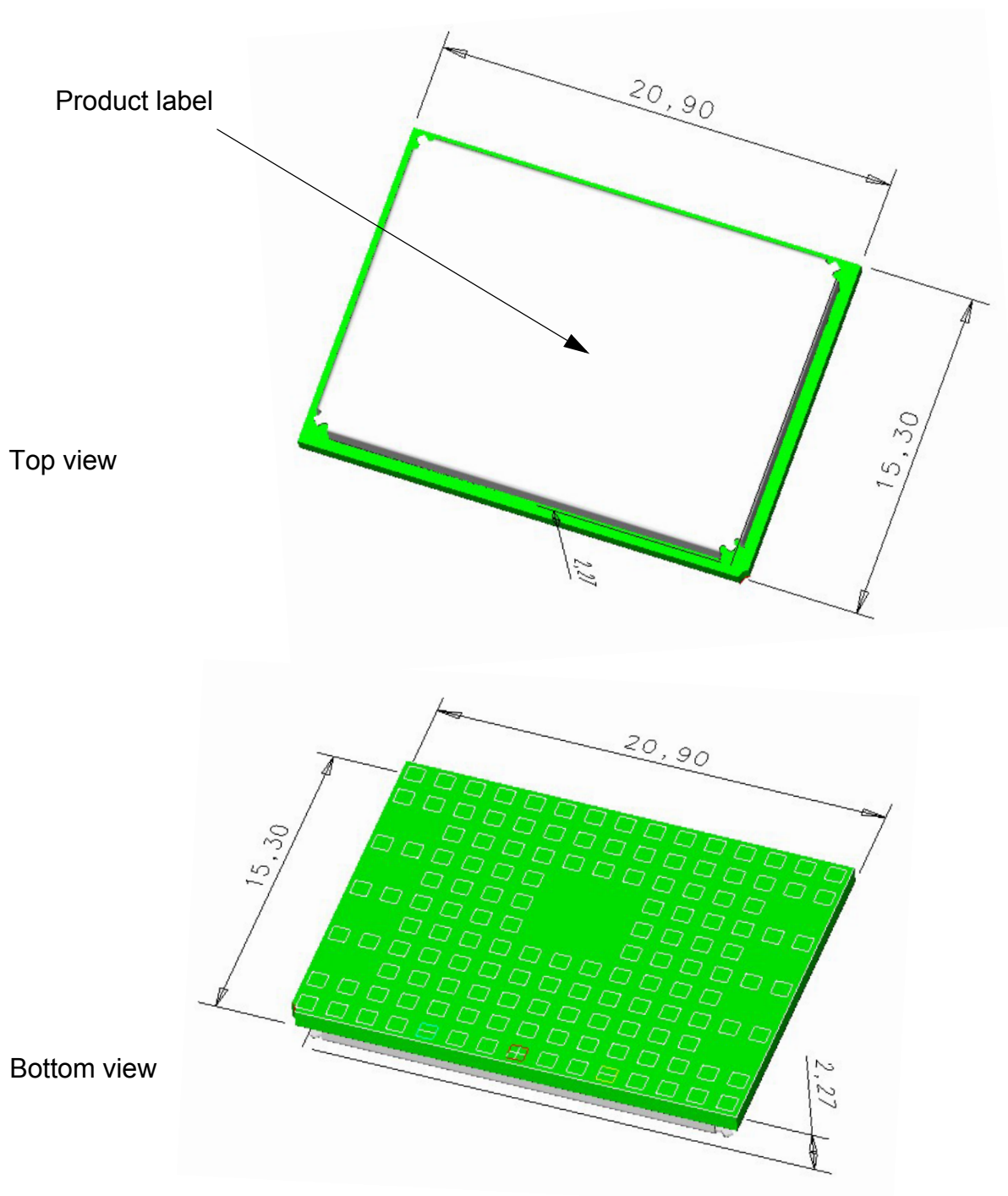
Figure 54: TX82-W– top and bottom view
