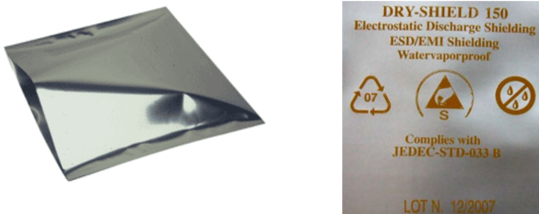
Figure 66: Moisture barrier bag (MBB) with imprint
