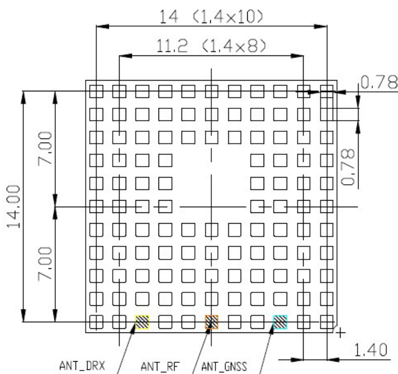
Figure 57: Land pattern TX62-W (top view)
