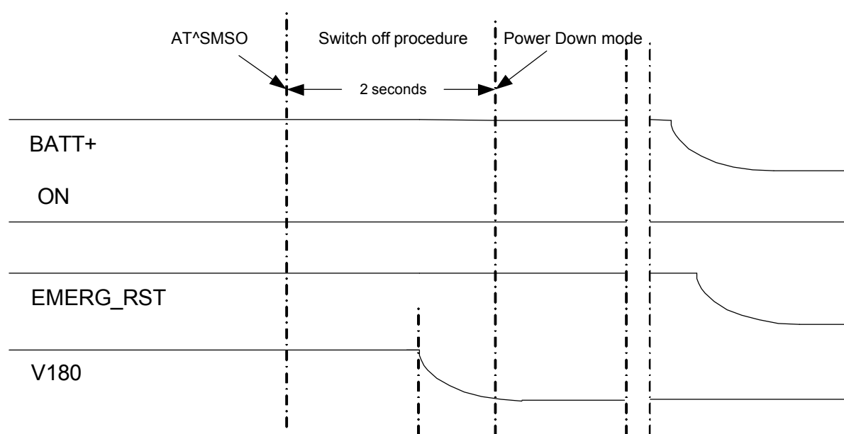
Figure 37: Switch off behavior
