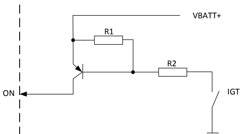
Figure 34: Sample ON circuit
