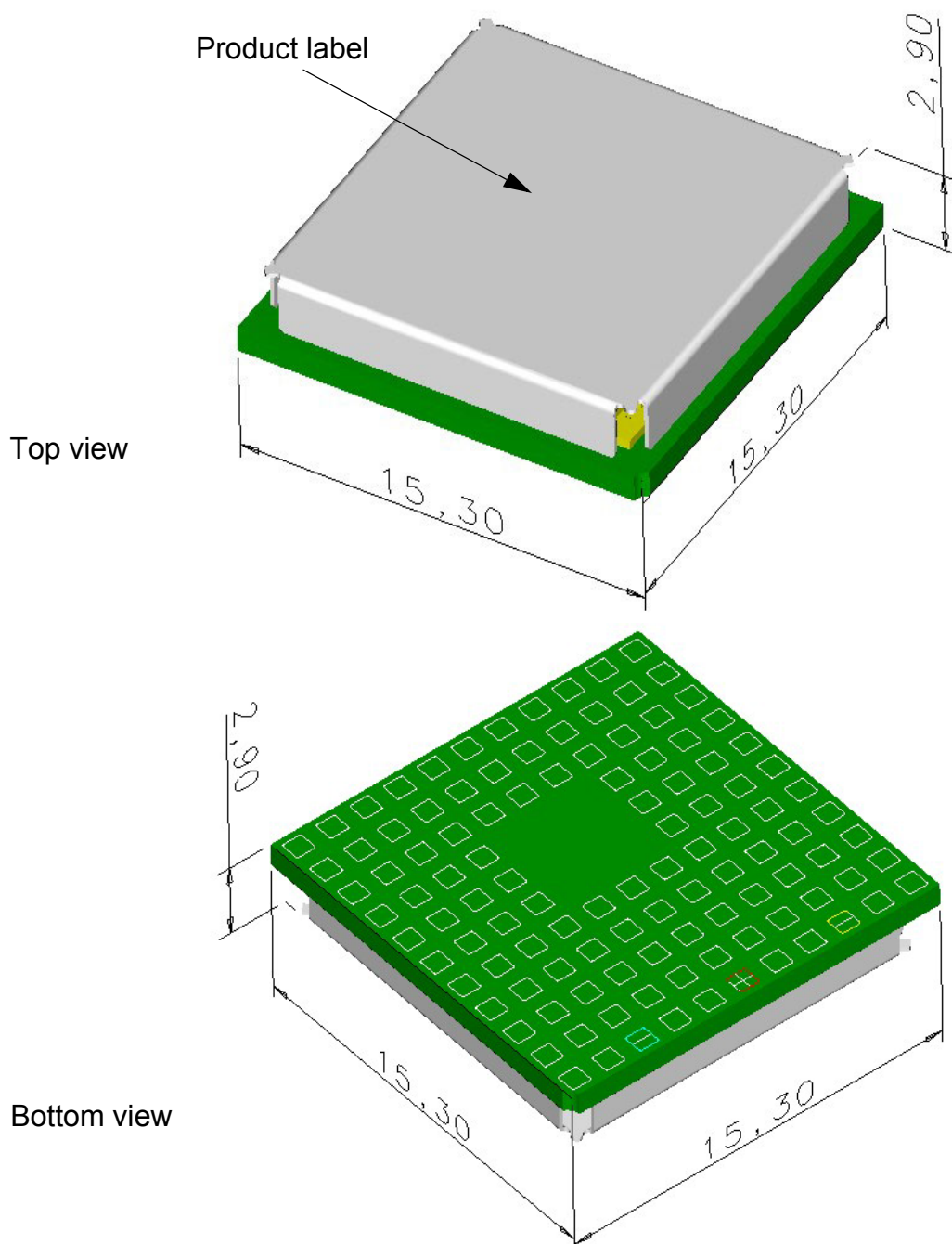
Figure 51: TX62-W– top and bottom view
