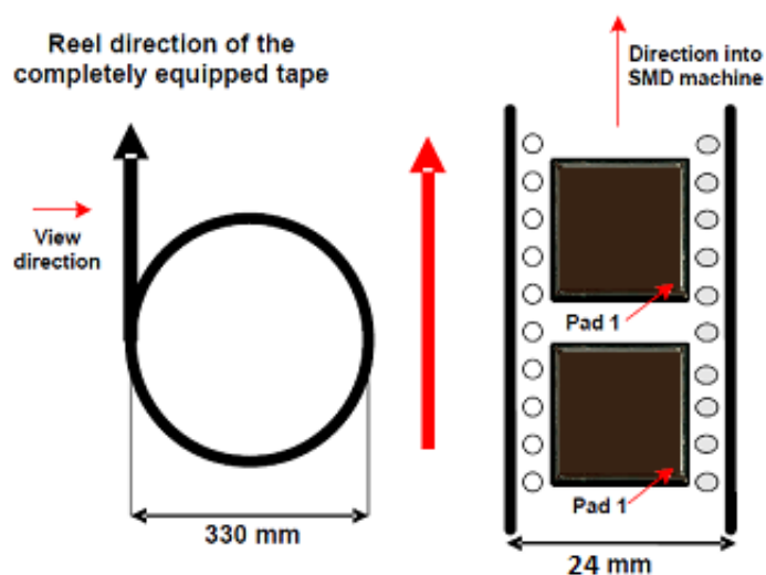
Figure 63: Reel direction
