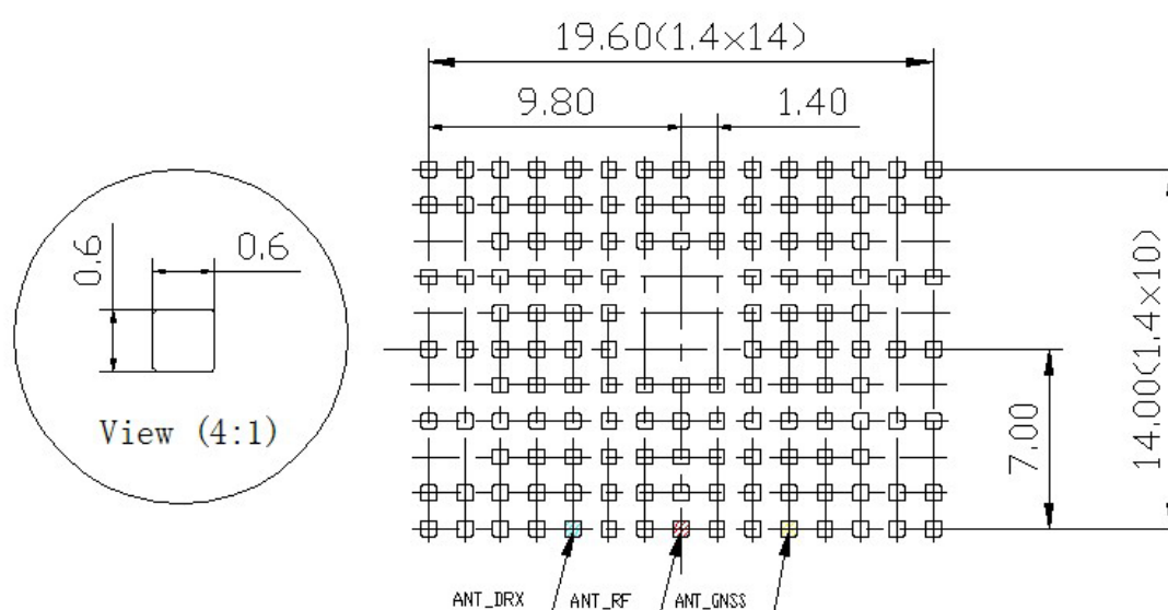
Figure 60: Recommended design for 110µm thick stencil for TX82-W, TX62-W-B and TX62-W-C (top view)
