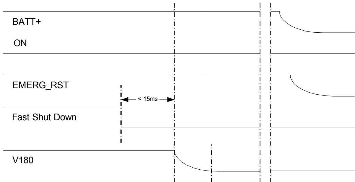
Figure 22: Fast shutdown timing
