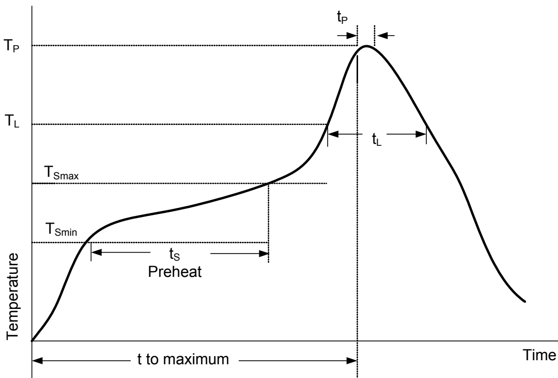
Figure 61: Reflow Profile
