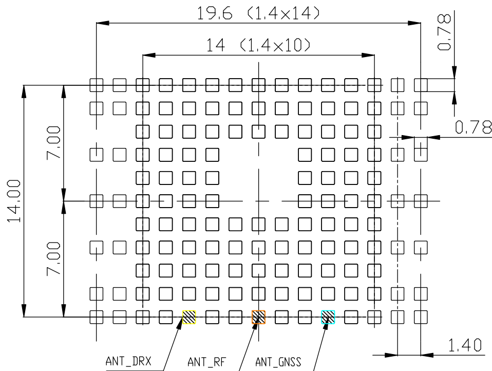
Figure 58: Land pattern TX82-W, TX62-W-B and TX62-W-C (top view)
