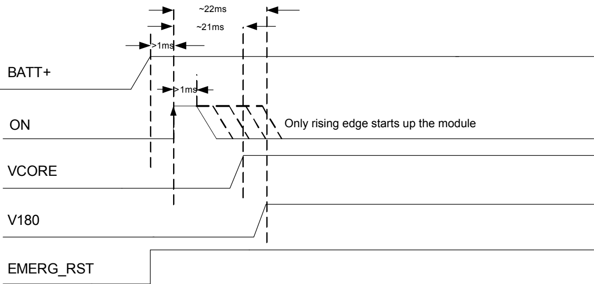
Figure 35: ON startup timing
