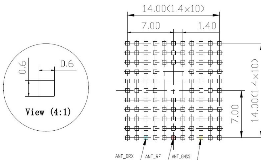
Figure 59: Recommended design for 110µm thick stencil for TX62-W (top view)
