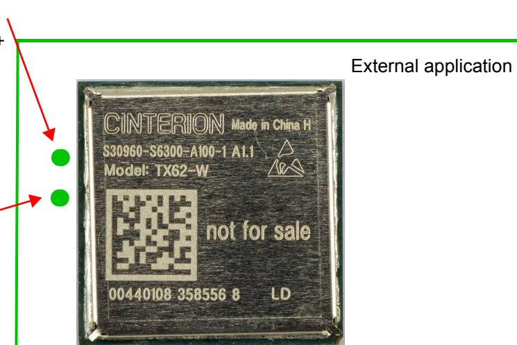
Figure 48: Position of reference points BATT+ and GND
