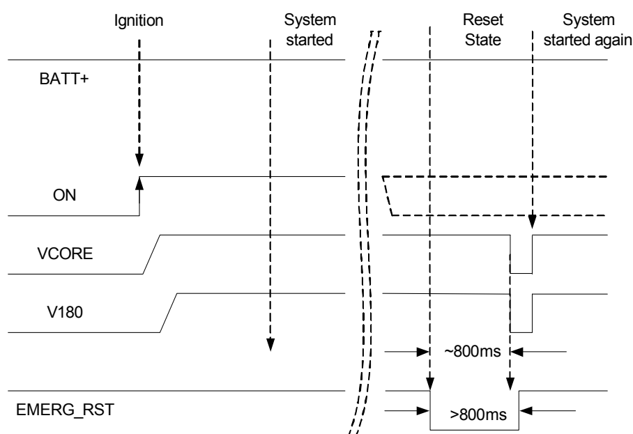
Figure 36: Emergency restart timing
