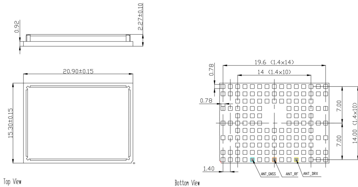
Figure 55: Dimensions of TX82-W, TX62-W-B and TX62-W-C (all dimensions in mm)
