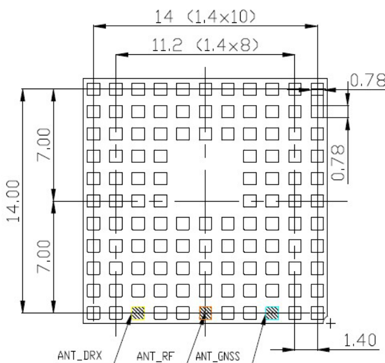
Figure 58: Land pattern TX62-W (top view)
