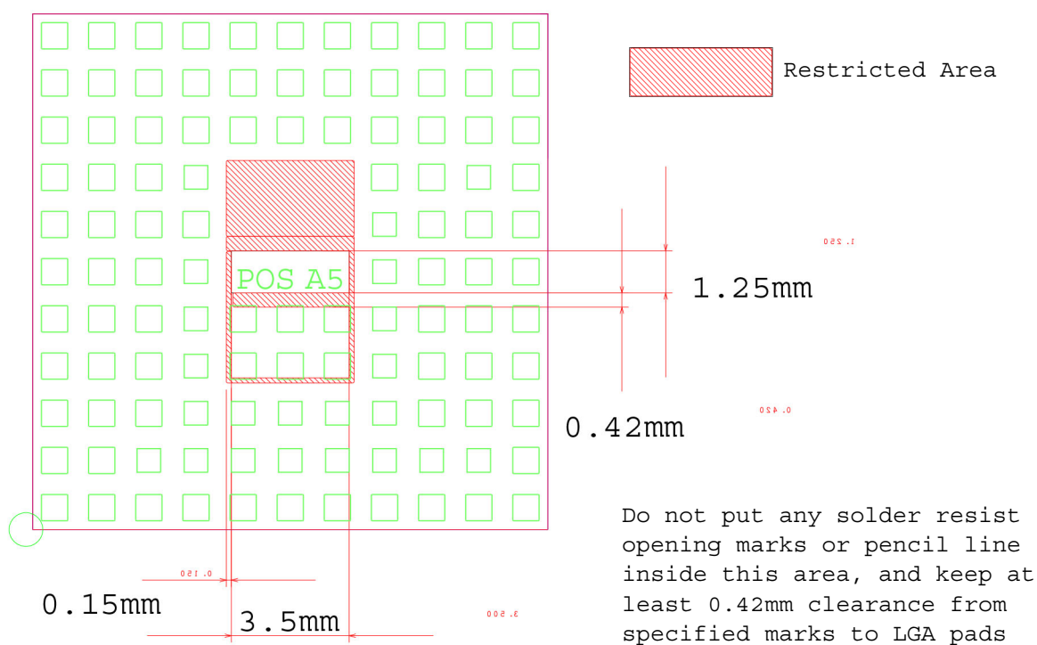
Figure 57: Dimensions of area for possible markings TX82-W, TX62-W-B and TX62-W-C (bottom view)
