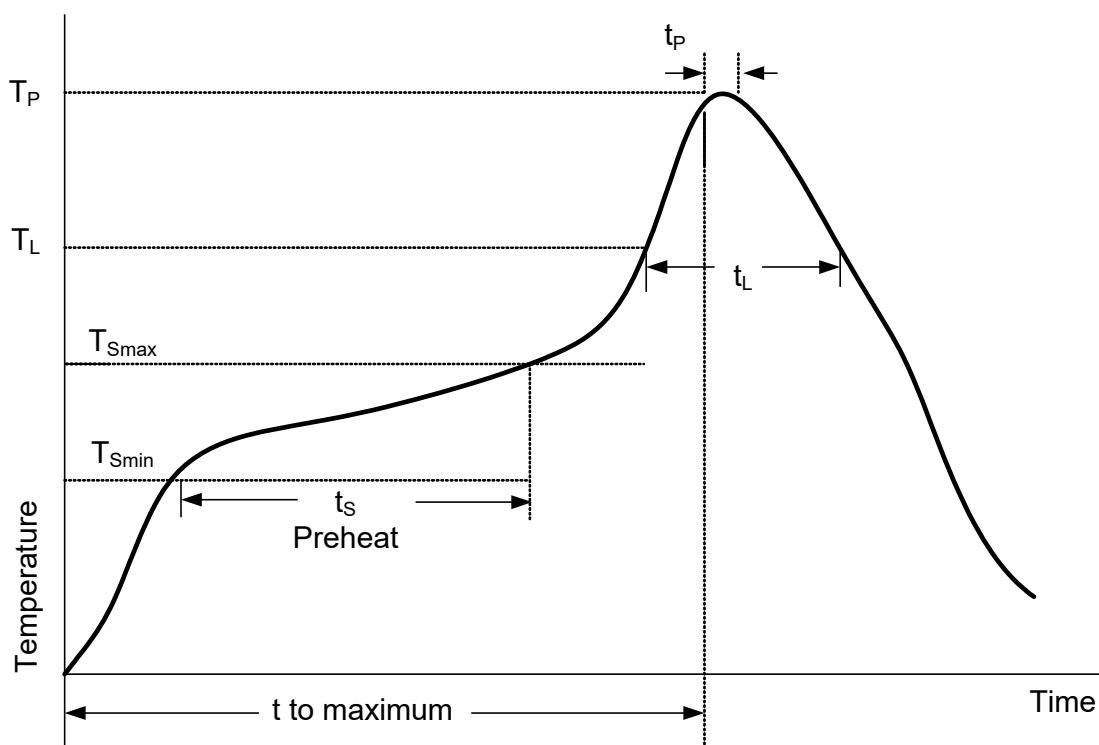
Figure 62: Reflow Profile
