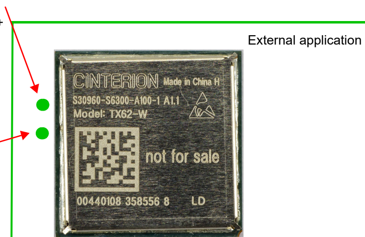
Figure 49: Position of reference points BATT+ and GND
