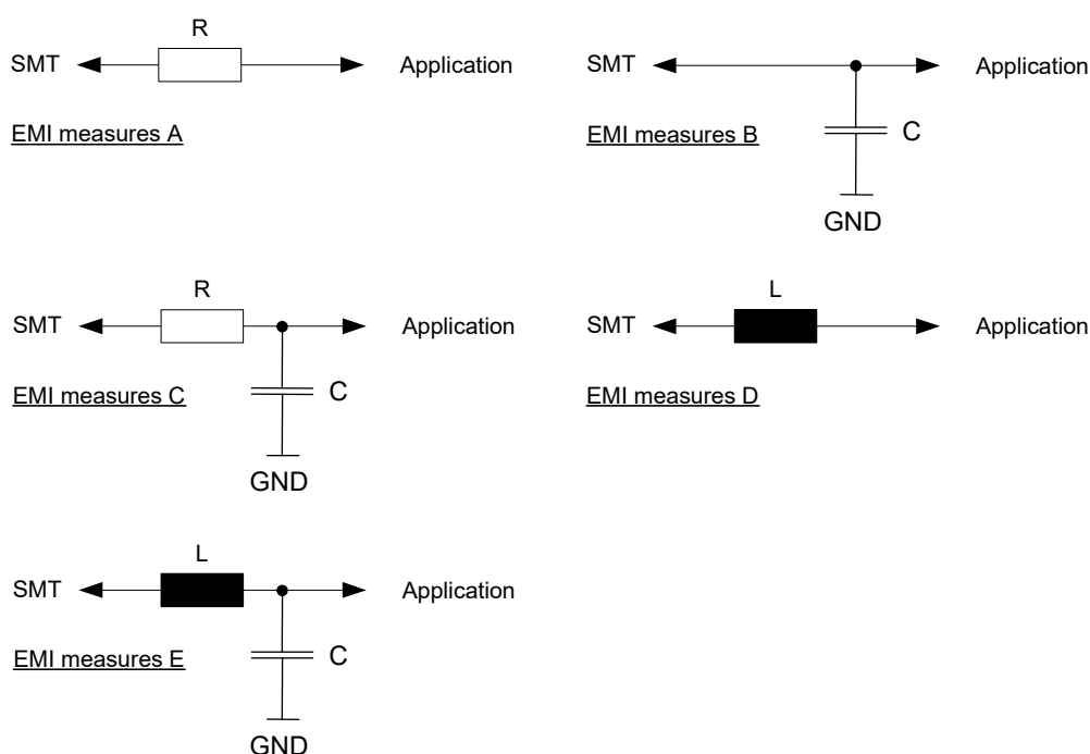
Figure 51: EMI circuits
