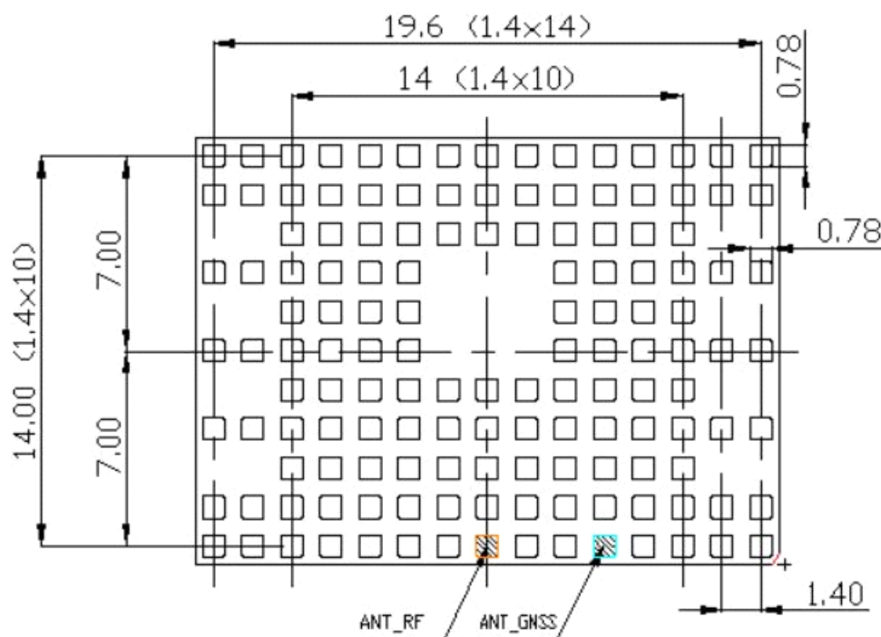
Figure 62: Land pattern TX82-W, TX82-W-B, TX62-W-B and TX62-W-C (top view)
