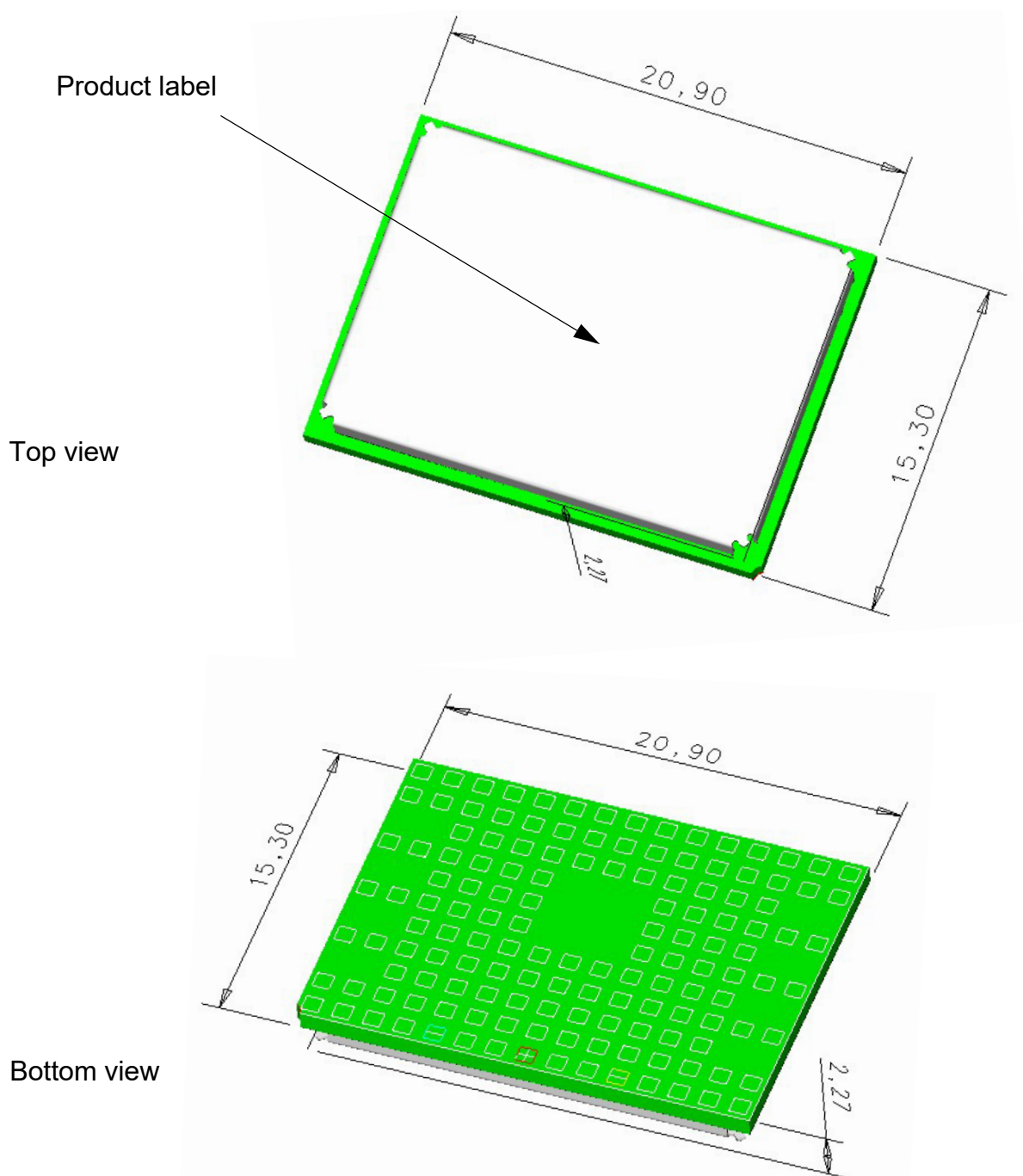
Figure 57: TX82– top and bottom view
