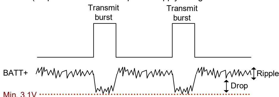
Figure 50: Power supply limits during transmit burst
