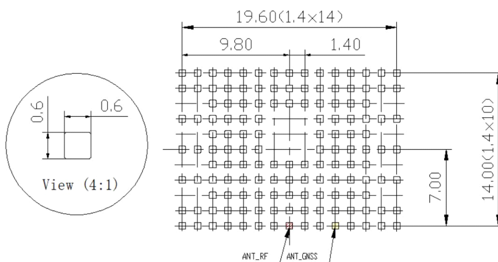
Figure 64: Recommended design for 110µm thick stencil for TX82-W, TX82-W-B, TX62-W-B and TX62-W-C (top view)
