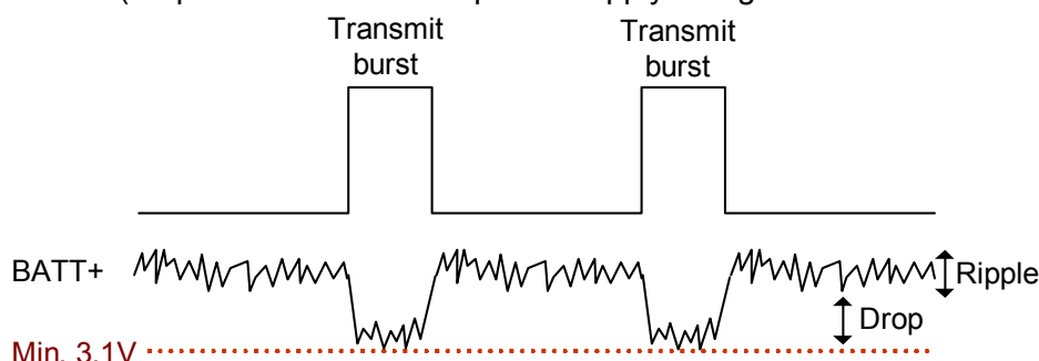
Figure 45: Power supply limits during transmit burst
