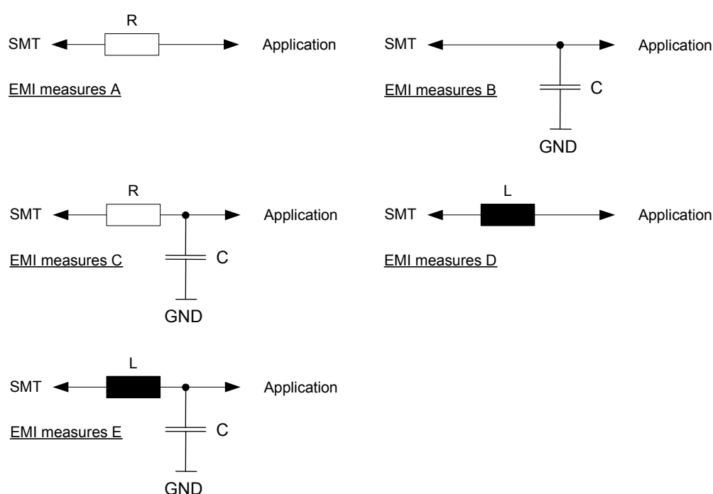
Figure 48: EMI circuits
