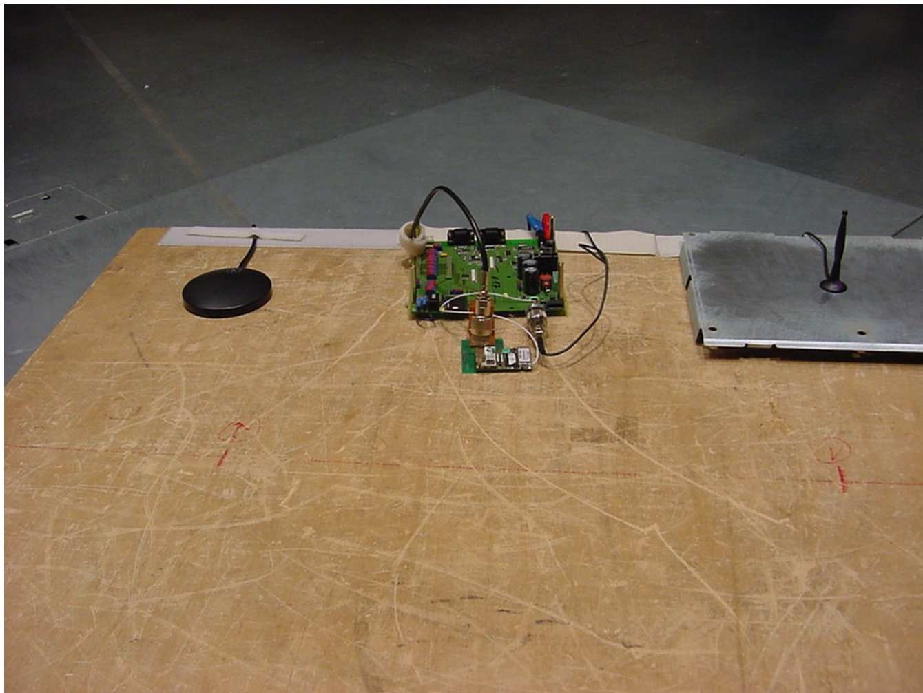
Photo 2 (Radiated Emissions):
