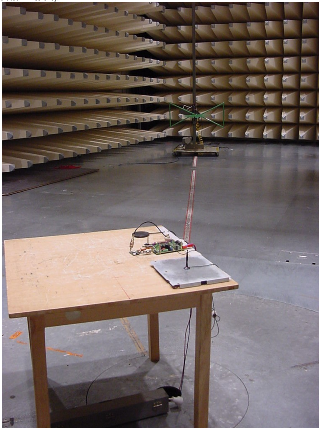
Photo 1 (Radiated Emissions):
