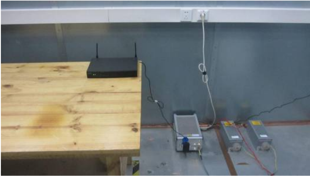
Picture 2 Conducted Emission Test Setup
