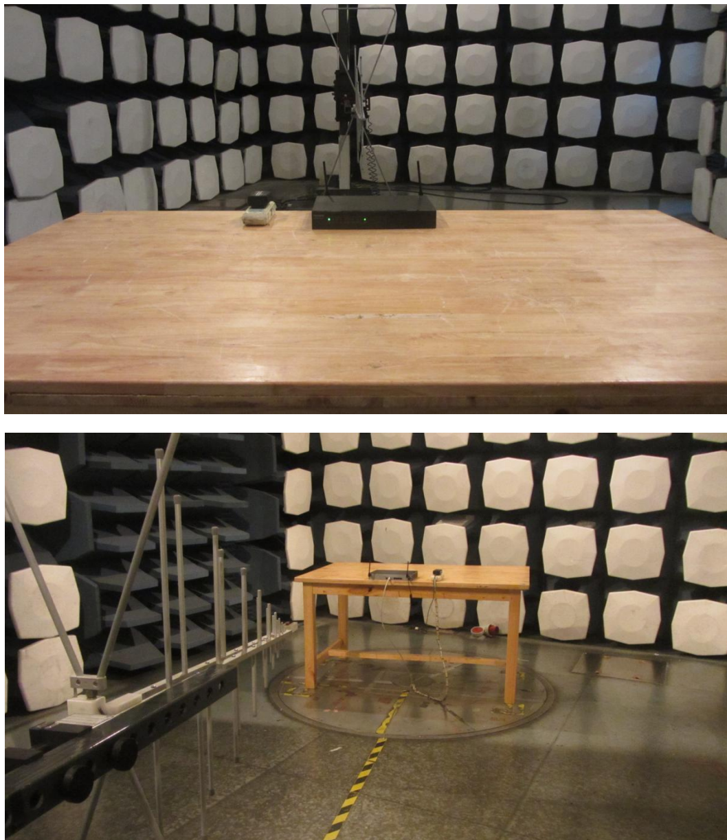
Picture 1 Radiated Emission Test Setup
