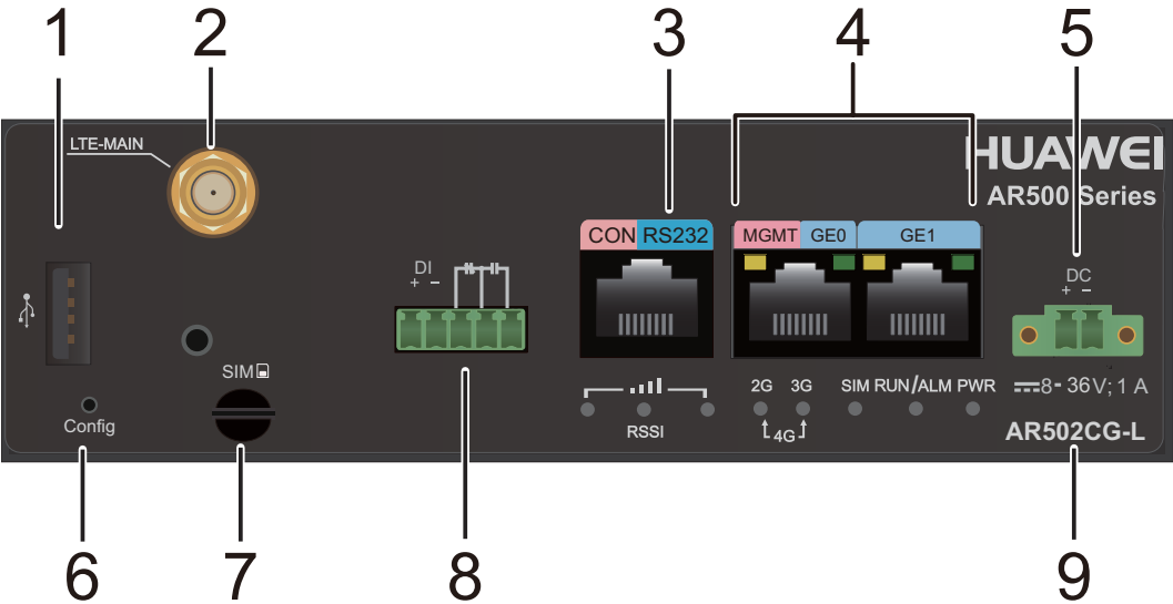
Figure 4-3 AR502CG-L appearance Removing the SIM card cover:
