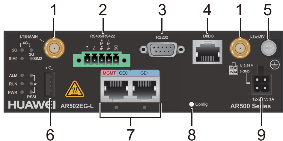
Figure 4-1 AR502EG-L appearance
