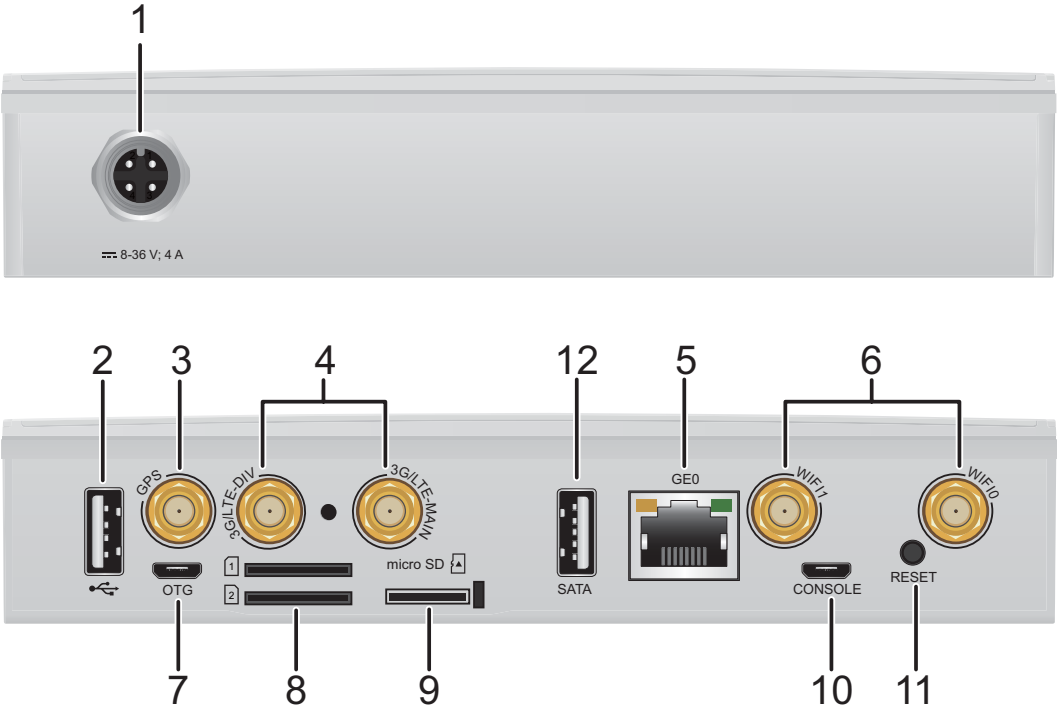
Figure 4-15 AR511GW-LM7 appearance
