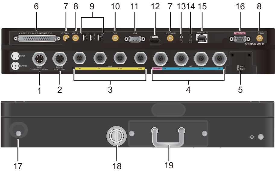
Figure 4-18 AR515GW-LM9-D appearance
