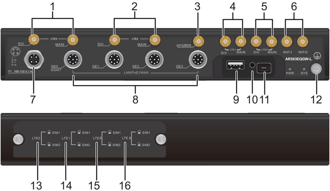
Figure 4-11 AR503EQGW-L appearance
