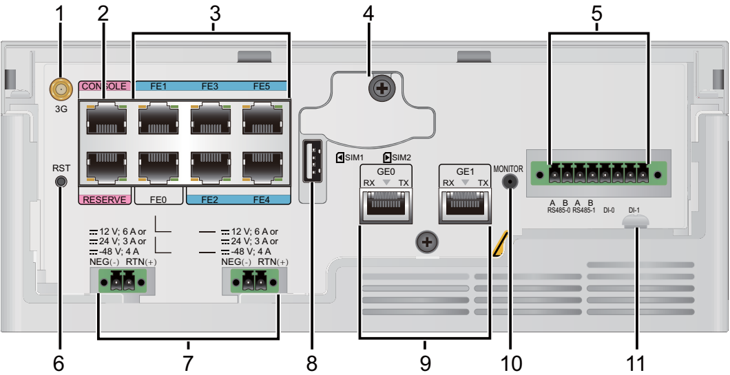
Figure 4-22 AR531G-U-D-H panel
