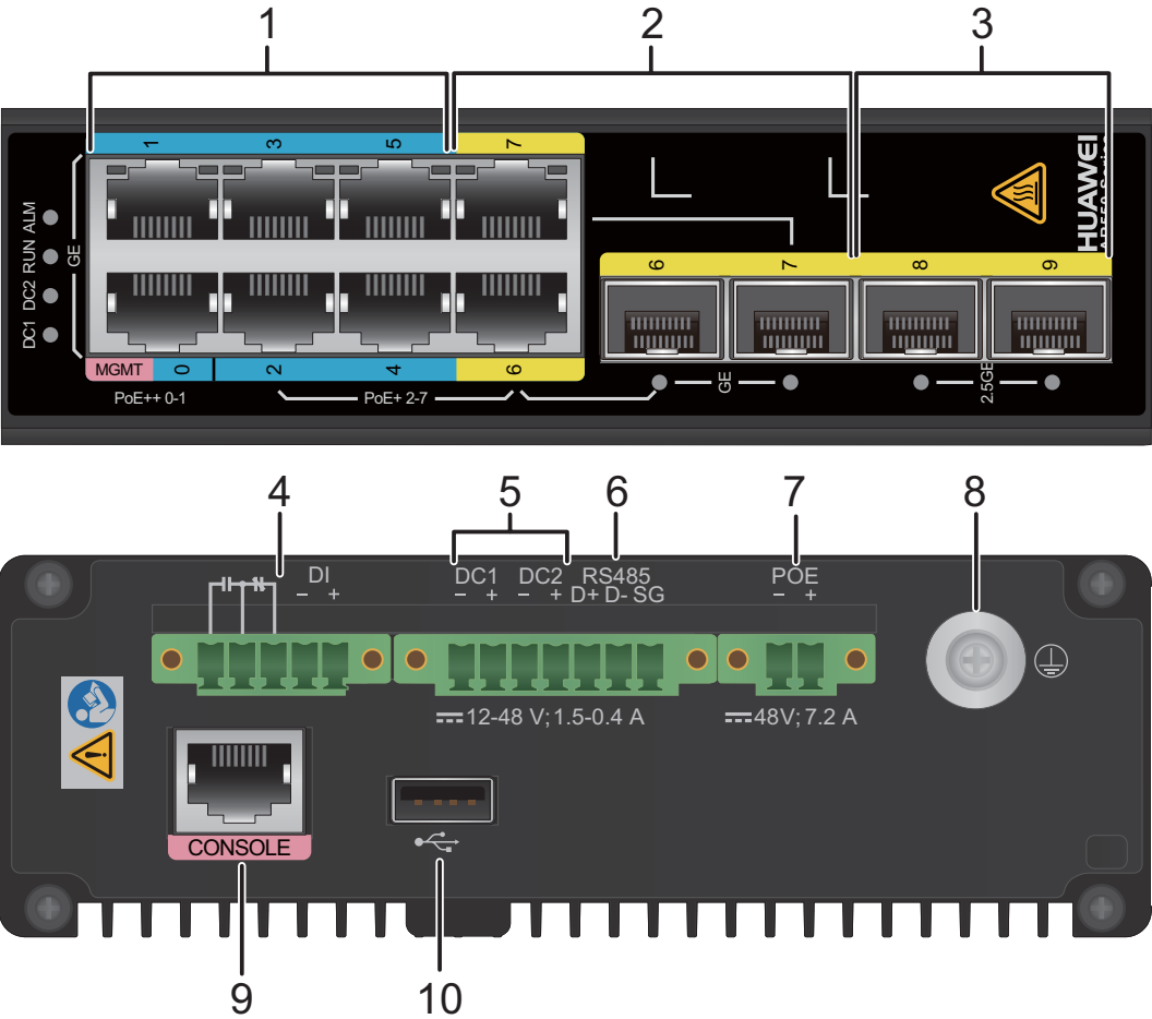
Figure 4-24 AR550C-2C6GE appearance
