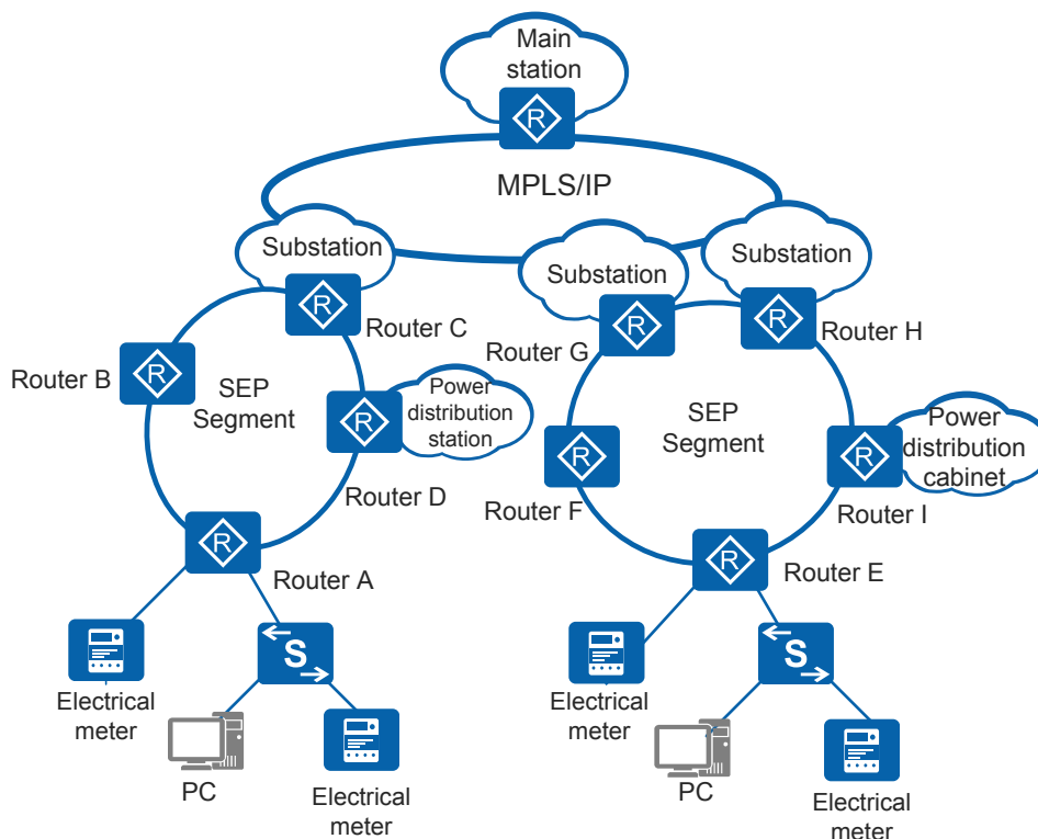
Figure 2-4 AR2500s used as industrial switches to implement fast switching of data channels
