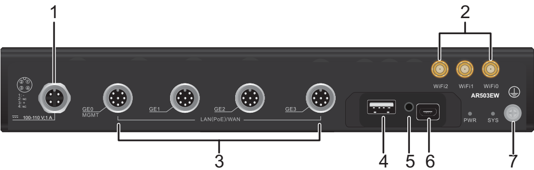
Figure 4-12 AR503EW appearance
