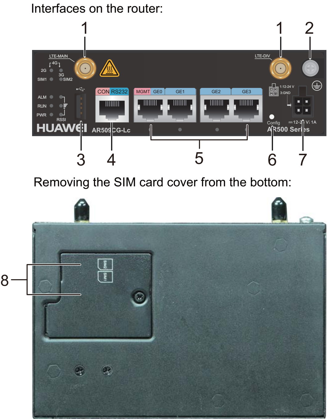
Figure 4-9 AR509CG-Lc appearance
