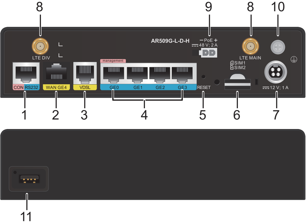
Figure 4-7 AR509G-L-D-H appearance
