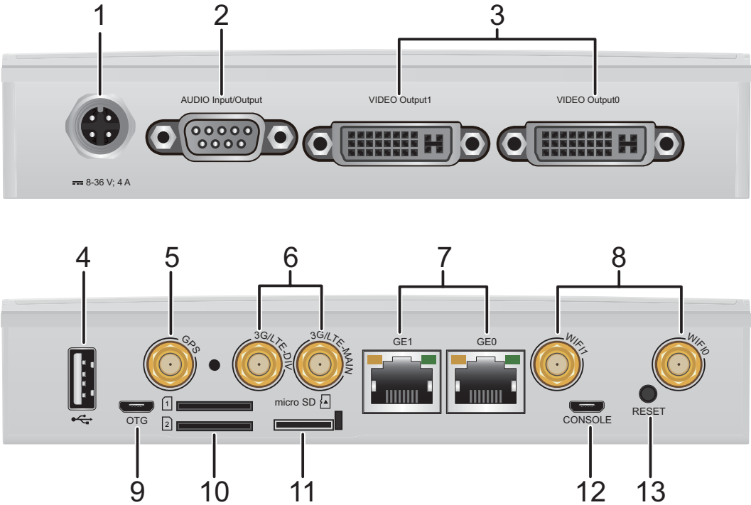
Figure 4-13 AR511GW-LAV2M3 appearance
