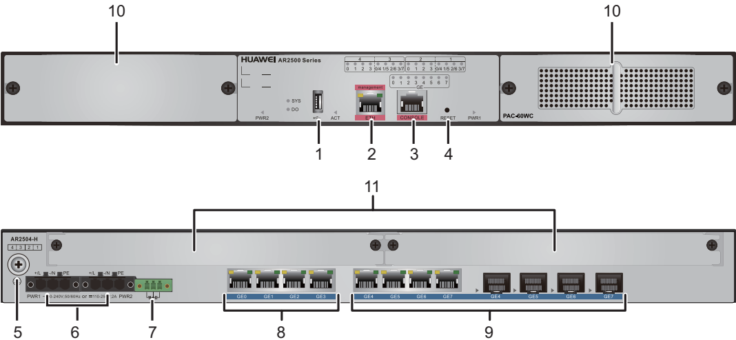
Figure 4-25 AR2504-H panels
