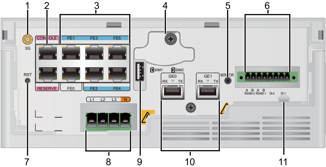
Figure 4-21 AR531GPe-U-H panel
