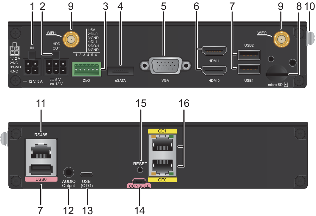
Figure 4-17 AR513W-V3M8 appearance
