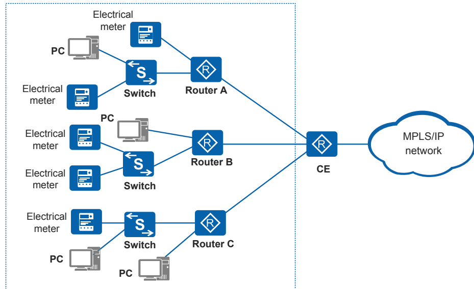
Figure 2-3 AR2500 used as industrial switches to connect to terminals and access switches
