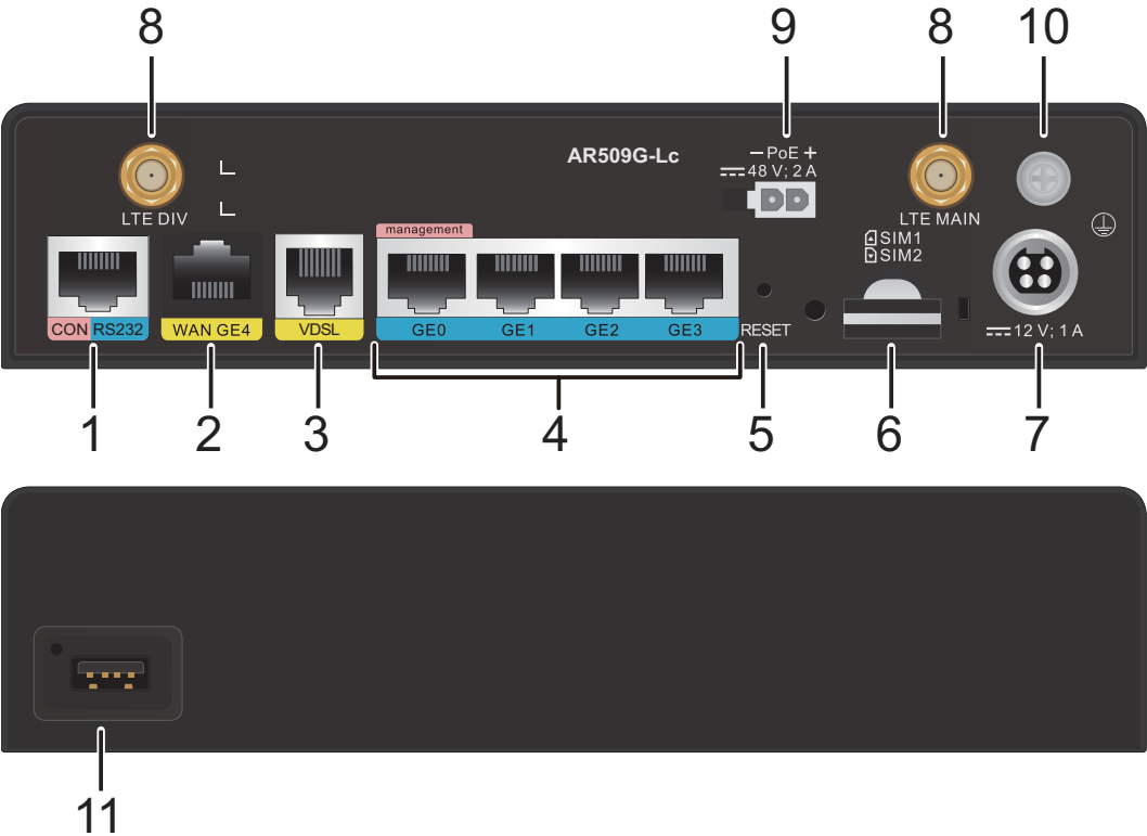
Figure 4-8 AR509G-Lc appearance
