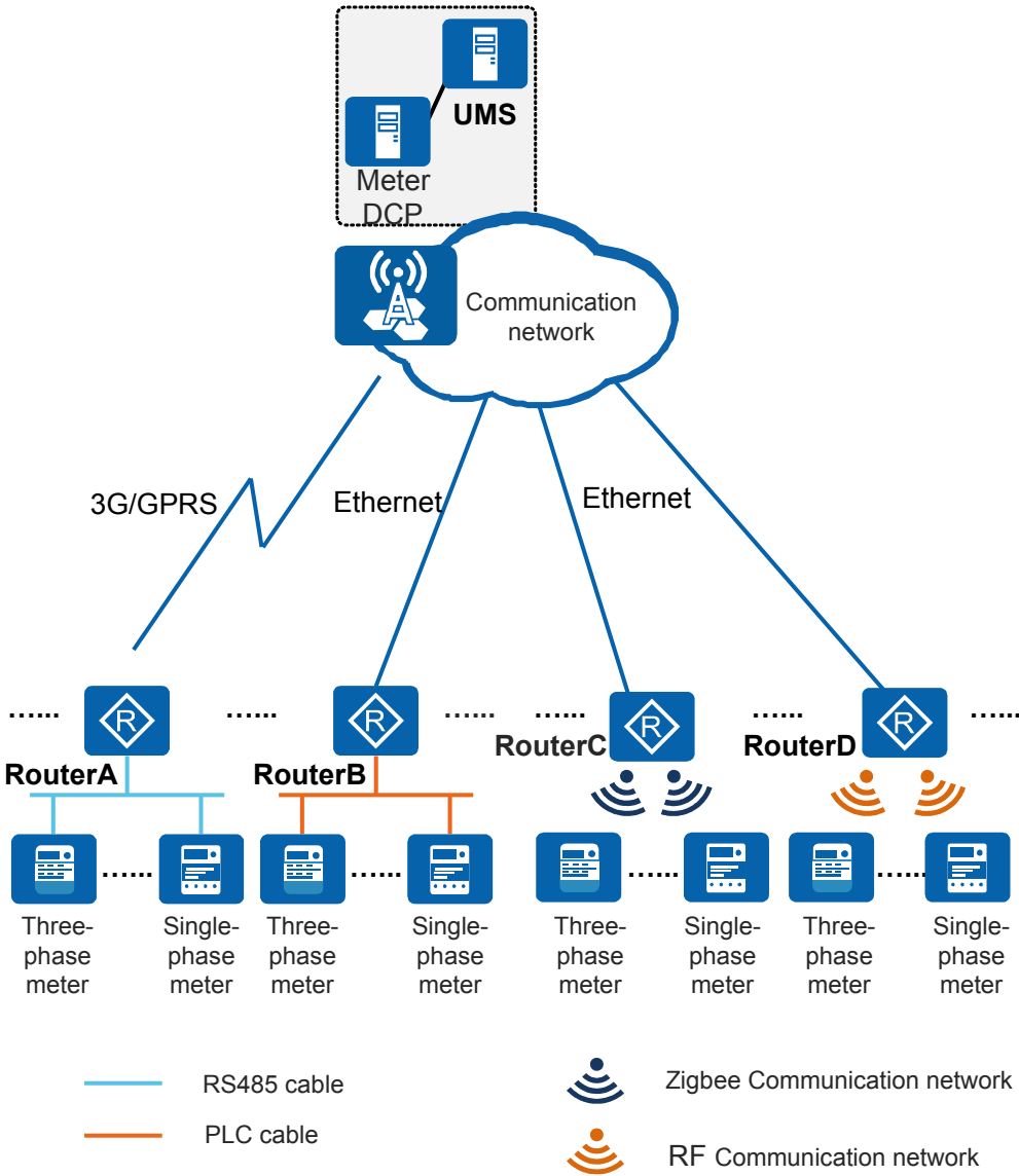
Figure 2-5 AR500&AR530 used as industrial gateways
