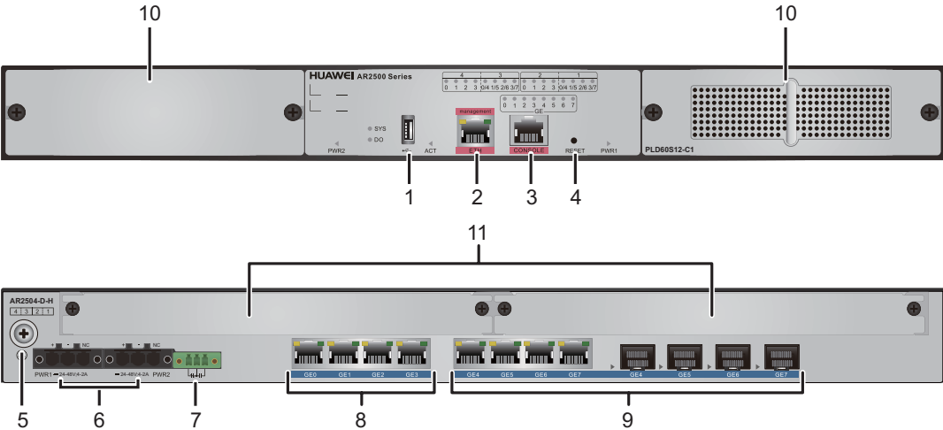
Figure 4-27 AR2504-D-H appearance
