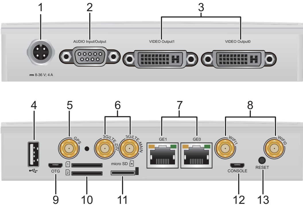
Figure 4-14 AR511CGW-LAV2M3 appearance
