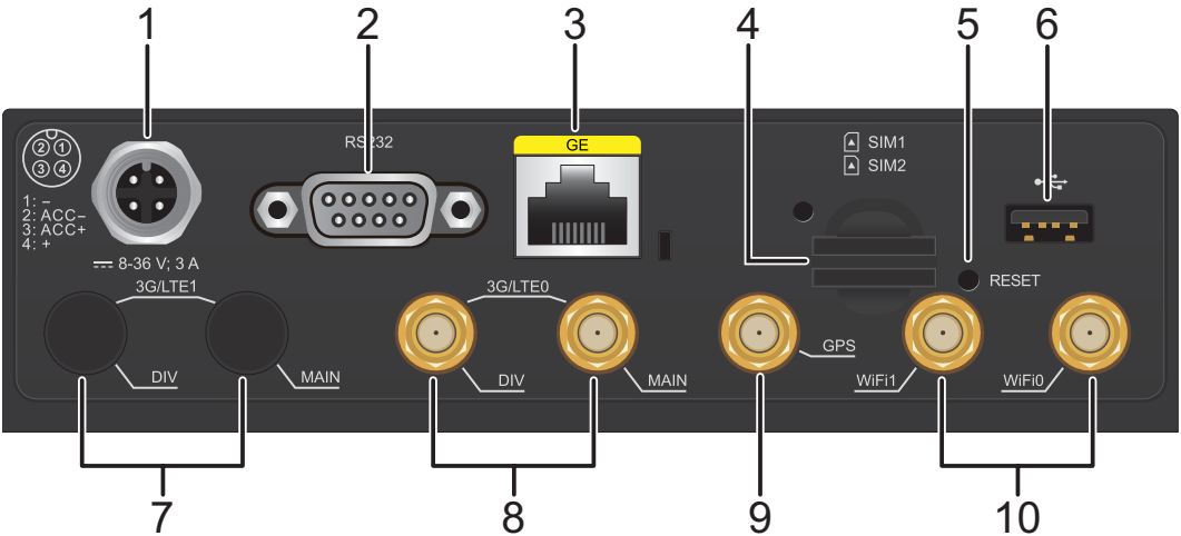
Figure 4-4 AR503GW-LM7 appearance
