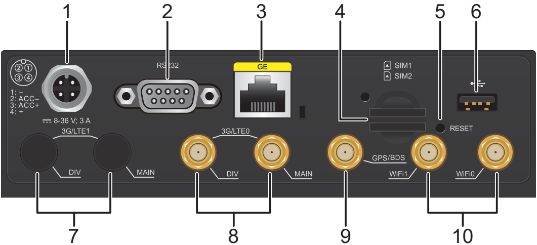
Figure 4-5 AR503GW-LcM7 appearance
