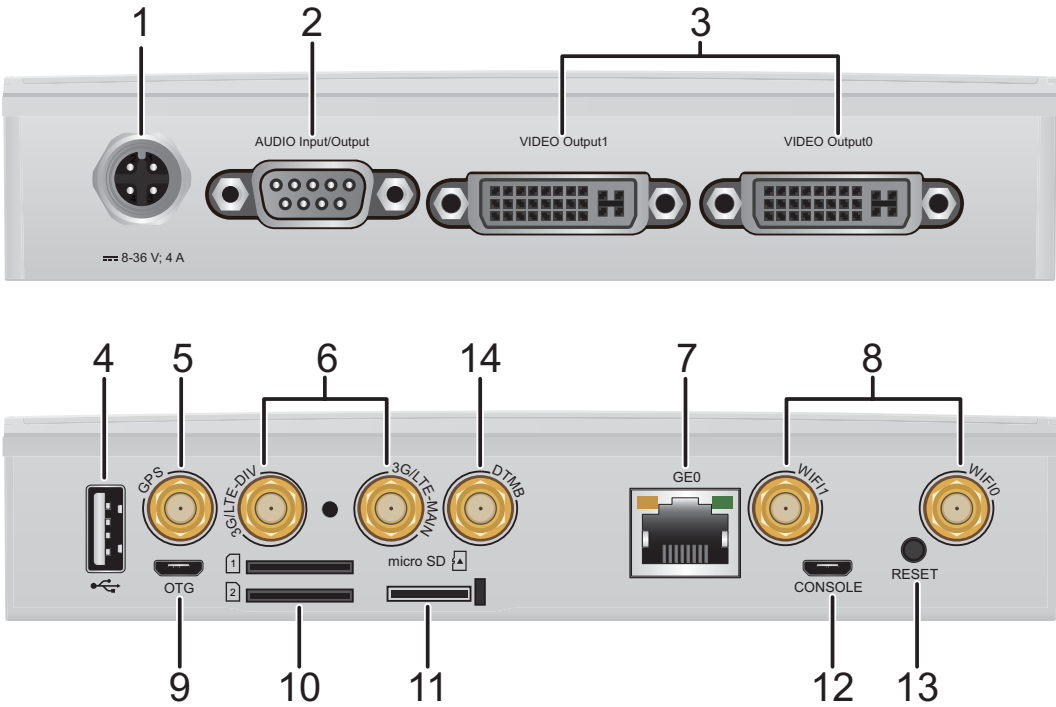
Figure 4-16 AR511GW-L-B3 appearance
