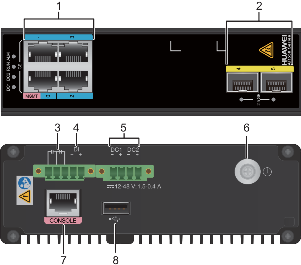
Figure 4-23 AR550C-4GE appearance
