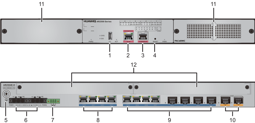
Figure 4-26 AR2504E-H panels
