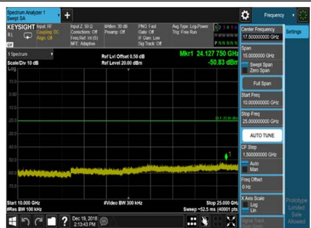
DQPSK,2480MHz,2DH5,Plot 4,10000MHz~25000MHz
