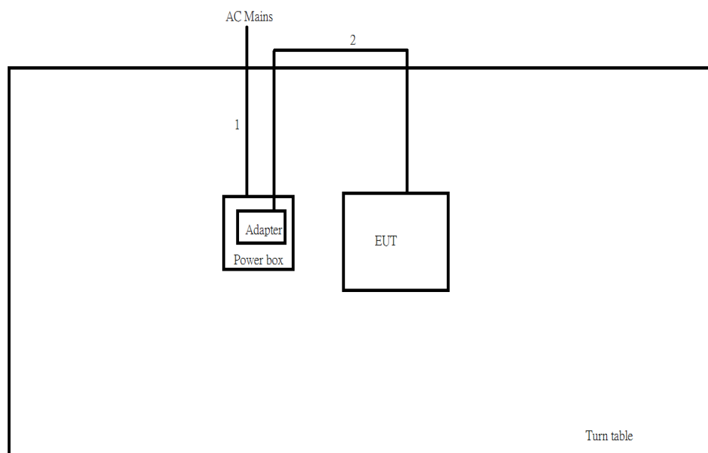
Test Setup Diagram - Radiated Test
