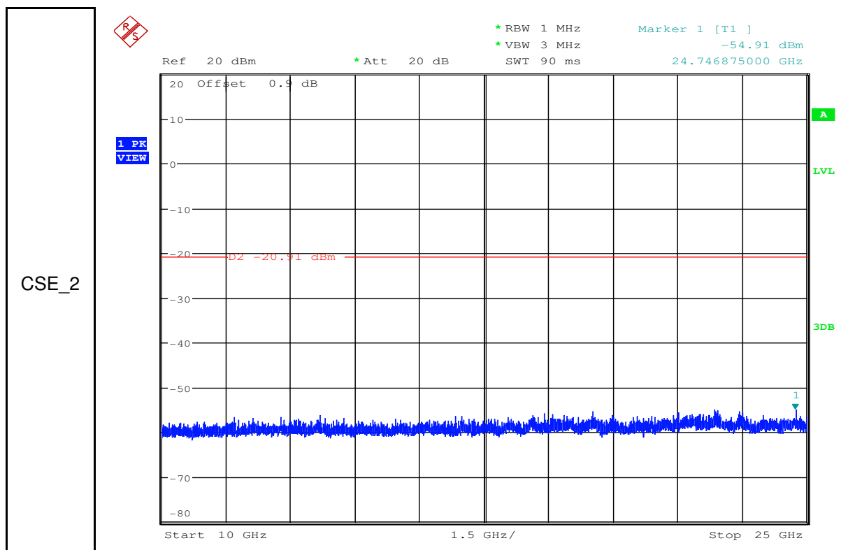
RF Conducted Spurious Emissions 11N20SISO 2412 Ant2
