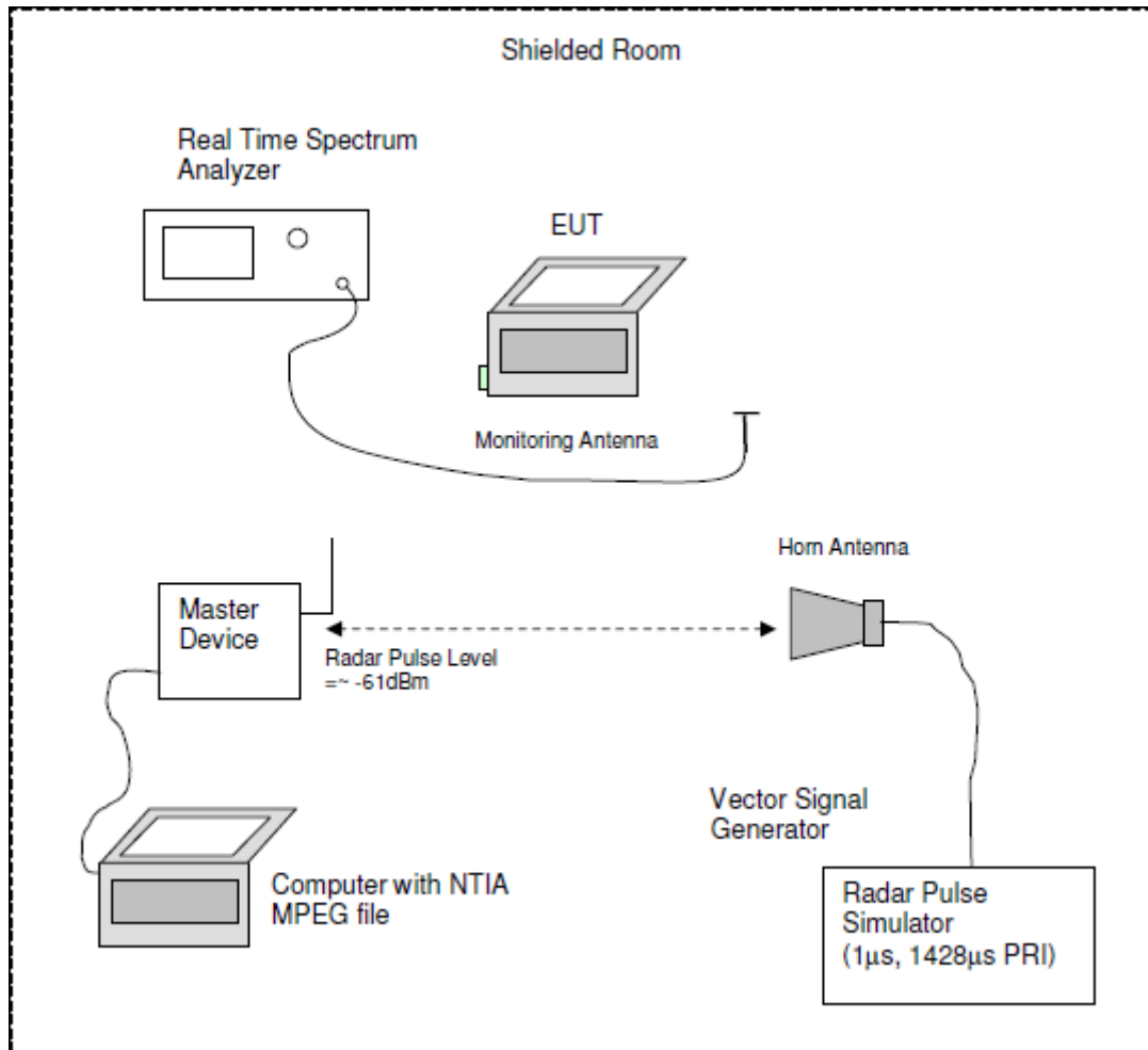
Figure 3-1. Radiated Test Setup for DFS
