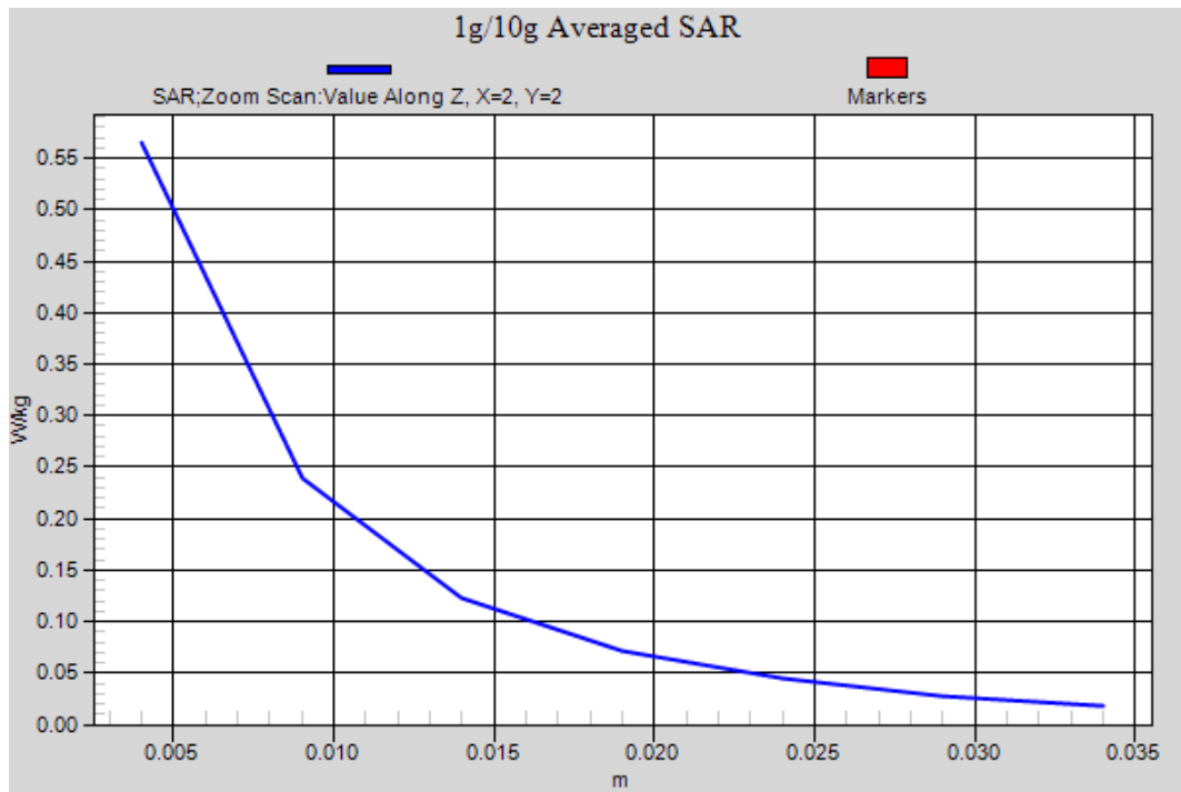
Figure 16 GSM 850 GPRS (2TXslots) with Test Position 1 Channel 190
