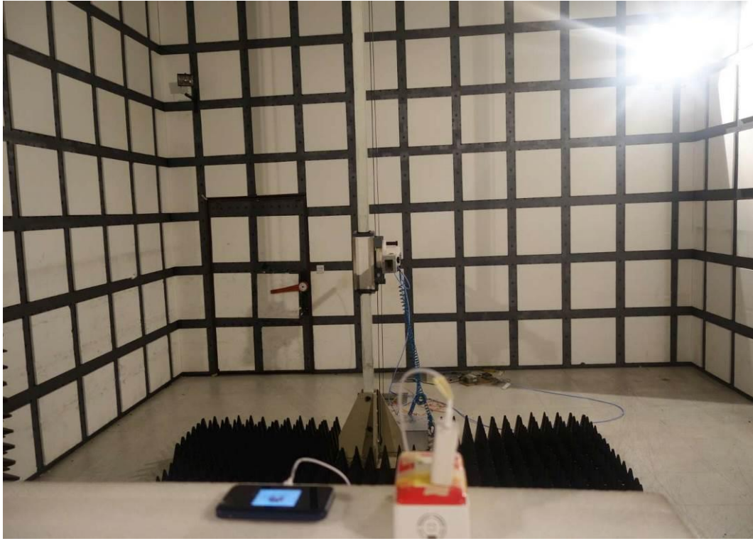
Radiated Disturbance (18GHz-40GHz)
