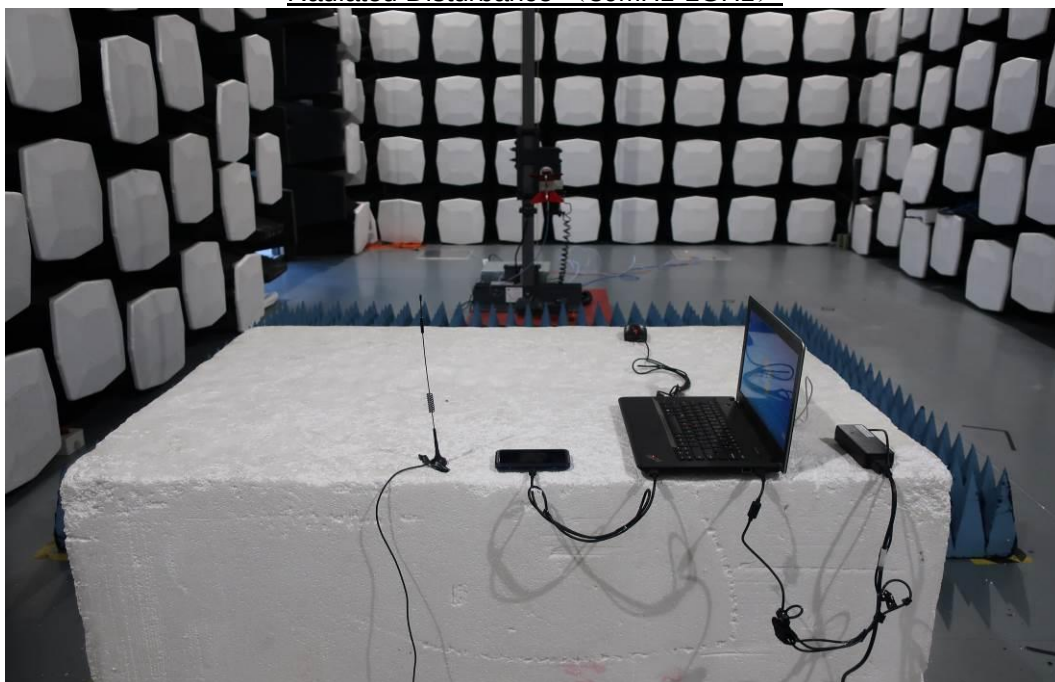
Radiated Disturbance (1GHz-18GHz)
