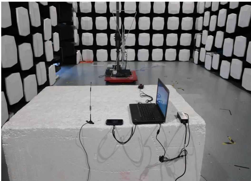
Radiated Disturbance (30MHz-1GHz)
