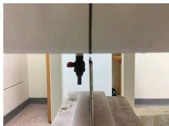
Fig.8 EUT Top side (11mm) to flat phantom
