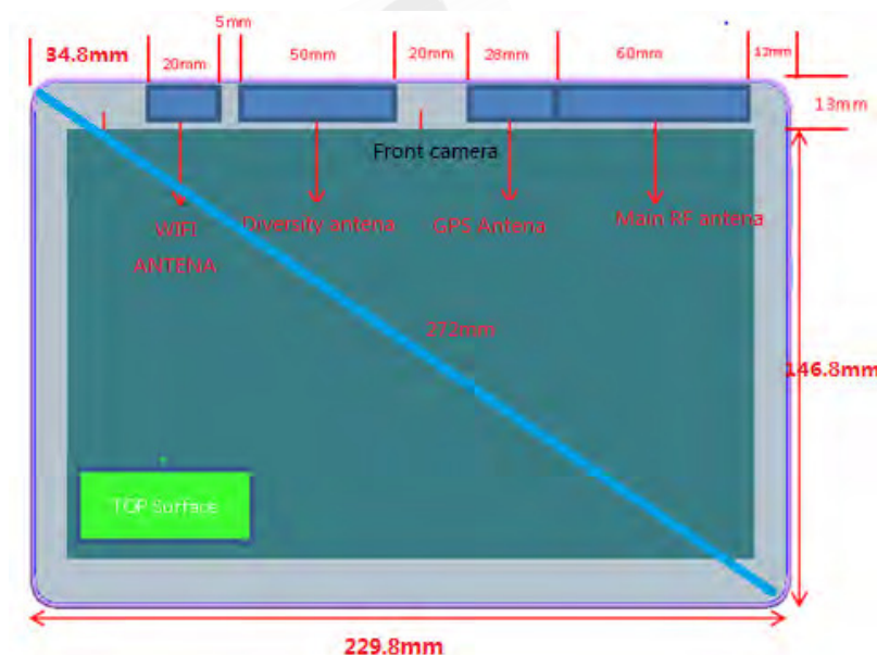
Fig.13 Antenna position of EUT (Front view)
