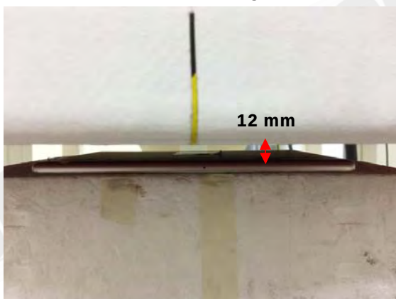
Fig.5 EUT Back side (12mm) to flat phantom
