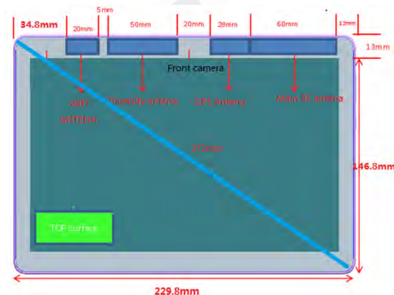
Fig.10 Antenna position of EUT (Front view)
