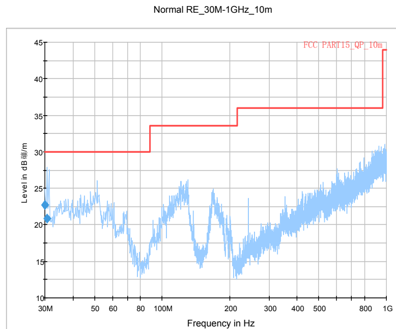
Fig. 25 Radiated Spurious Emission (GFSK, Ch0, 30 MHz ~1 GHz,AE4)
