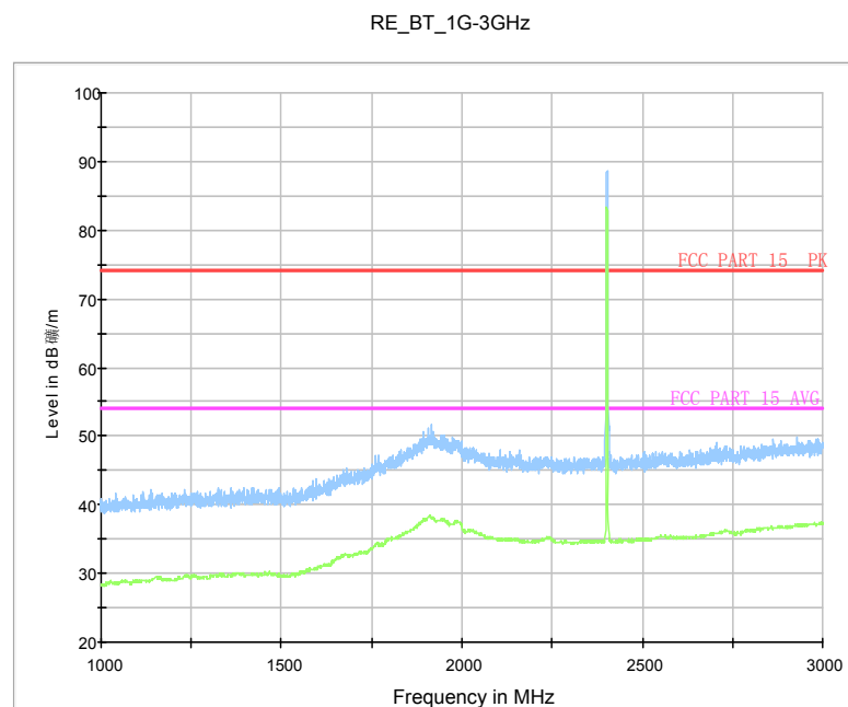
Fig.28 Radiated Spurious Emission (Ch0, 1 GHz-3 GHz)
