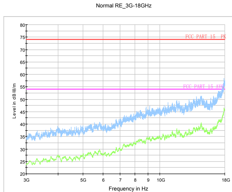
Fig.29 Radiated Spurious Emission (Ch0, 3 GHz-18 GHz)
