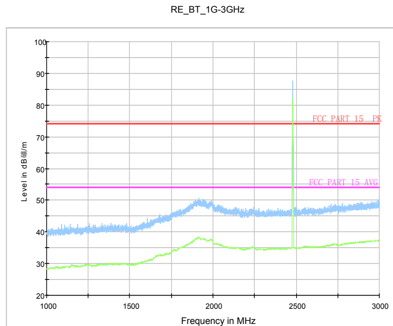
Fig.32 Radiated Spurious Emission (Ch39, 1 GHz-3 GHz)
