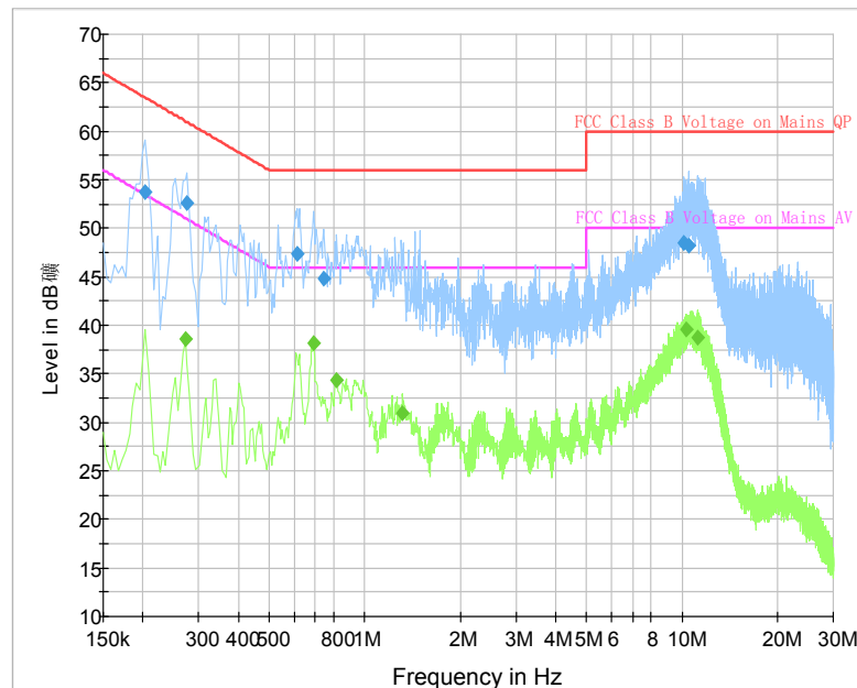
Fig. 38 AC Power line Conducted Emission (Traffic, AE2)
