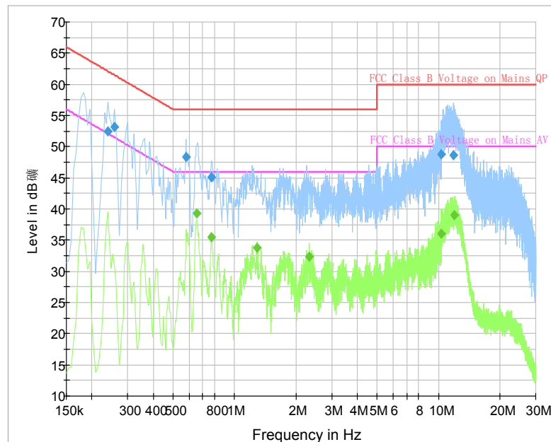
Fig. 41 AC Power line Conducted Emission (Traffic, AE5)
