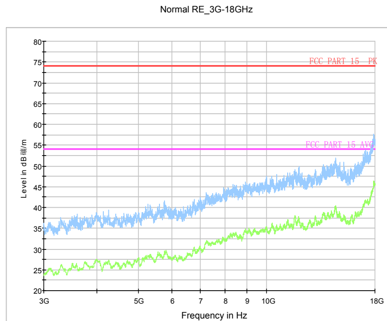
Fig.33 Radiated Spurious Emission (Ch39, 3 GHz-18 GHz)
