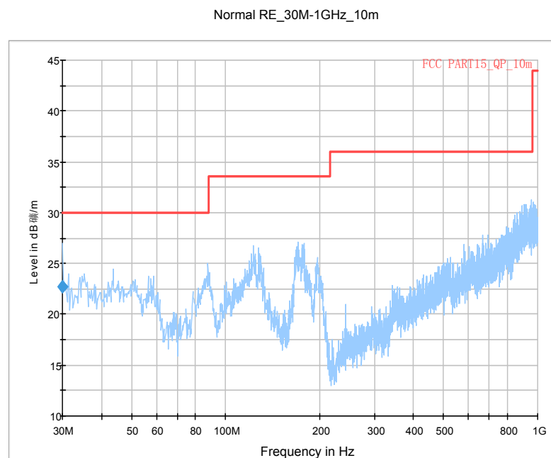
Fig. 24 Radiated Spurious Emission (GFSK, Ch0, 30 MHz ~1 GHz,AE3)
