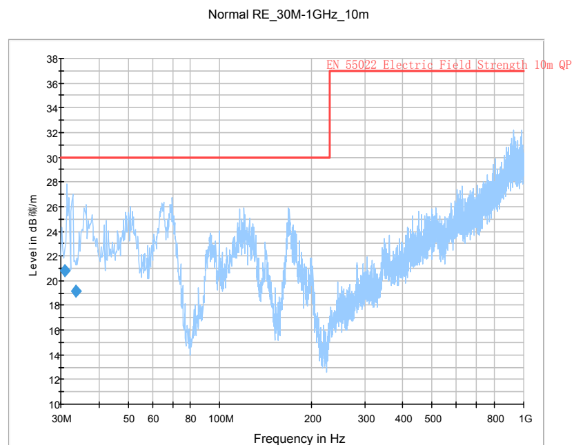
Fig. 26 Radiated Spurious Emission (GFSK, Ch0, 30 MHz ~1 GHz,AE5)
