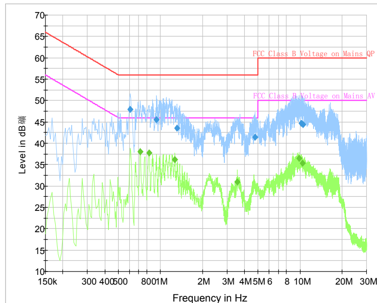
Fig. 42 AC Power line Conducted Emission (Traffic, AE6)
