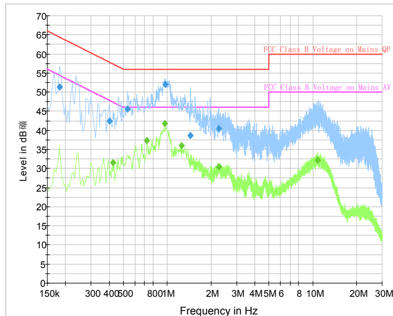
Fig. 37 AC Power line Conducted Emission (Traffic, AE1)
