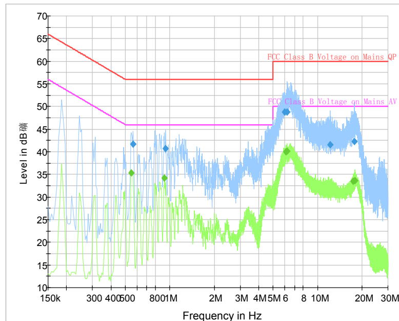
Fig. 40 AC Power line Conducted Emission (Traffic, AE4)
