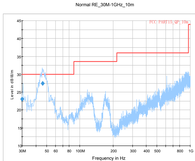
Fig. 27 Radiated Spurious Emission (GFSK, Ch0, 30 MHz ~1 GHz,AE6)
