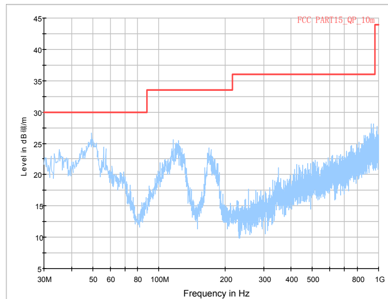
Fig. 22 Radiated Spurious Emission (GFSK, Ch0, 30 MHz ~1 GHz,AE1)
