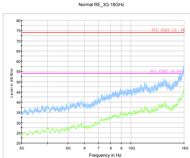
Fig.31 Radiated Spurious Emission (Ch19, 3 GHz-18 GHz)
