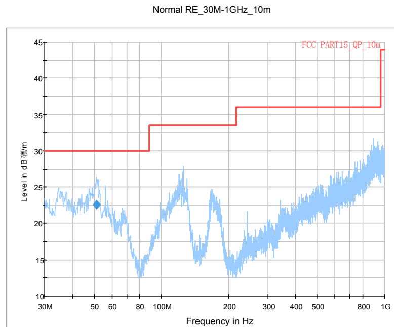
Fig. 23 Radiated Spurious Emission (GFSK, Ch0, 30 MHz ~1 GHz,AE2)
