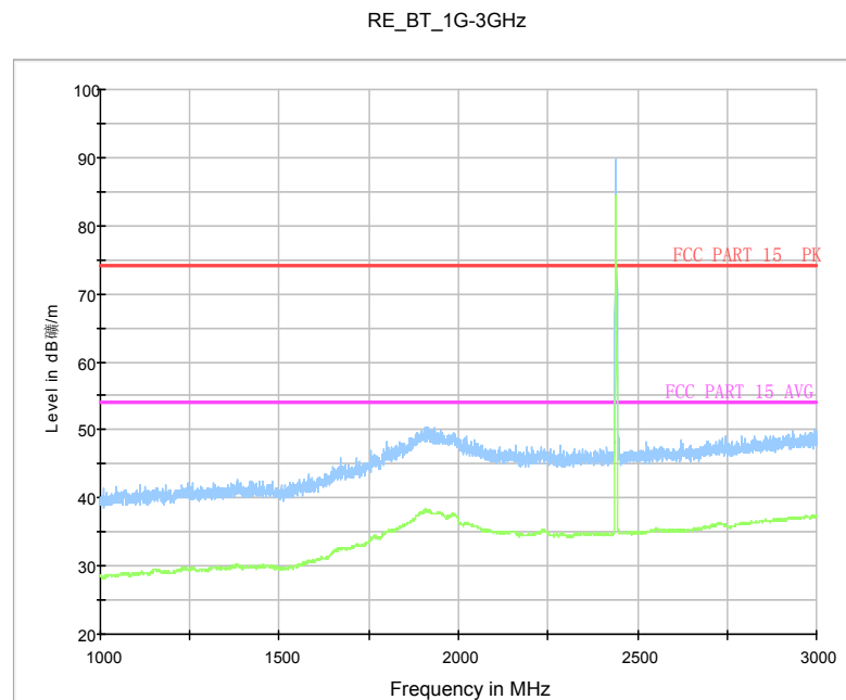
Fig.30 Radiated Spurious Emission (Ch19, 1 GHz-3 GHz)
