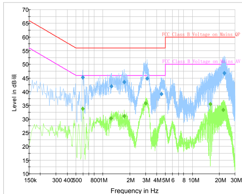
Fig. 39 AC Power line Conducted Emission (Traffic, AE3)
