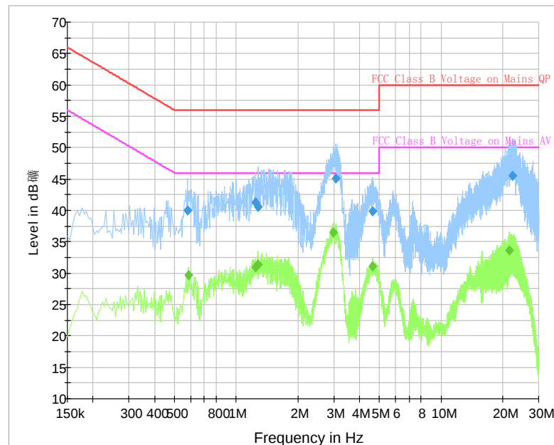
Fig. 110 AC Power line Conducted Emission (Traffic, AE4)
