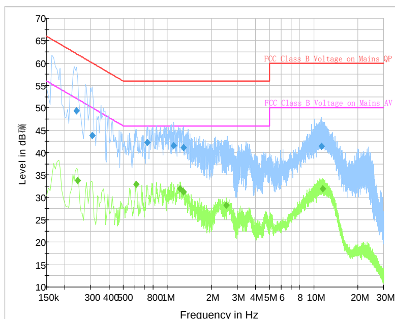
Fig. 107 AC Power line Conducted Emission (Traffic, AE1)
