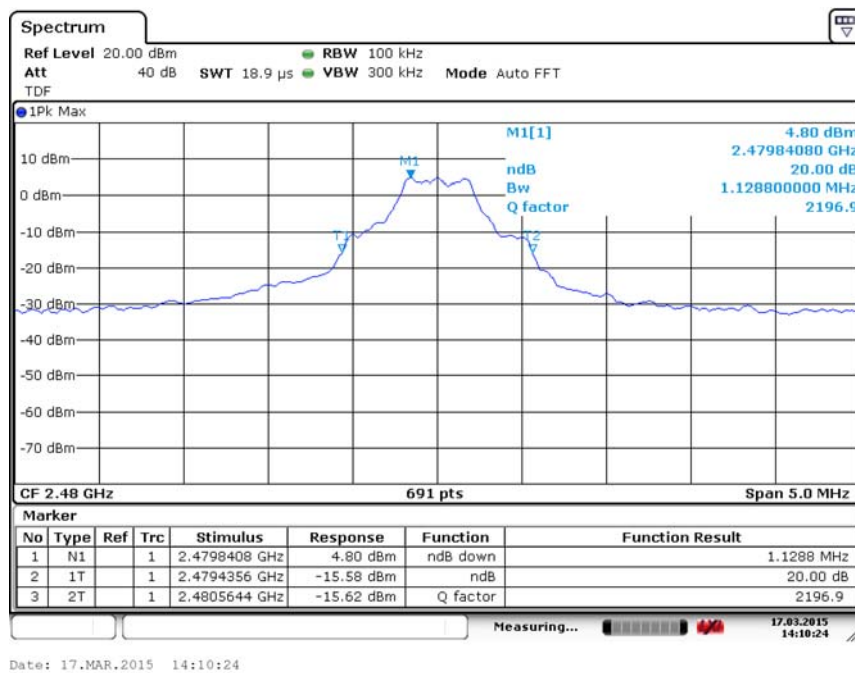
Fig. 85 Occupied 20dB Bandwidth (GFSK, Ch 78)
