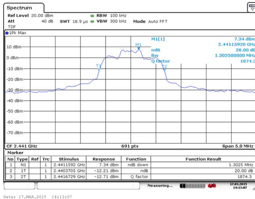
Fig. 90 Occupied 20dB Bandwidth (8DPSK, Ch 39)
