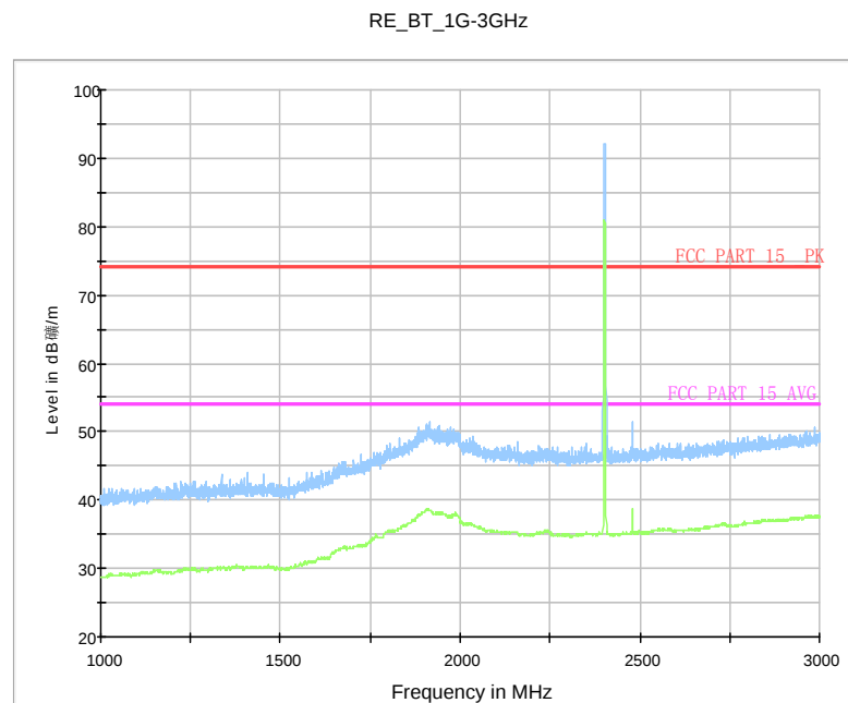
Fig. 64 Radiated Spurious Emission ( \pi/4 DQPSK, Ch0, 1 GHz ~3 GHz)
