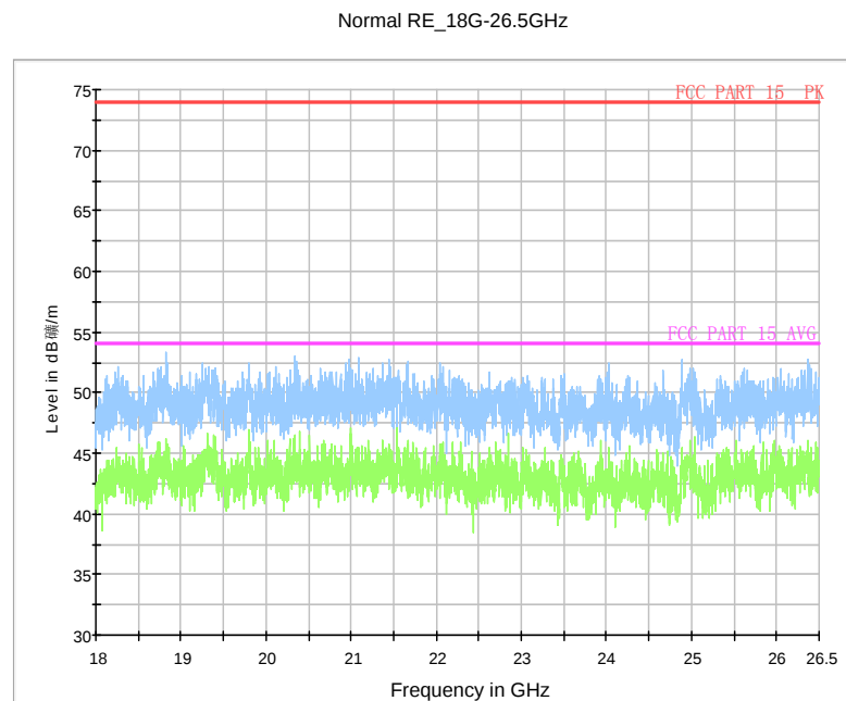
Fig. 82 Radiated Spurious Emission (All channel, 18 GHz ~26.5 GHz)
