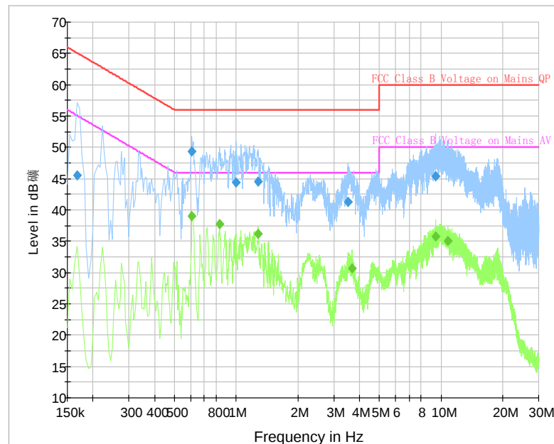
Fig. 112 AC Power line Conducted Emission (Traffic, AE6)
