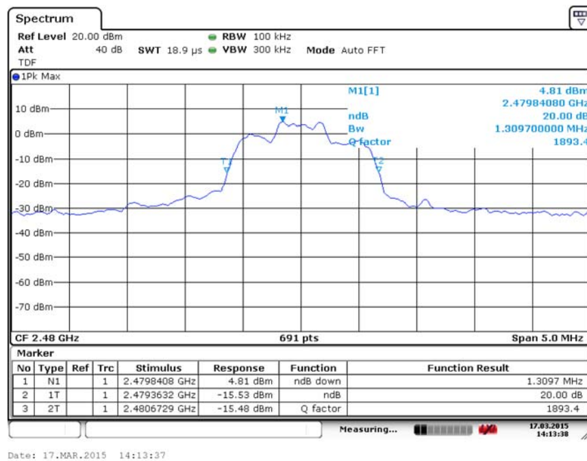
Fig. 91 Occupied 20dB Bandwidth (8DPSK, Ch 78)
