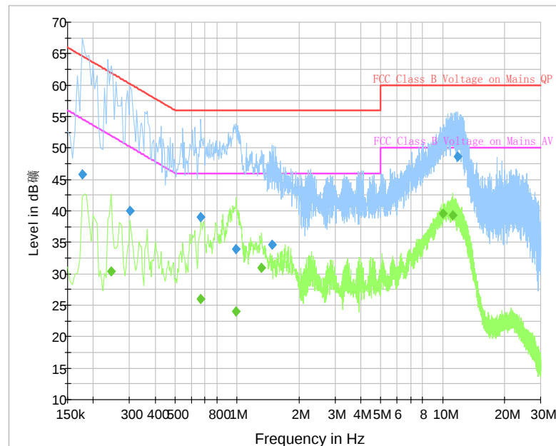
Fig. 108 AC Power line Conducted Emission (Traffic, AE2)
