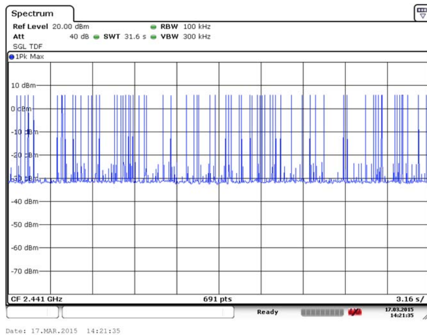
Fig. 95 Number of Transmissions ( \pi/4 DQPSK, Ch39)
