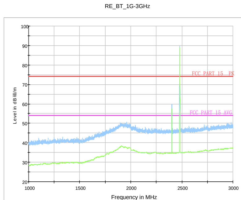
Fig. 60 Radiated Spurious Emission (GFSK, Ch78, 1 GHz ~3 GHz)
