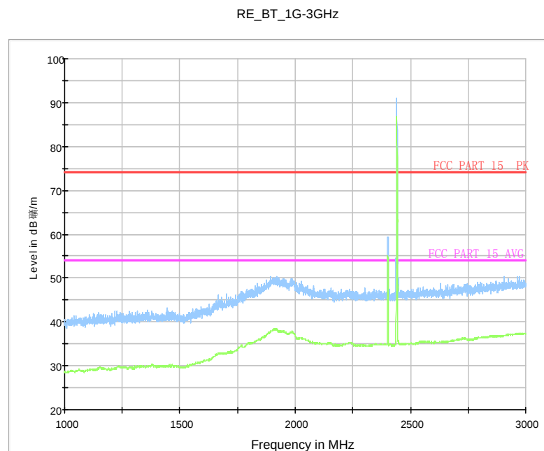
Fig. 76 Radiated Spurious Emission (8DPSK, Ch39, 1 GHz ~3 GHz)
