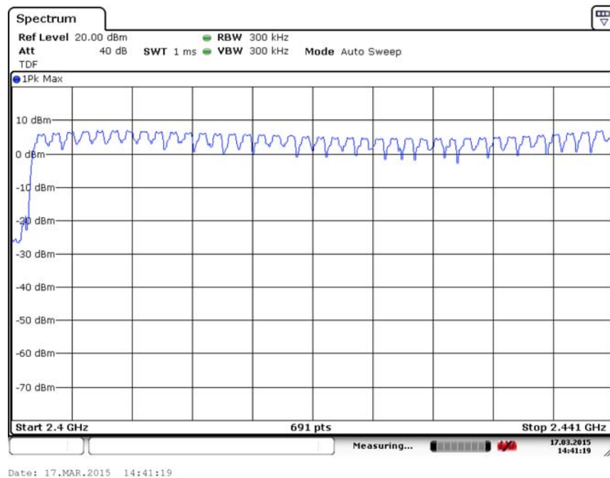
Fig. 100 Hopping channel ch0~39 ( \pi/4 DQPSK, Ch39)
