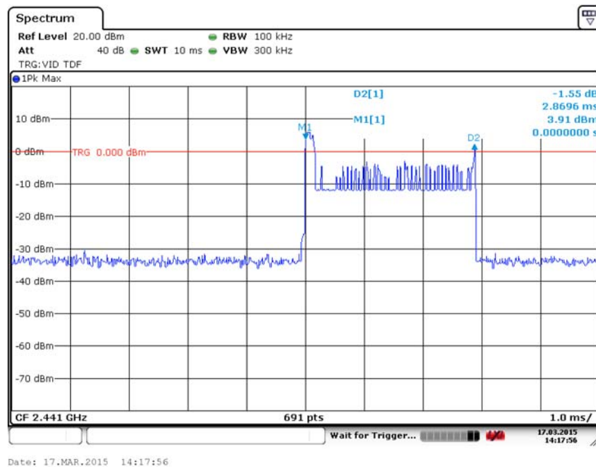
Fig. 94 Time of Occupancy(Dwell Time) ( \pi/4 DQPSK, Ch39)
