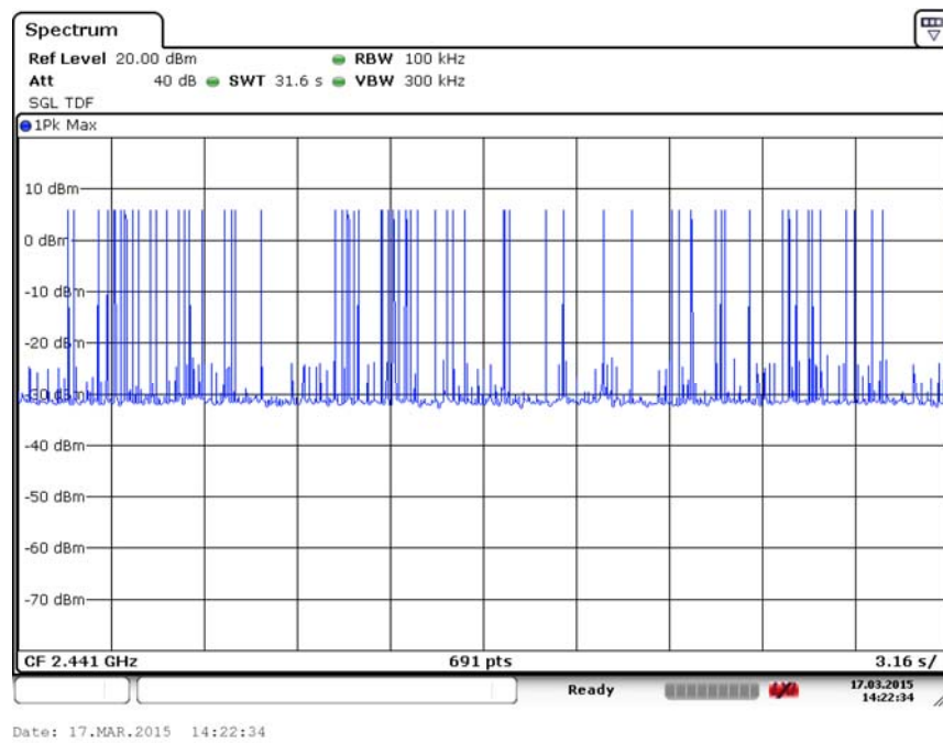
Fig. 97 Number of Transmissions (8DPSK, Ch39)
