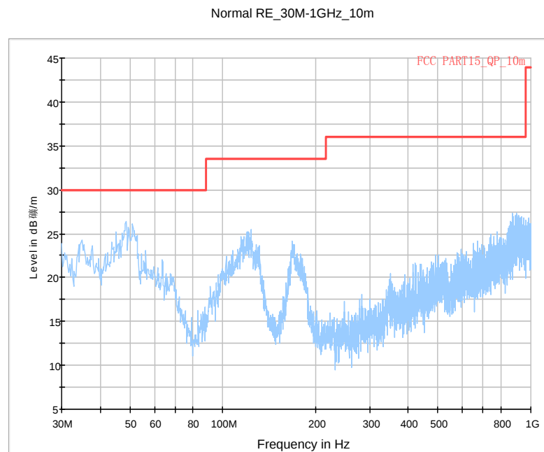
Fig. 75 Radiated Spurious Emission (8DPSK, Ch39, 30 MHz ~1 GHz)
