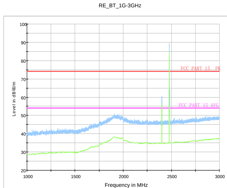
Fig. 78 Radiated Spurious Emission (8DPSK, Ch78, 1 GHz ~3 GHz)
