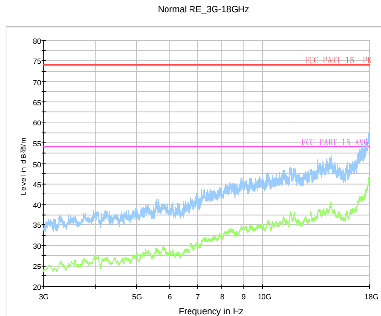
Fig. 74 Radiated Spurious Emission (8DPSK, Ch0, 3 GHz ~18 GHz)
