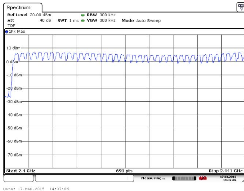
Fig. 102 Hopping channel ch0~39 (8DPSK, Ch39)
