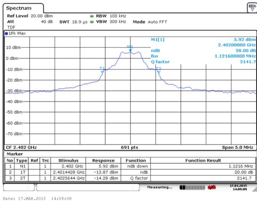
Fig. 83 Occupied 20dB Bandwidth (GFSK, Ch 0)
