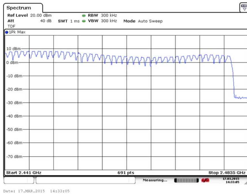
Fig. 101 Hopping channel ch39~78 ( \pi/4 DQPSK, Ch39)
