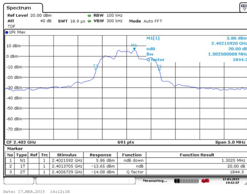
Fig. 89 Occupied 20dB Bandwidth (8DPSK, Ch 0)
