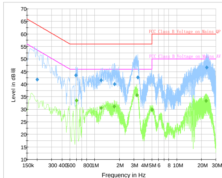
Fig. 109 AC Power line Conducted Emission (Traffic, AE3)
