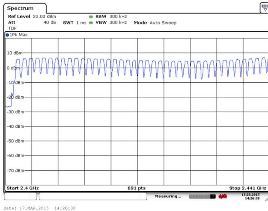
Fig. 98 Hopping channel ch0~39 (GFSK, Ch39)
