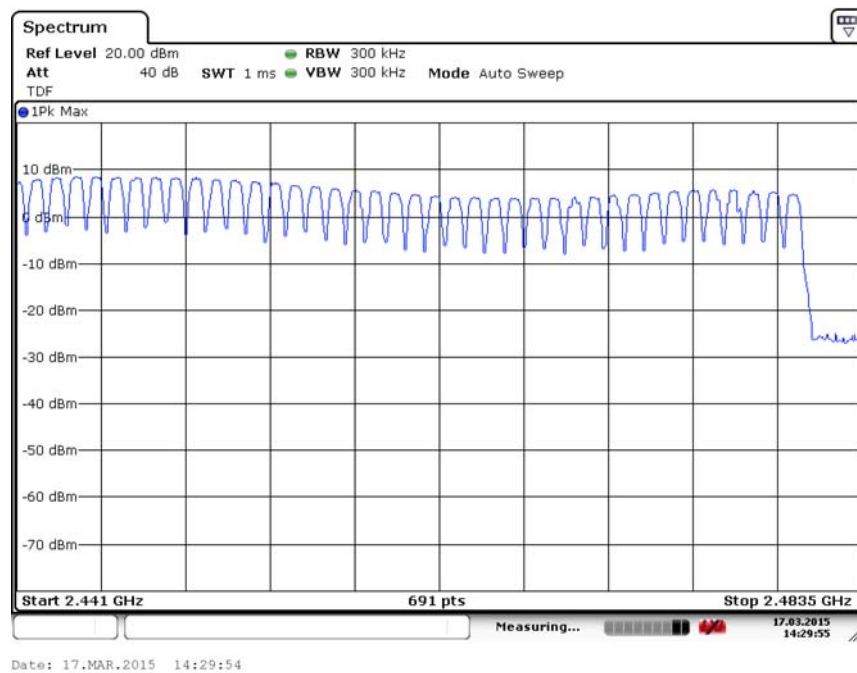
Fig. 99 Hopping channel ch39~78 (GFSK, Ch39)
