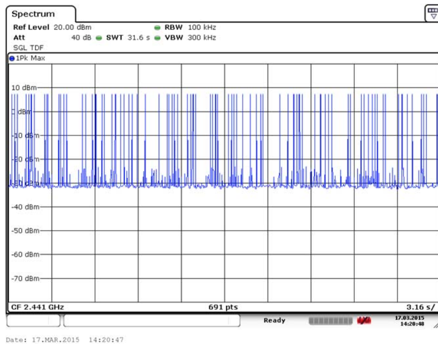
Fig. 93 Number of Transmissions (GFSK, Ch39)
