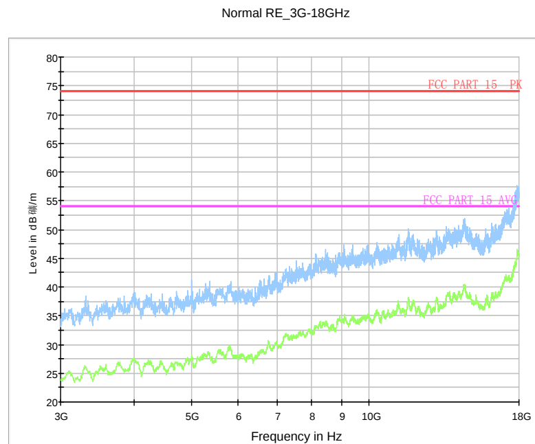
Fig. 59 Radiated Spurious Emission (GFSK, Ch39, 3 GHz ~18 GHz)
