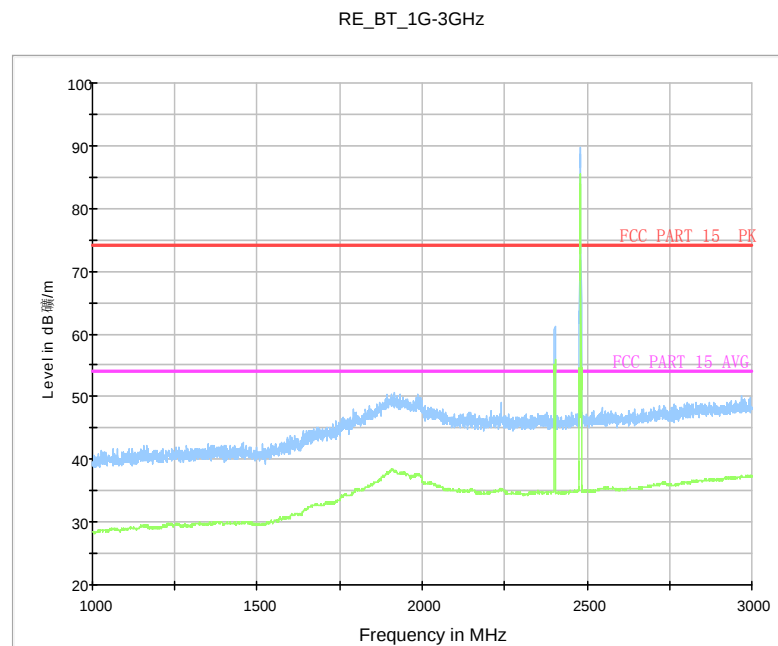
Fig. 69 Radiated Spurious Emission ( \pi/4 DQPSK, Ch78, 1 GHz ~3 GHz)
