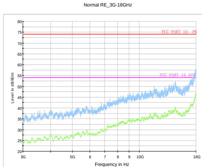
Fig. 70 Radiated Spurious Emission ( \pi/4 DQPSK, Ch78, 3 GHz ~18 GHz)
