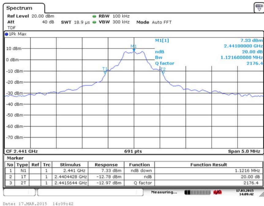
Fig. 84 Occupied 20dB Bandwidth (GFSK, Ch 39)
