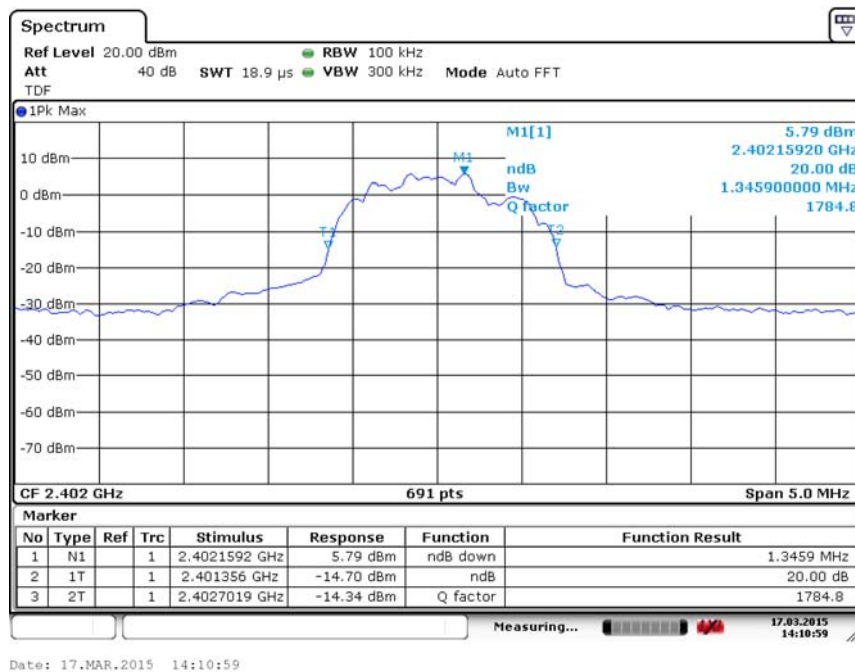
Fig. 86 Occupied 20dB Bandwidth ( \pi/4 DQPSK, Ch 0)
