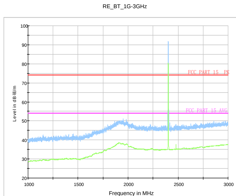
Fig. 56 Radiated Spurious Emission (GFSK, Ch0, 1 GHz ~3 GHz)
