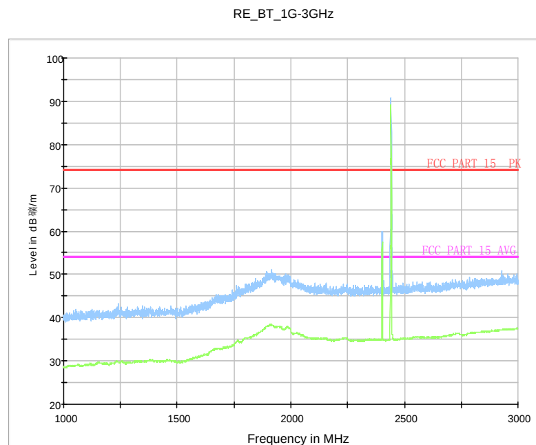
Fig. 58 Radiated Spurious Emission (GFSK, Ch39, 1 GHz ~3 GHz)
