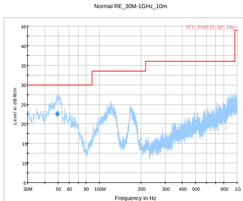
Fig. 66 Radiated Spurious Emission ( \pi/4 DQPSK, Ch39, 30 MHz ~1 GHz)
