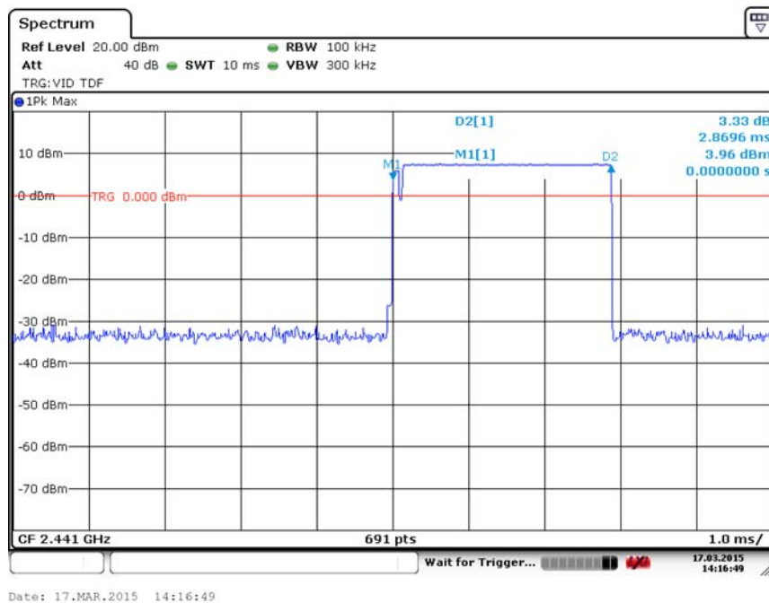
Fig. 92 Time of Occupancy(Dwell Time) (GFSK, Ch39)
