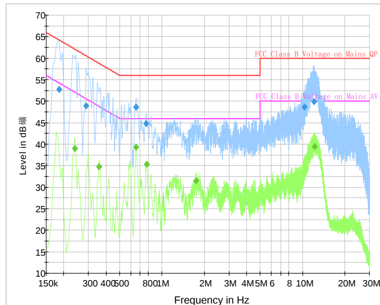
Fig. 111 AC Power line Conducted Emission (Traffic, AE5)
