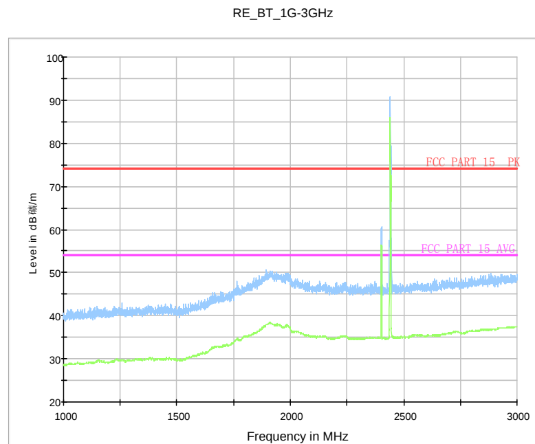
Fig. 67 Radiated Spurious Emission ( \pi/4 DQPSK, Ch39, 1 GHz ~3 GHz)
