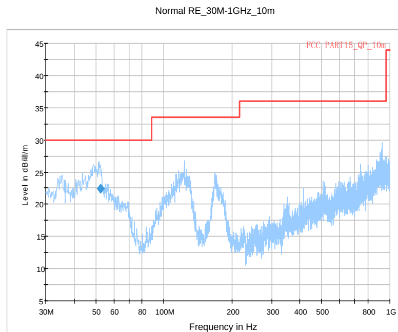
Fig. 50 Radiated Spurious Emission (GFSK, Ch0, 30 MHz ~1 GHz, AE1)
