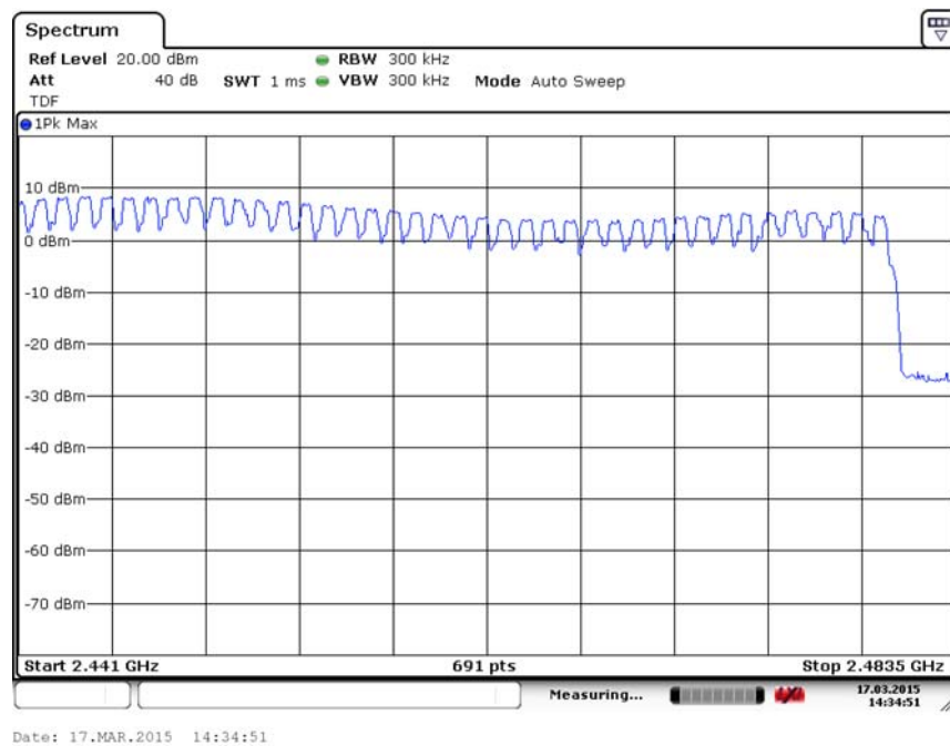
Fig. 103 Hopping channel ch39~78 (8DPSK, Ch39)
