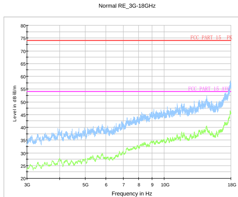
Fig. 57 Radiated Spurious Emission (GFSK, Ch39, 3 GHz ~18 GHz)
