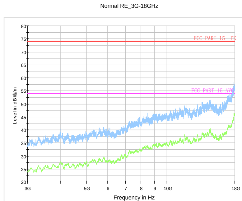
Fig. 65 Radiated Spurious Emission ( \pi/4 DQPSK, Ch0, 3 GHz ~18 GHz)
