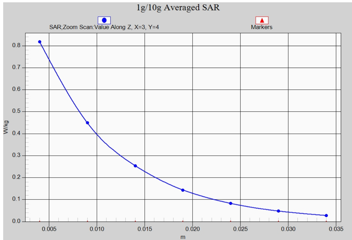
Fig. 7-1 Z-Scan at power reference point (LTE Band7)
