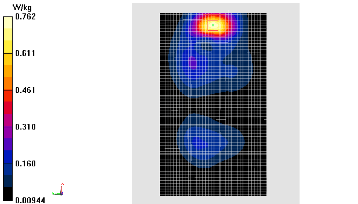
Fig.4 1900 MHz
