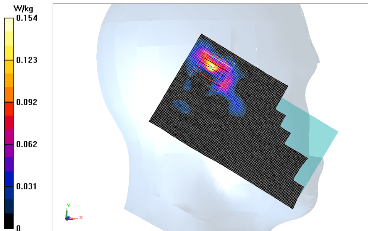
Fig.10 2450 MHz
