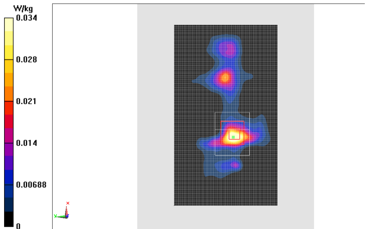
Fig.11 2450 MHz
