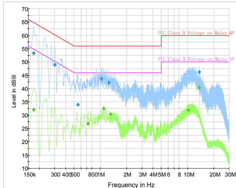
Fig. 14 AC Power line Conducted Emission (Traffic, AE1)
