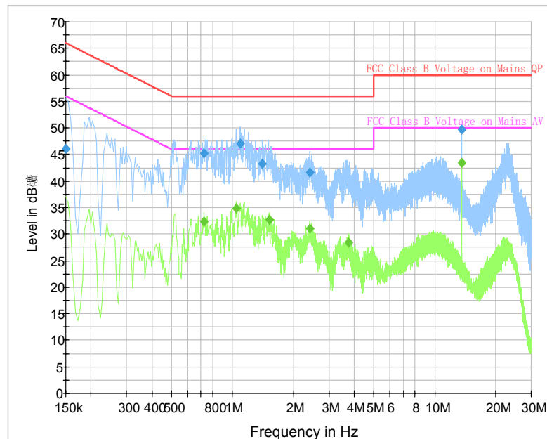
Fig. 18 AC Power line Conducted Emission (Traffic, AE5)
