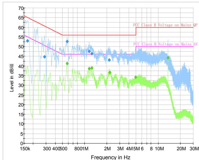
Fig. 21 AC Power line Conducted Emission (Traffic, AE8)
