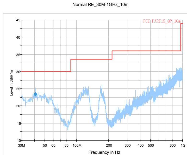
Fig. 3 Radiated Emission \geq 30 MHz (AE1)
