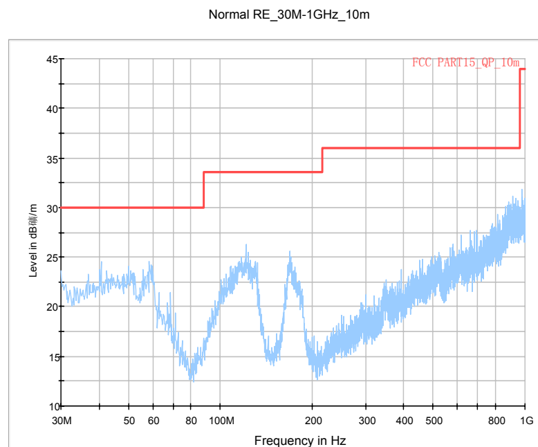
Fig. 6 Radiated Emission \geq 30 MHz (AE4)
