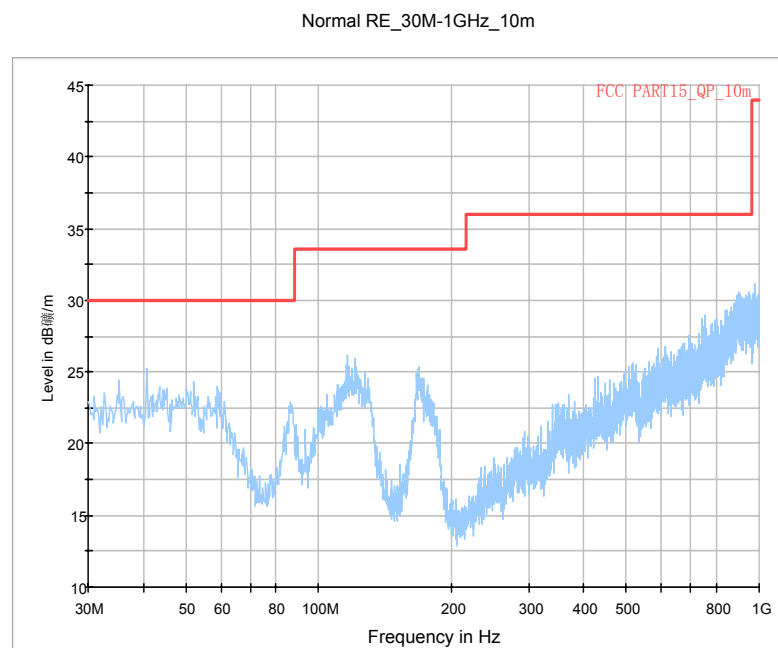
Fig. 9 Radiated Emission \geq 30 MHz (AE7)
