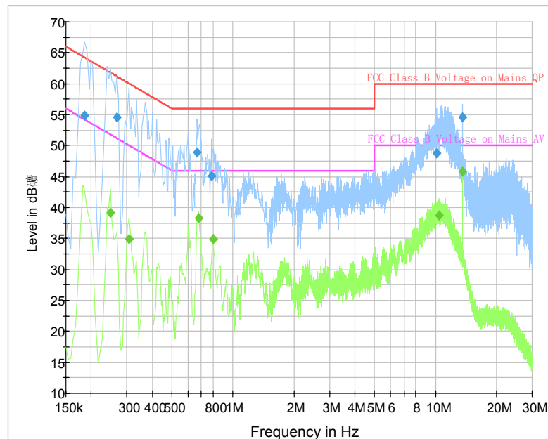
Fig. 15 AC Power line Conducted Emission (Traffic, AE2)
