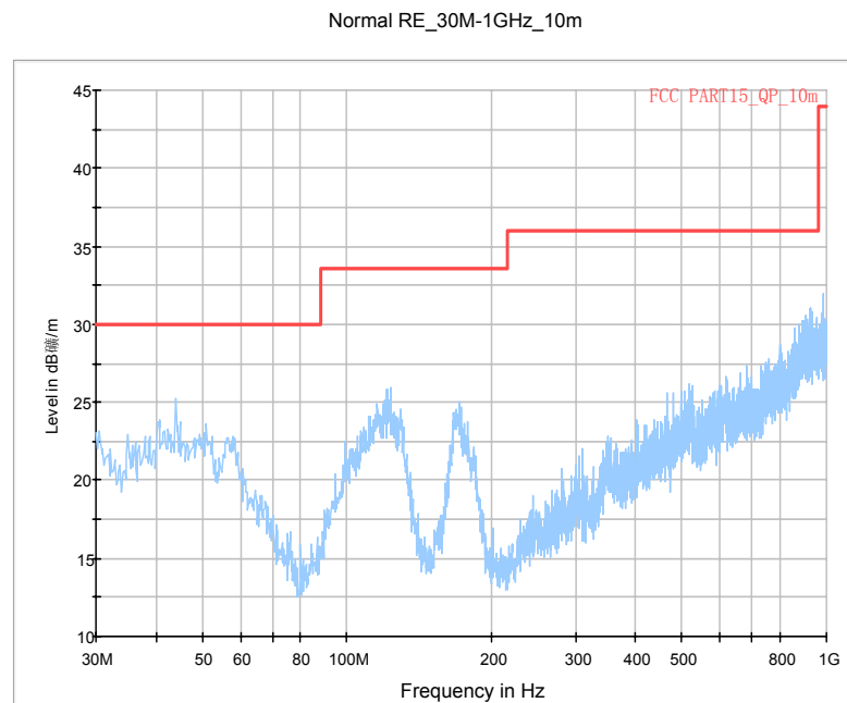
Fig. 5 Radiated Emission \geq 30 MHz (AE3)
