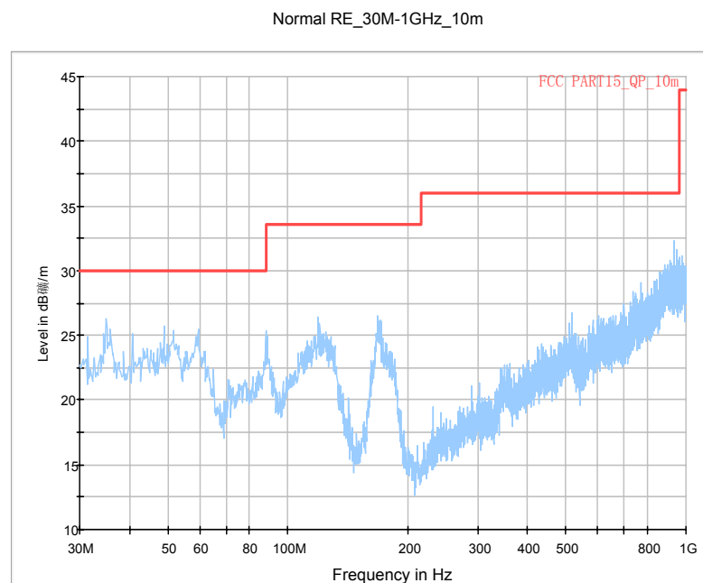
Fig. 8 Radiated Emission \geq 30 MHz (AE6)
