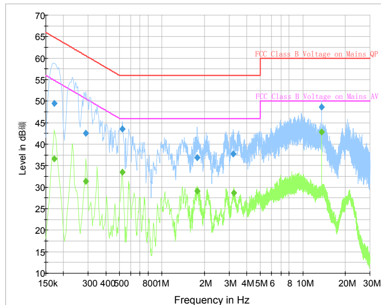
Fig. 20 AC Power line Conducted Emission (Traffic, AE7)
