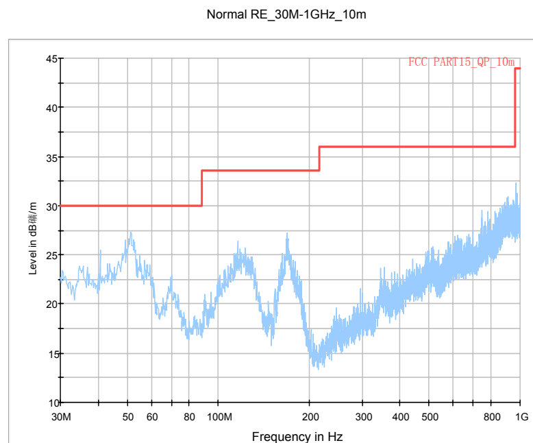
Fig. 12 Radiated Emission \geq 30 MHz (AE10)
