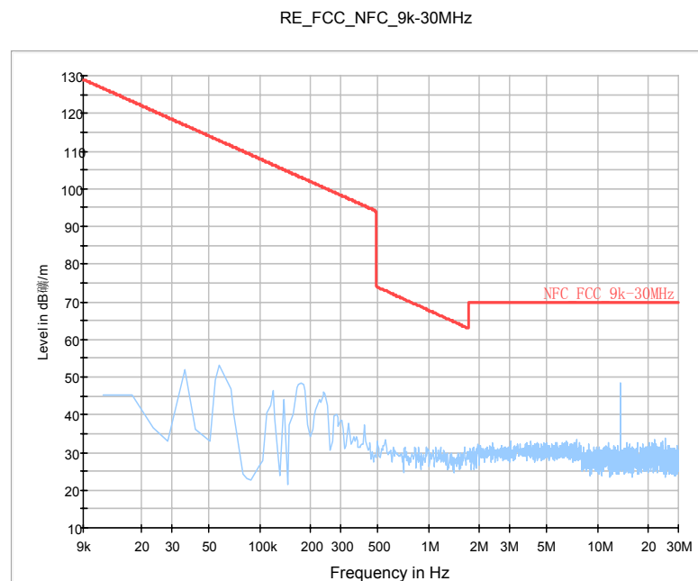
Fig. 2 Radiated Emission Below 30 MHz
