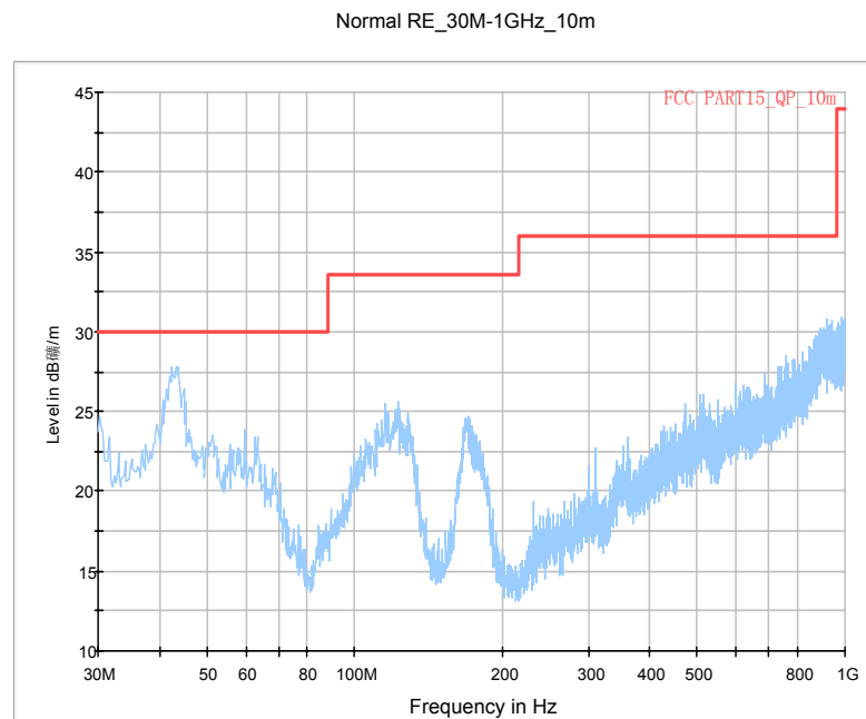
Fig. 7 Radiated Emission \geq 30 MHz (AE5)
