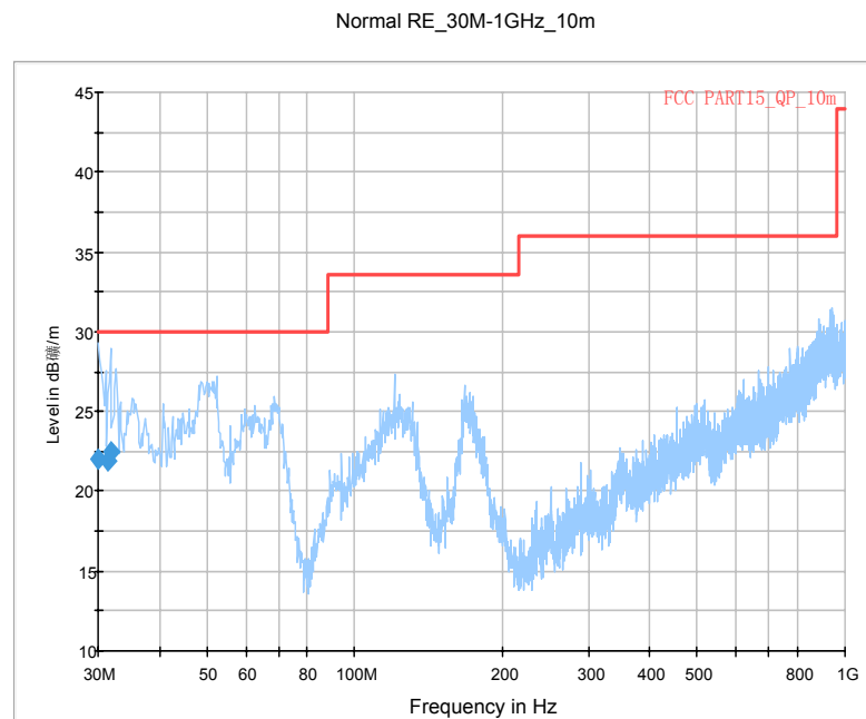
Fig. 11 Radiated Emission \geq 30 MHz (AE9)
