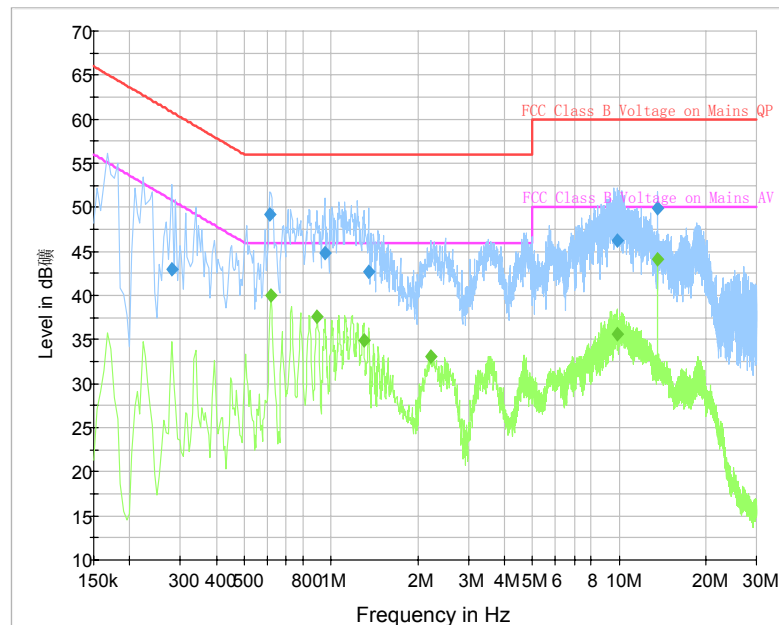
Fig. 22 AC Power line Conducted Emission (Traffic, AE9)
