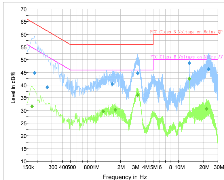
Fig. 16 AC Power line Conducted Emission (Traffic, AE3)
