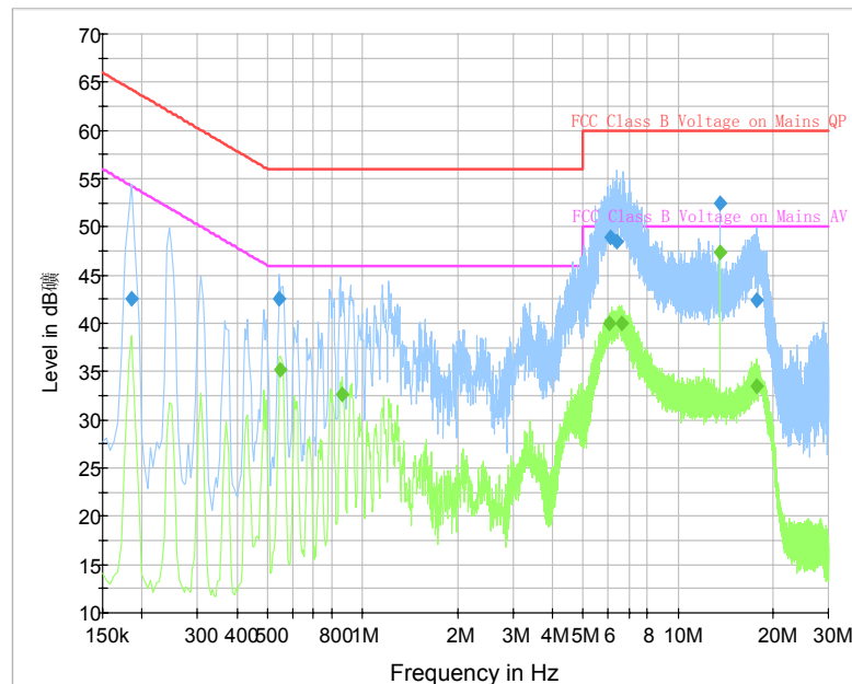
Fig. 17 AC Power line Conducted Emission (Traffic, AE4)
