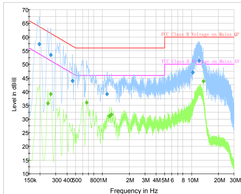
Fig. 23 AC Power line Conducted Emission (Traffic, AE10)
