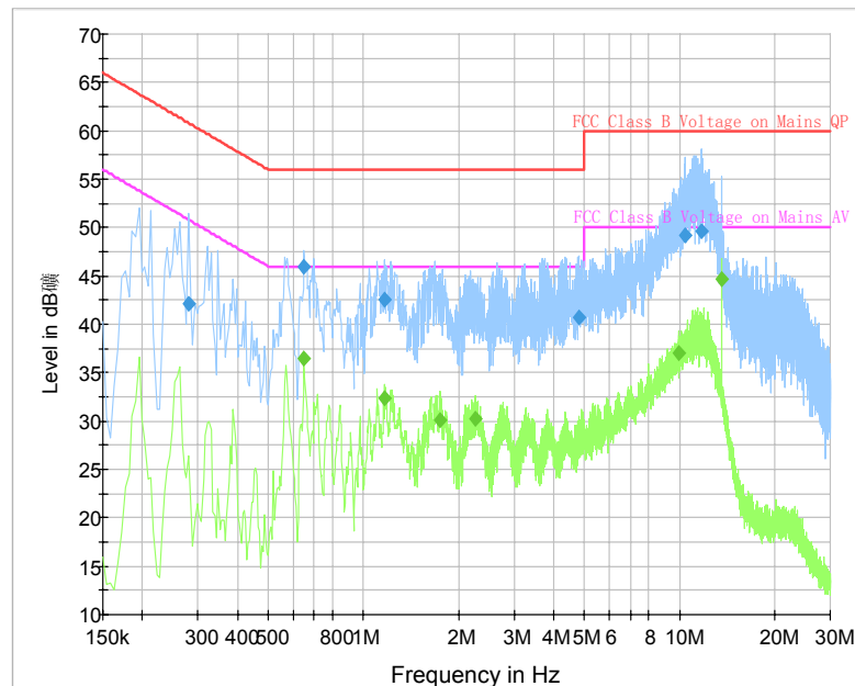
Fig. 19 AC Power line Conducted Emission (Traffic, AE6)
