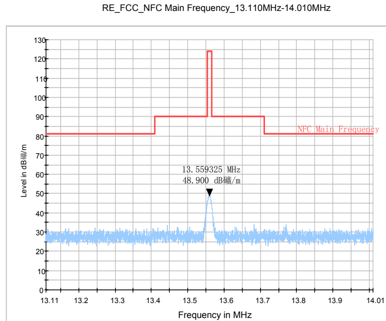
Fig. 1 In band and out of band electric field strength test (MASK)
