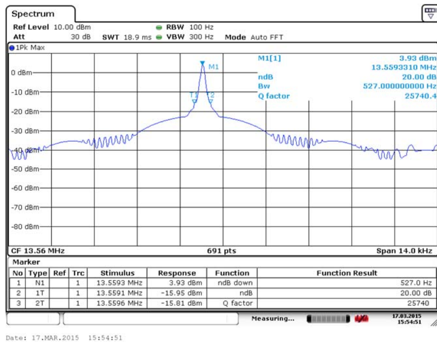
Fig. 13 Occupied 20dB Bandwidth
