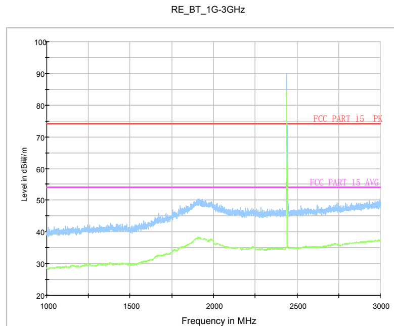
Fig.34 Radiated Spurious Emission (Ch19, 1 GHz-3 GHz)
