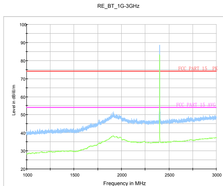
Fig.32 Radiated Spurious Emission (Ch0, 1 GHz-3 GHz)
