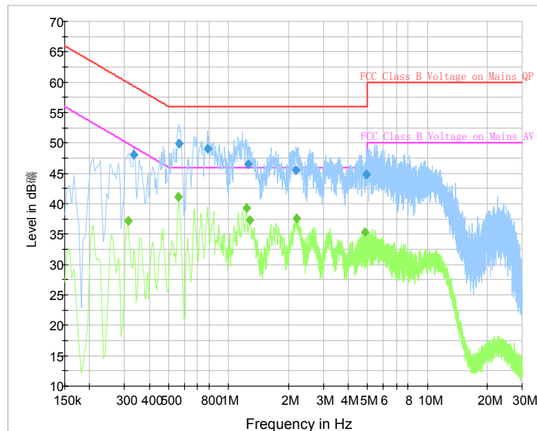
Fig. 48 AC Power line Conducted Emission (Traffic, AE8)
