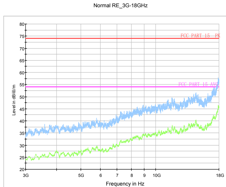
Fig.35 Radiated Spurious Emission (Ch19, 3 GHz-18 GHz)
