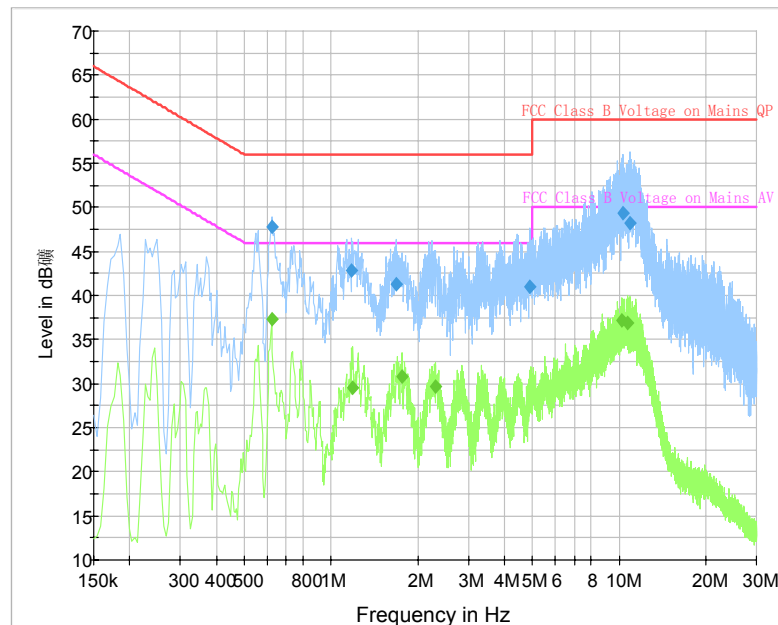
Fig. 46 AC Power line Conducted Emission (Traffic, AE6)
