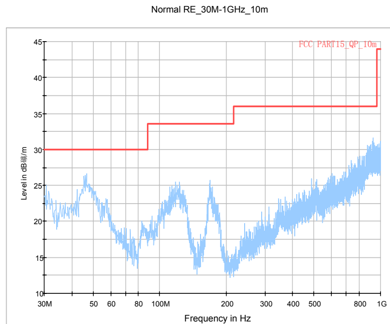
Fig. 29 Radiated Spurious Emission (GFSK, Ch0, 30 MHz ~1 GHz,AE8)
