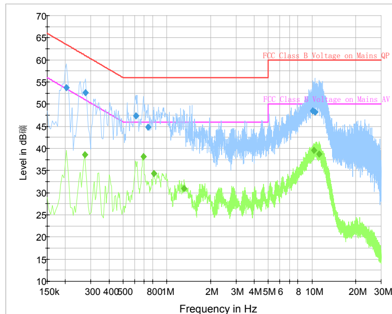
Fig. 42 AC Power line Conducted Emission (Traffic, AE2)
