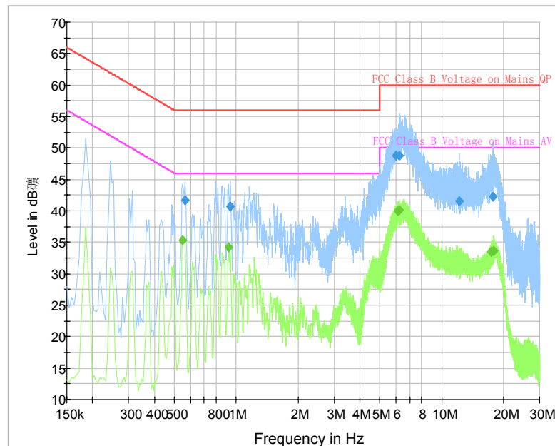
Fig. 44 AC Power line Conducted Emission (Traffic, AE4)
