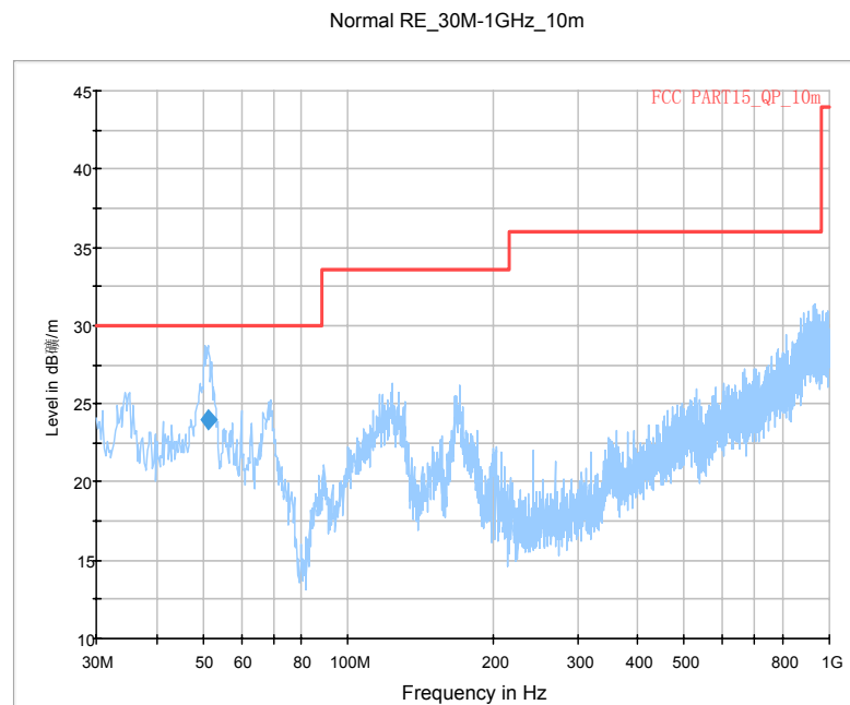
Fig. 26 Radiated Spurious Emission (GFSK, Ch0, 30 MHz ~1 GHz,AE5)
