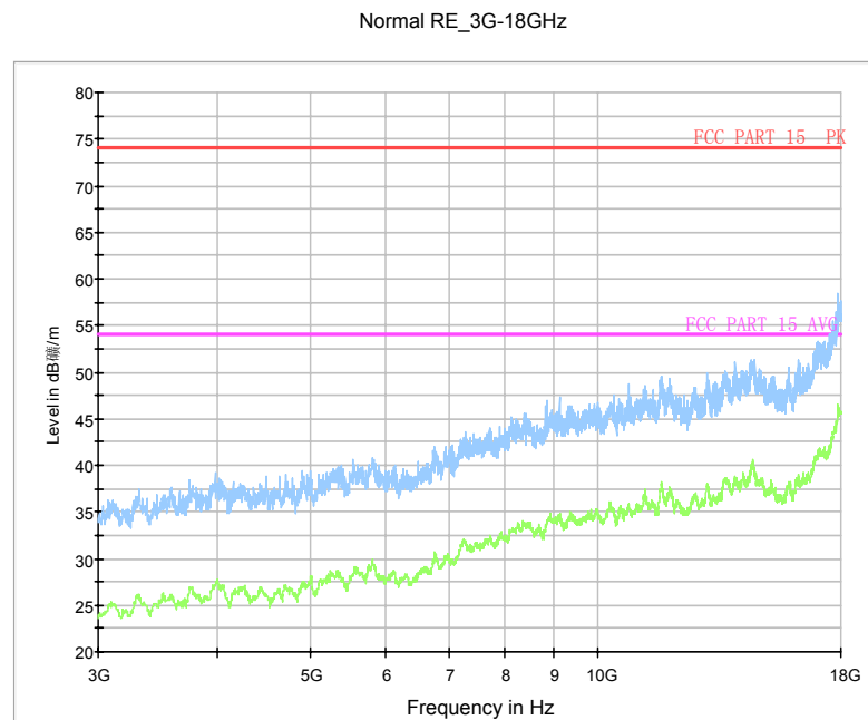
Fig.33 Radiated Spurious Emission (Ch0, 3 GHz-18 GHz)
