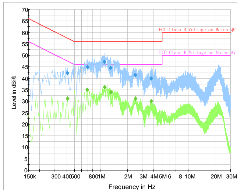
Fig. 45 AC Power line Conducted Emission (Traffic, AE5)
