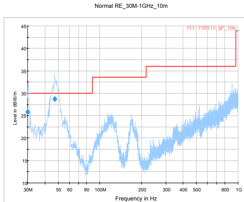
Fig. 28 Radiated Spurious Emission (GFSK, Ch0, 30 MHz ~1 GHz,AE7)
