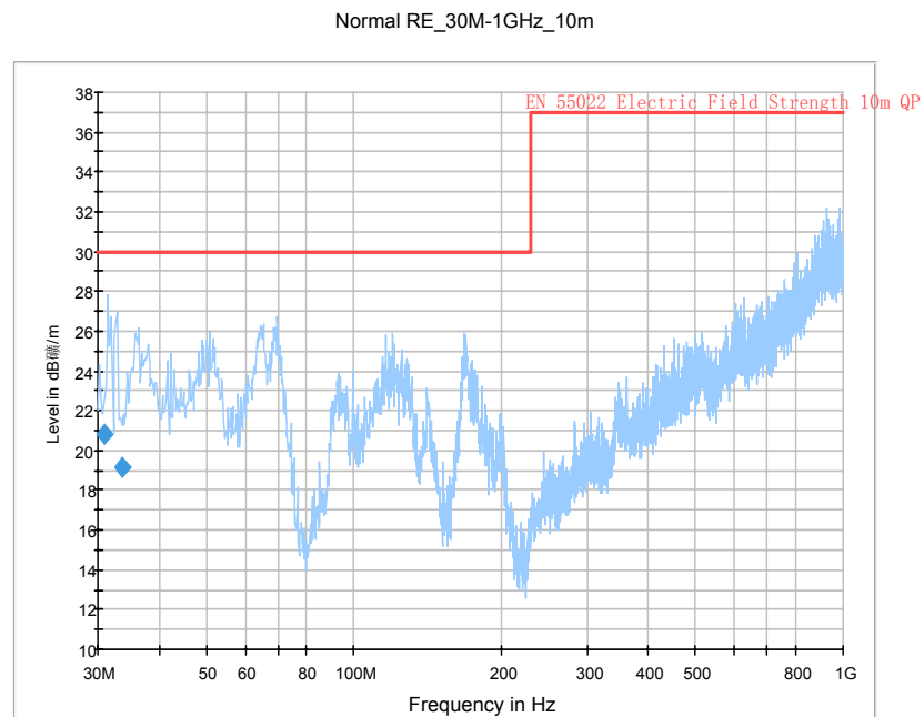
Fig. 30 Radiated Spurious Emission (GFSK, Ch0, 30 MHz ~1 GHz,AE9)
