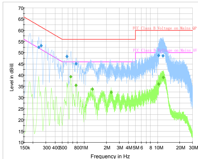
Fig. 49 AC Power line Conducted Emission (Traffic, AE9)
