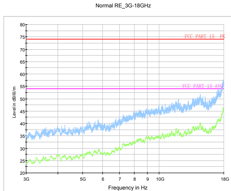
Fig.37 Radiated Spurious Emission (Ch39, 3 GHz-18 GHz)
