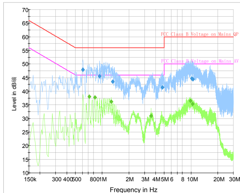
Fig. 50 AC Power line Conducted Emission (Traffic, AE10)
