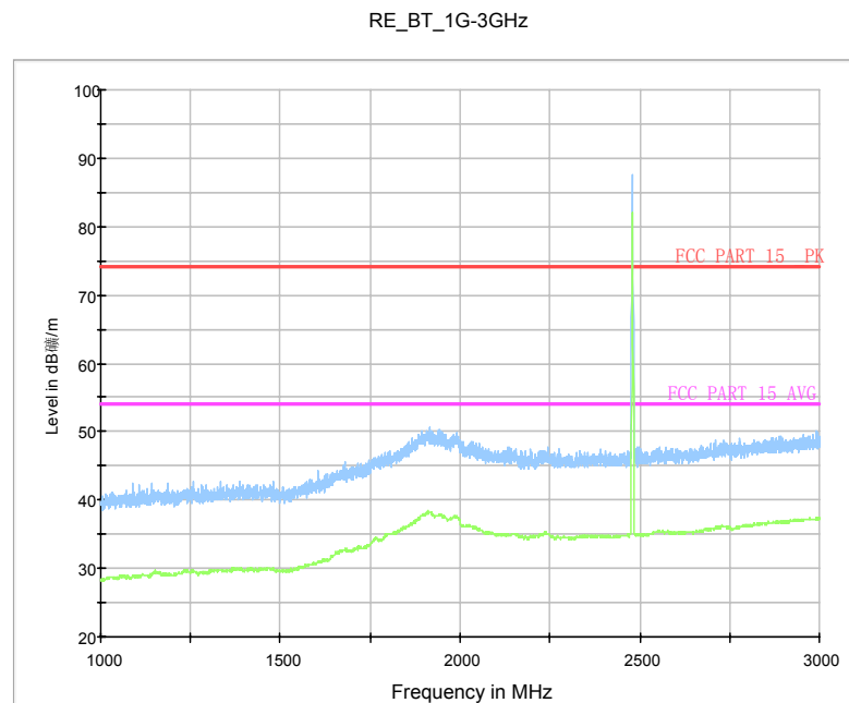
Fig.36 Radiated Spurious Emission (Ch39, 1 GHz-3 GHz)
