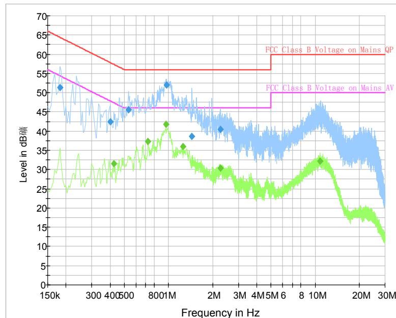
Fig. 41 AC Power line Conducted Emission (Traffic, AE1)
