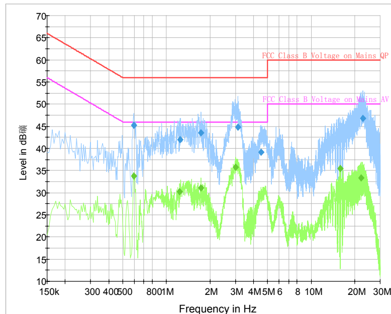
Fig. 43 AC Power line Conducted Emission (Traffic, AE3)
