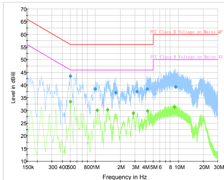
Fig. 47 AC Power line Conducted Emission (Traffic, AE7)
