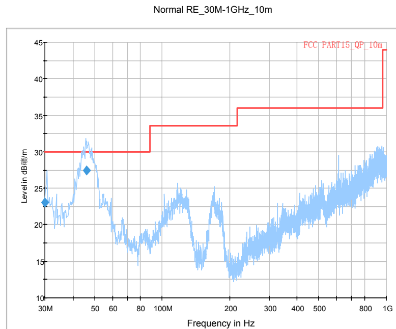
Fig. 31 Radiated Spurious Emission (GFSK, Ch0, 30 MHz ~1 GHz,AE10)
