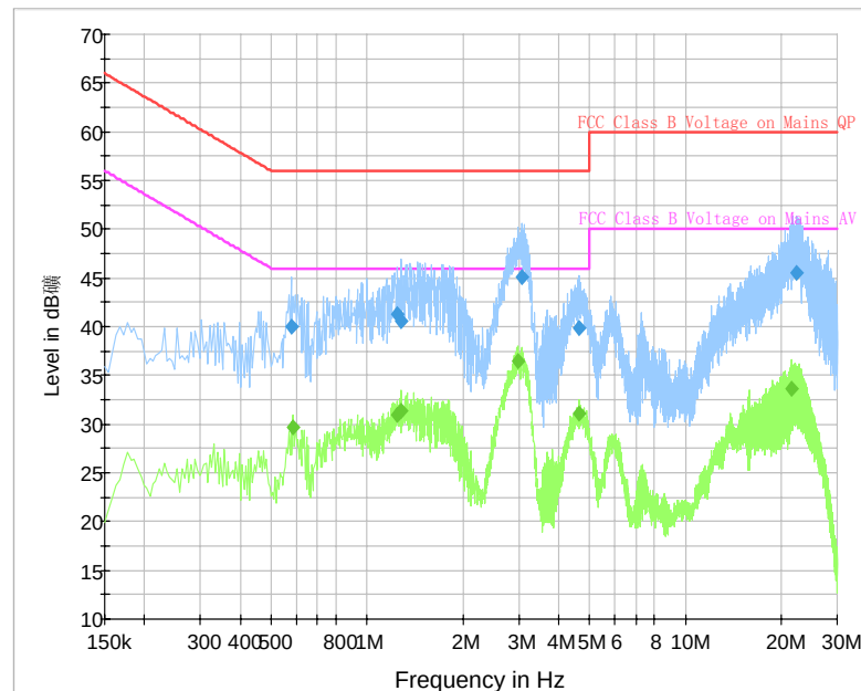
Fig. 114 AC Power line Conducted Emission (Traffic, AE4)
