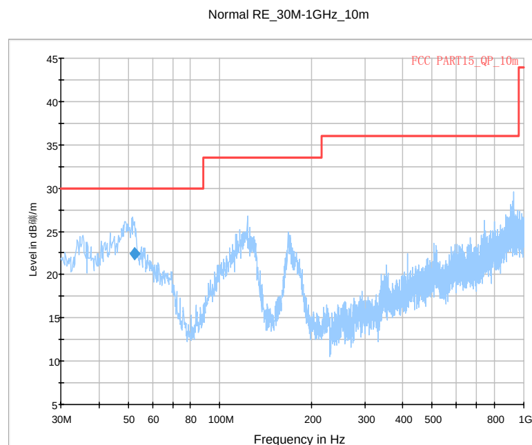
Fig. 50 Radiated Spurious Emission (GFSK, Ch0, 30 MHz ~1 GHz,AE1)
