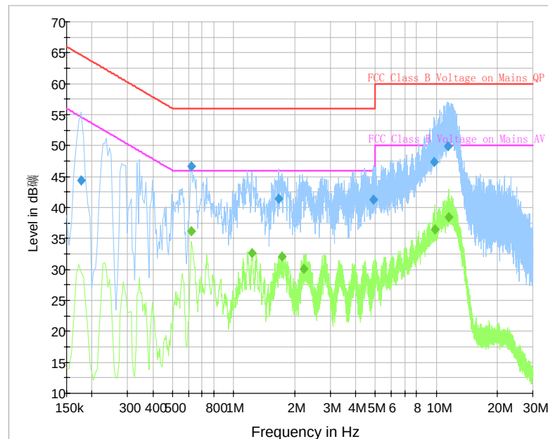
Fig. 116 AC Power line Conducted Emission (Traffic, AE6)
