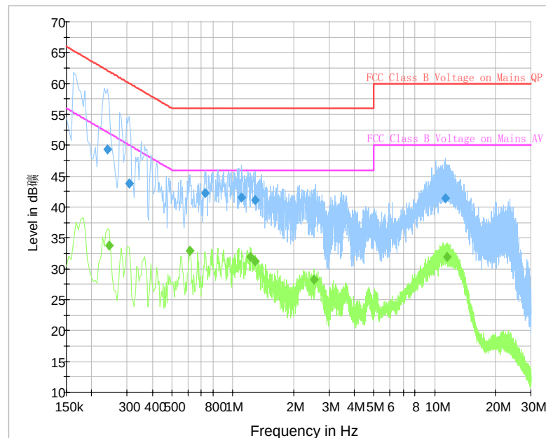
Fig. 111 AC Power line Conducted Emission (Traffic, AE1)
