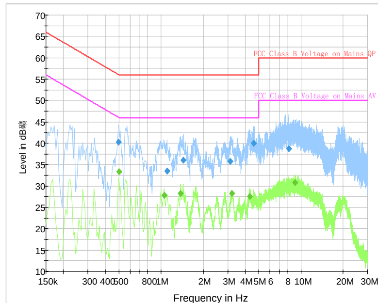
Fig. 117 AC Power line Conducted Emission (Traffic, AE7)
