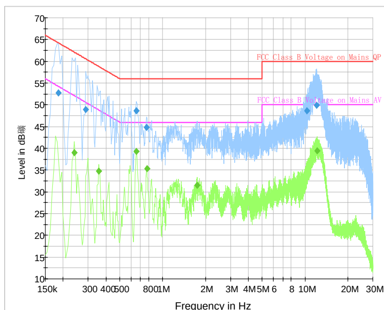
Fig. 119 AC Power line Conducted Emission (Traffic, AE9)
