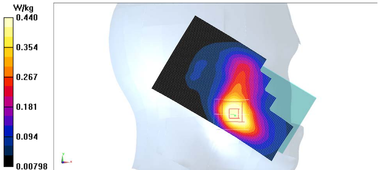
Fig.3 1900 MHz
