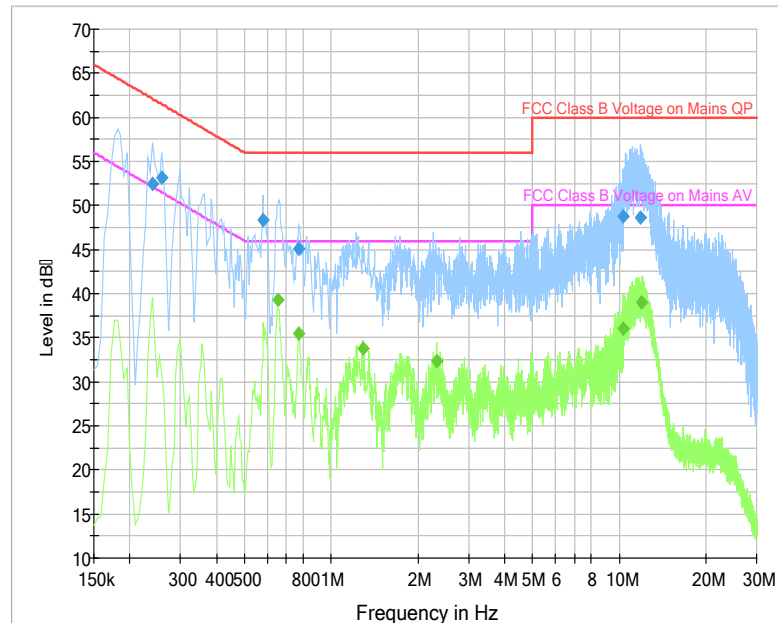
Fig. 49 AC Power line Conducted Emission (Traffic, AE9)
