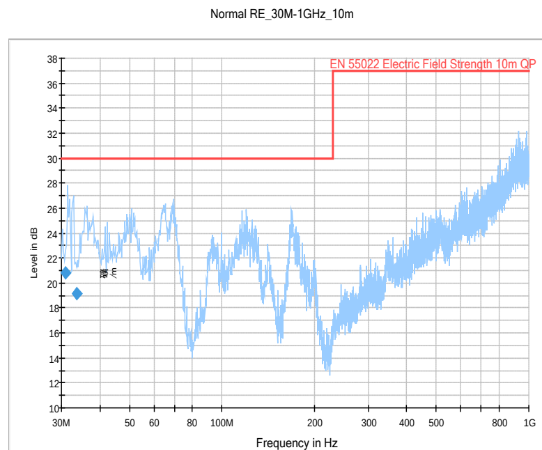
Fig. 30 Radiated Spurious Emission (GFSK, Ch0, 30 MHz ~1 GHz,AE9)
