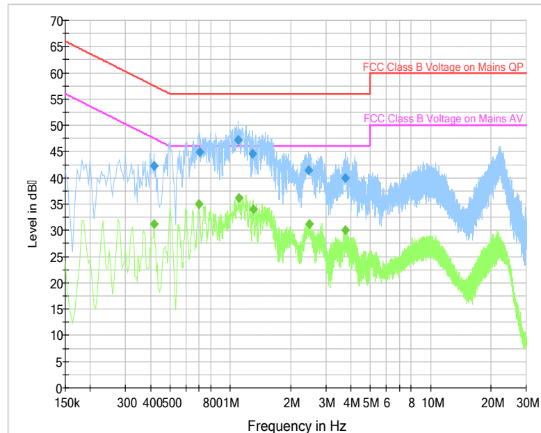
Fig. 45 AC Power line Conducted Emission (Traffic, AE5)
