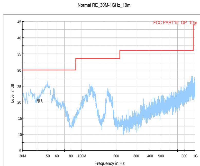
Fig. 22 Radiated Spurious Emission (GFSK, Ch0, 30 MHz ~1 GHz,AE1)
