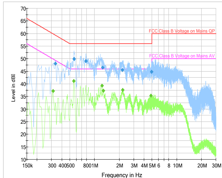
Fig. 48 AC Power line Conducted Emission (Traffic, AE8)
