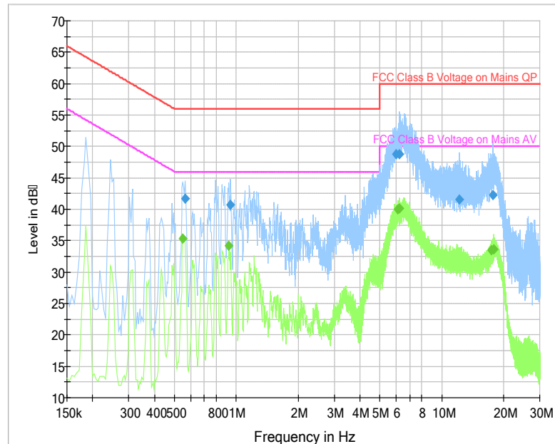
Fig. 44 AC Power line Conducted Emission (Traffic, AE4)
