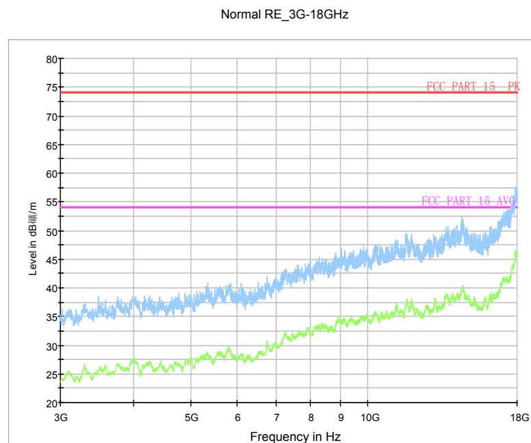
Fig.146 Radiated Spurious Emission (802.11n-20M, Ch11, 3 GHz-18 GHz)
