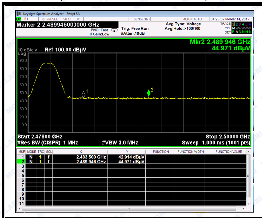
(Plot B2: Channel = 78 AVERAGE @ GFSK)
