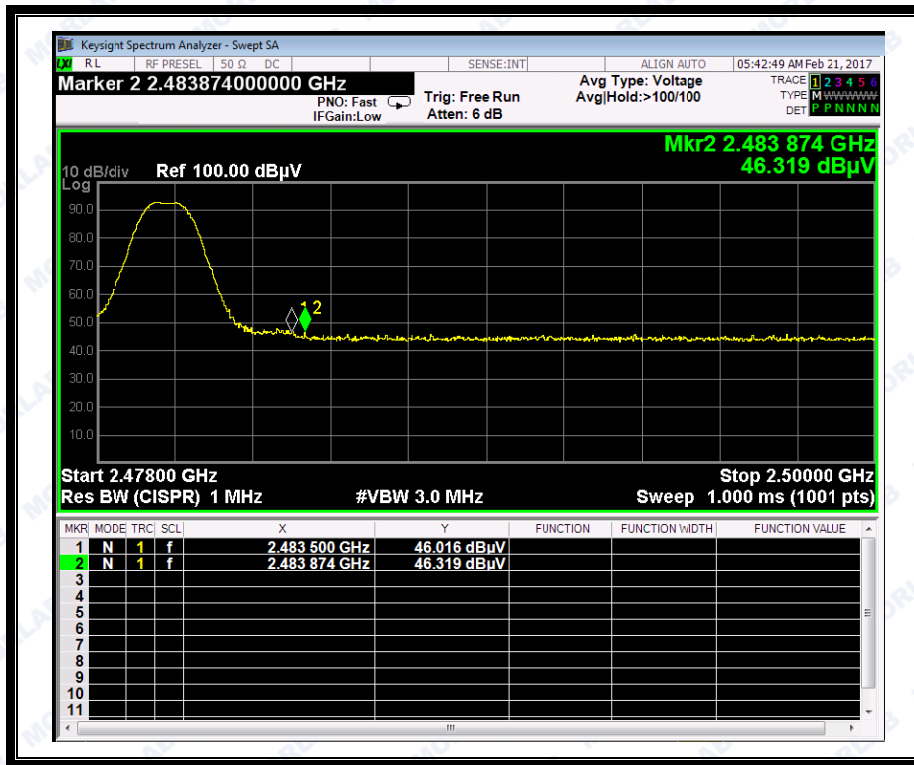
(Plot B1: Channel = 78 PEAK @ GFSK)
