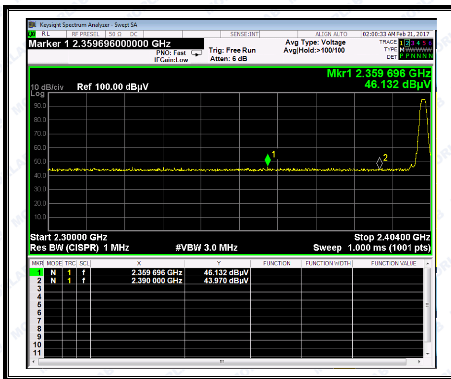
(Plot A1:Channel = 0 PEAK @ GFSK)
