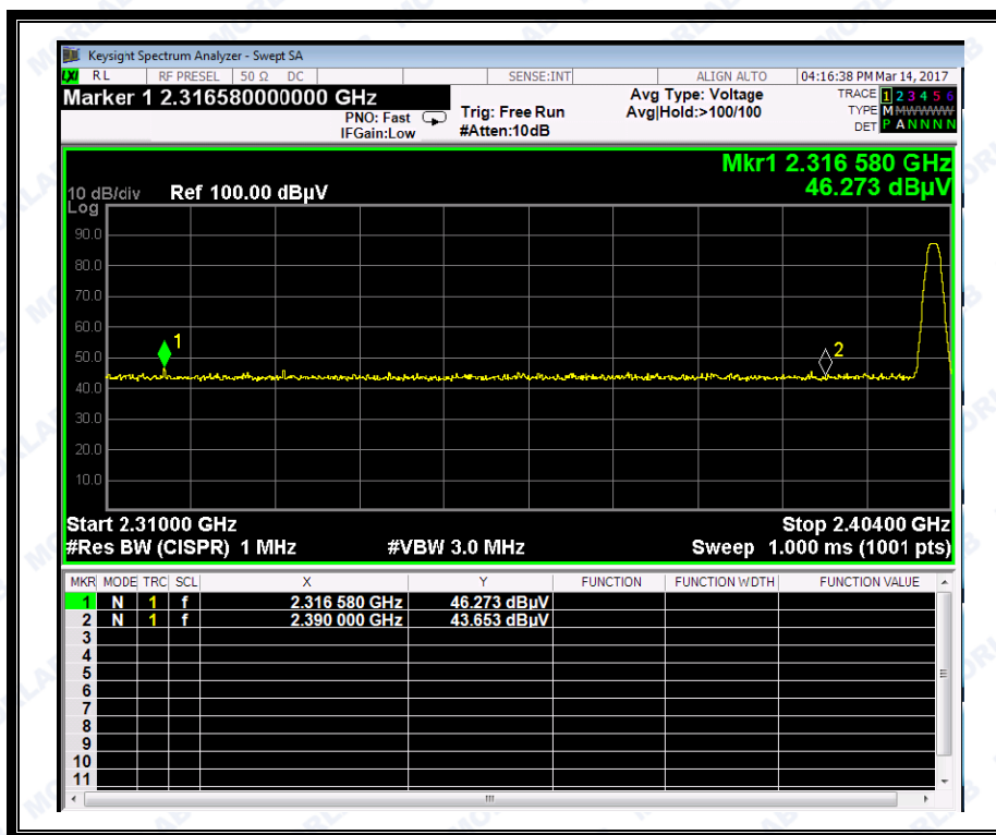
(Plot C2: Channel = 0 AVERAGE @ \pi/4 -DQPSK)
