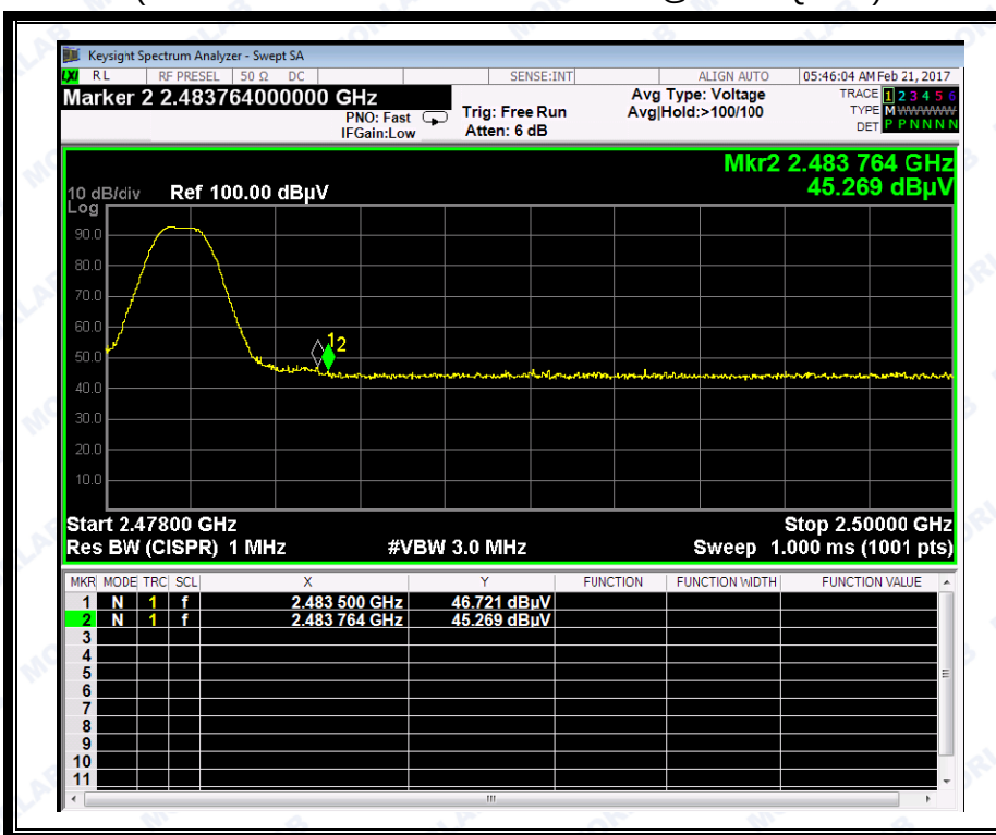
(Plot D1: Channel = 78 PEAK @ \pi/4 -DQPSK)
