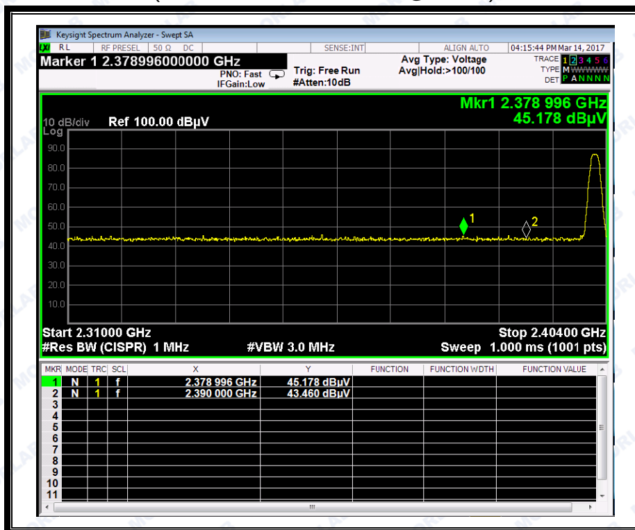
(Plot A2:Channel = 0 AVERAGE @ GFSK)
