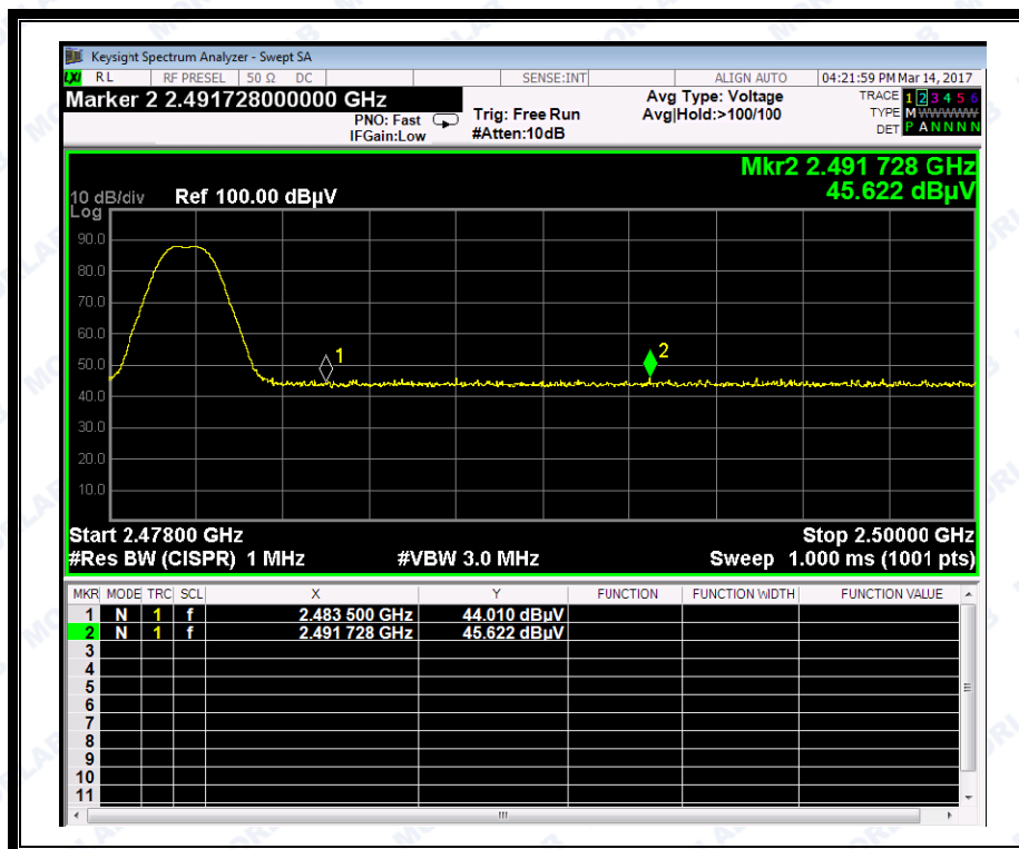
(Plot F2:Channel = 78 AVERAGE @ 8-DPSK Mode)
