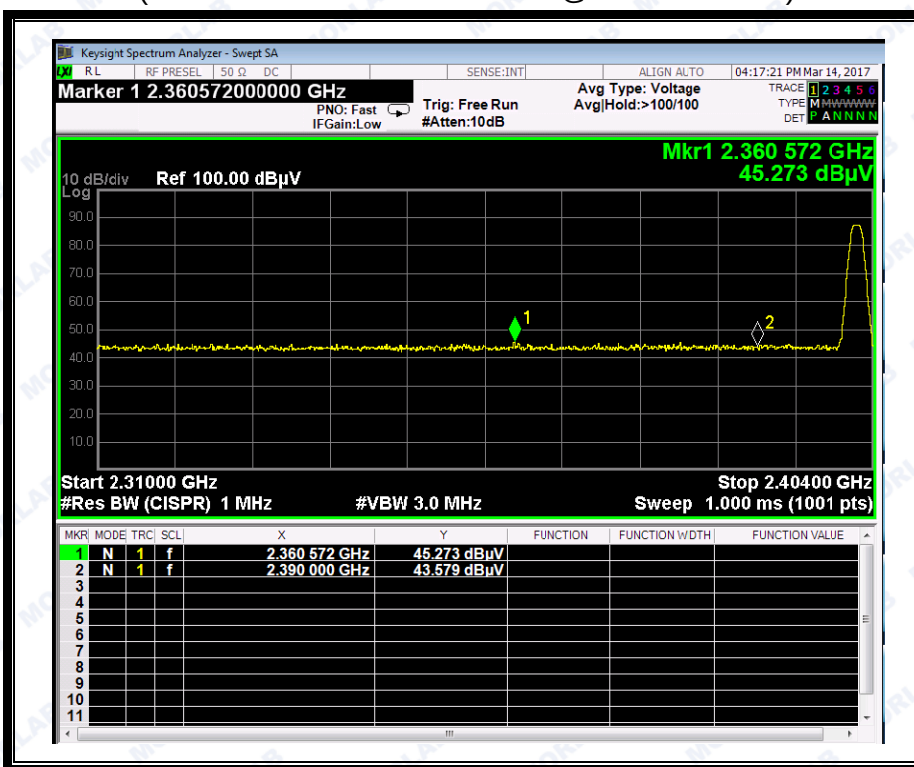
(Plot E2: Channel = 0 AVERAGE @ 8-DPSK Mode)
