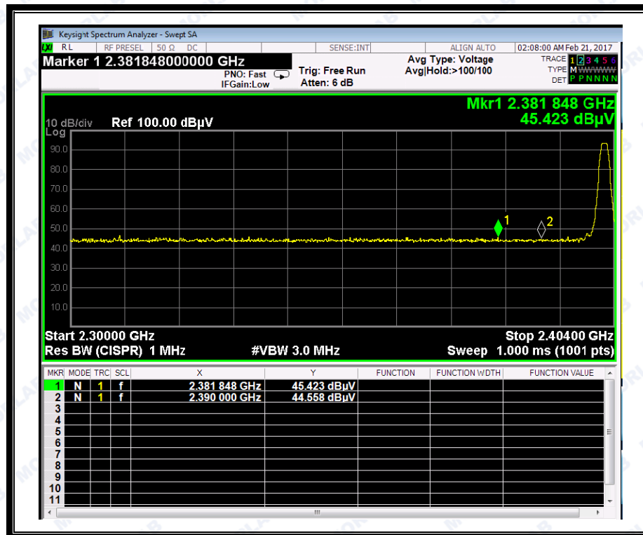
(Plot C1: Channel = 0 PEAK @ \pi/4 -DQPSK)
