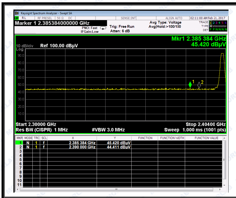
(Plot E1: Channel = 0 PEAK @ 8-DPSK Mode)
