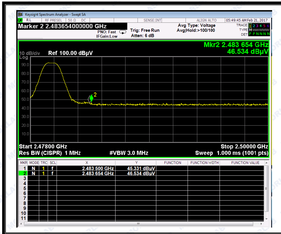
(Plot F1:Channel = 78 PEAK @ 8-DPSK Mode)
