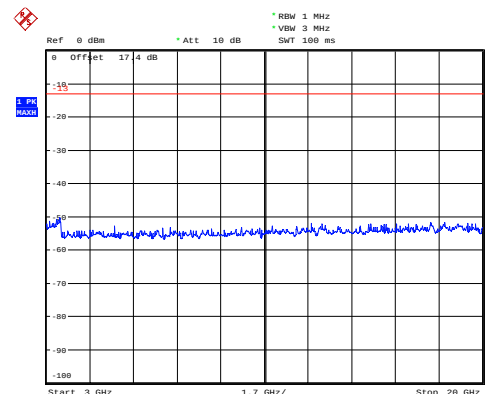
GSM 1900 CH-Middle 3GHz~20GHz
