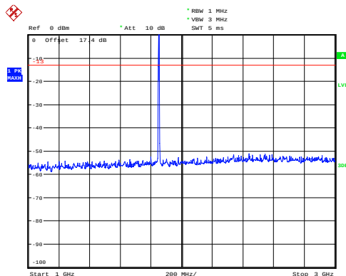
GSM 1900 CH-Low 1GHz~3GHz
