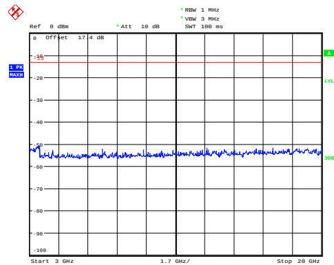
GSM 1900 CH-Low 3GHz~20GHz
