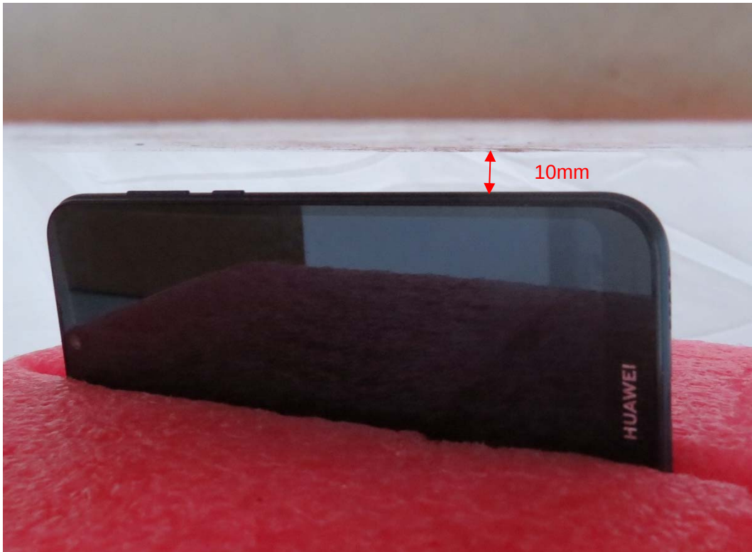
Picture 13: Right Side, the distance from handset to the bottom of the Phantom is 10mm
