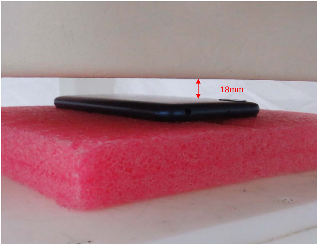
Picture 9: Back Side, the distance from handset to the bottom of the Phantom is 18mm
