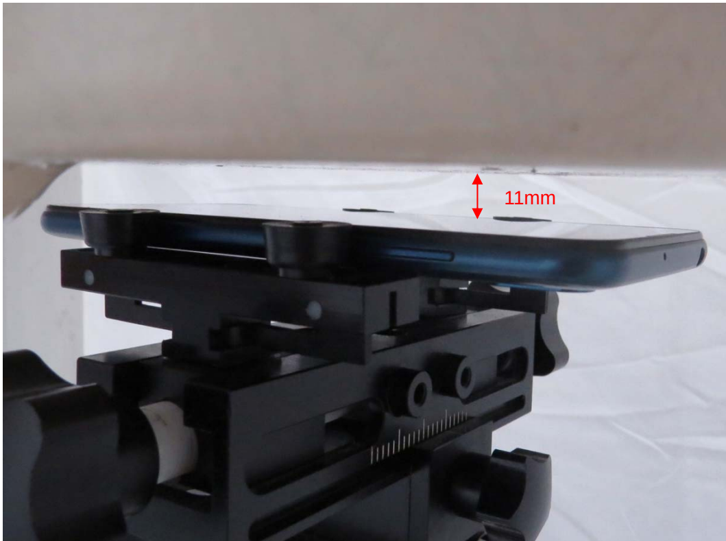
Picture 10: Front Side, the distance from handset to the bottom of the Phantom is 11mm
