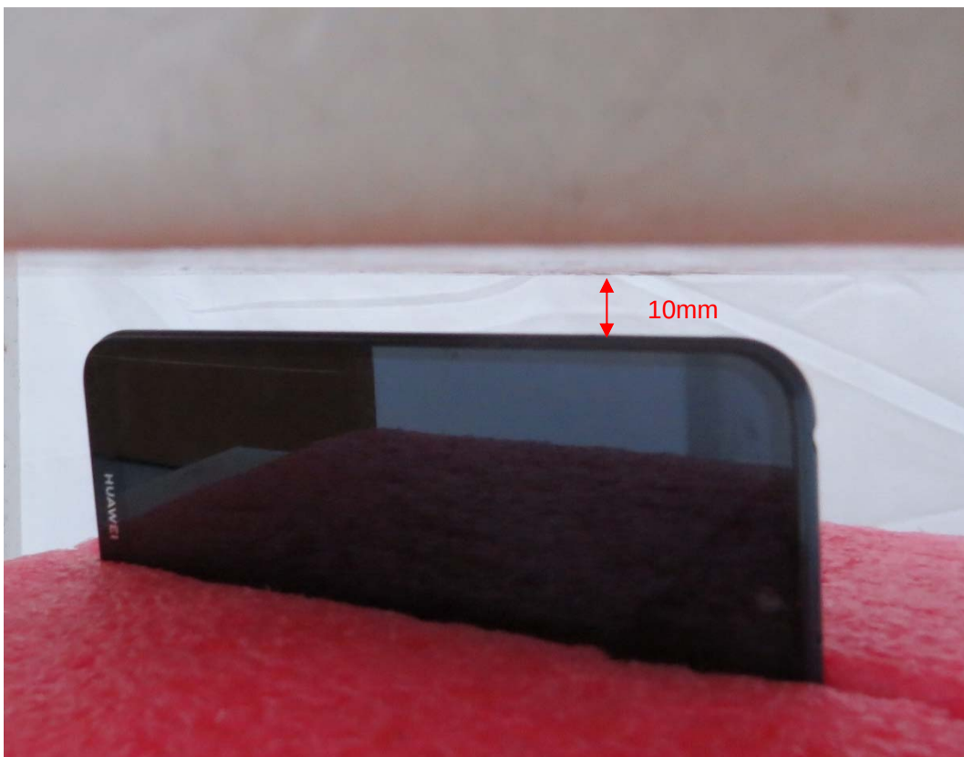
Picture 12: Left Side, the distance from handset to the bottom of the Phantom is 10mm
