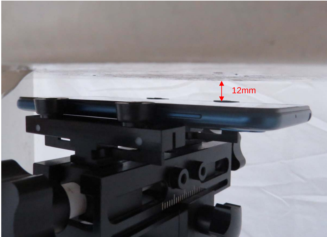
Picture 11: Front Side, the distance from handset to the bottom of the Phantom is 12mm
