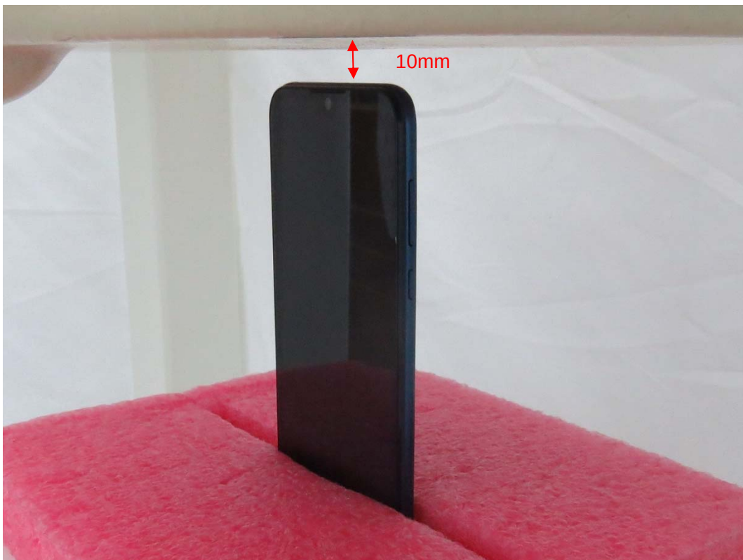
Picture 14: Top Side, the distance from handset to the bottom of the Phantom is 10mm
