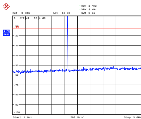
GSM 1900 CH-Low 1GHz~3GHz
