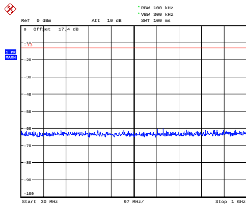
GSM 1900 CH-Low 30MHz~1GHz
