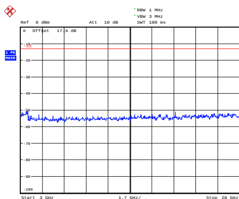
GSM 1900 CH-Low 3GHz~20GHz
