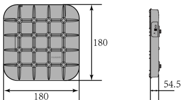
Figure 2-1 Dimension of AP4030DN (Unit: mm)
