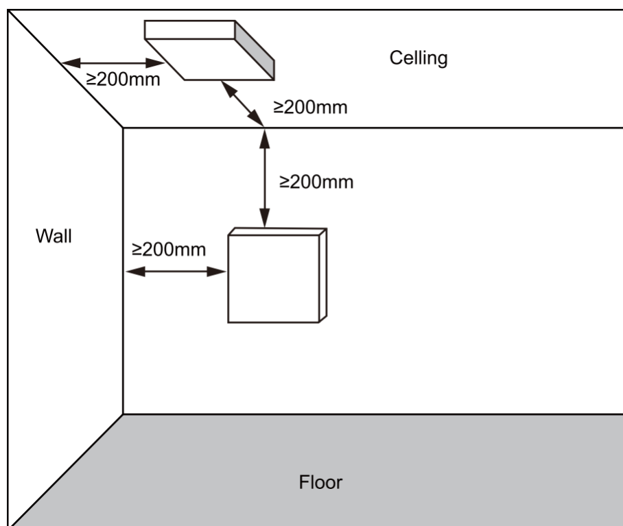
Figure 2-2 Mounting an AP (Unit: mm)
