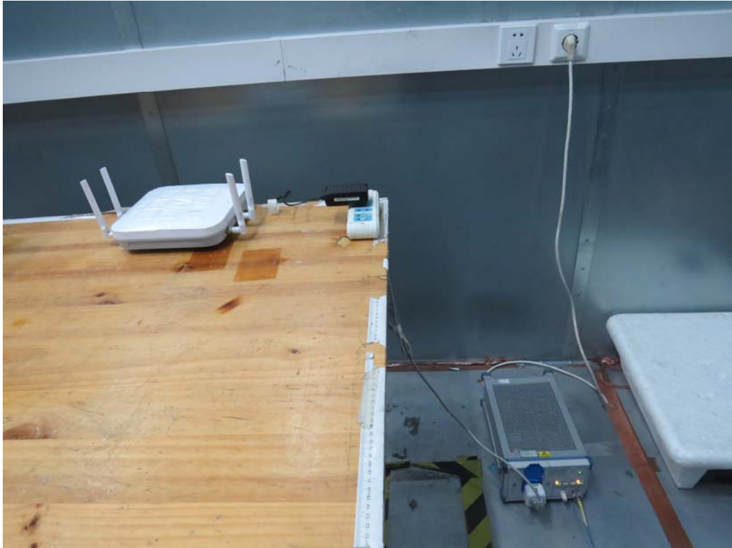
Picture 4 Conducted Emission Test Setup
