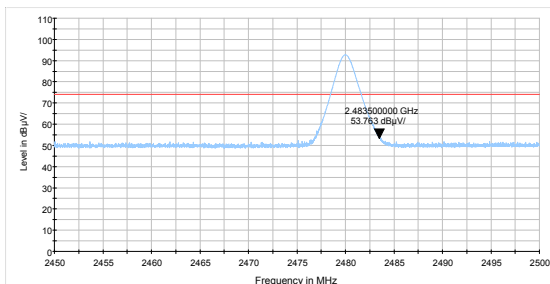
3DH5-Channel 78: Peak
