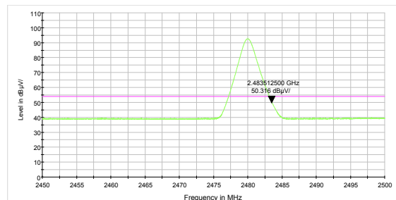
3DH5-Channel 78: Average
