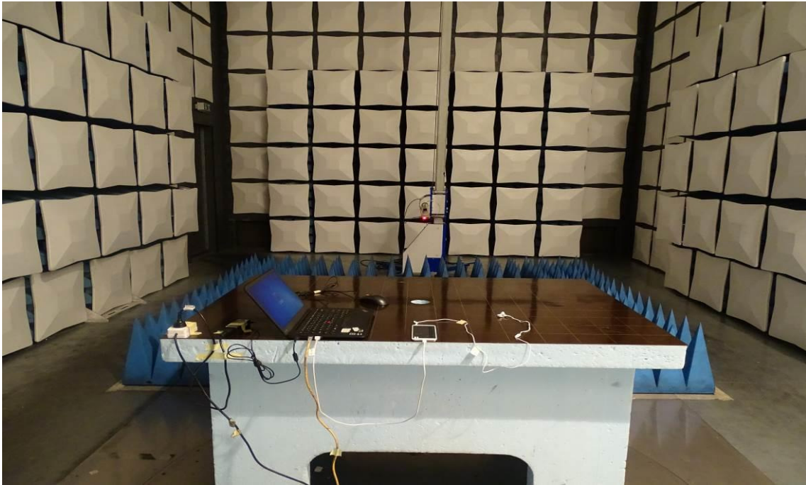
Radiated Disturbance Emissions (18GHz to26.5GHz)
