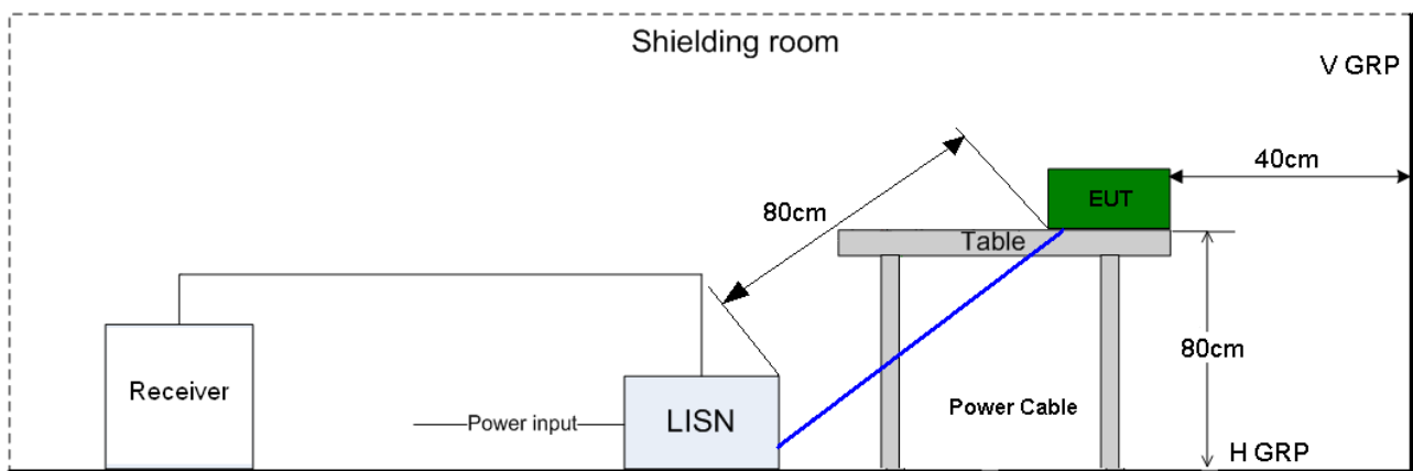
Figure 1. Test set-up of conducted disturbance for power port
