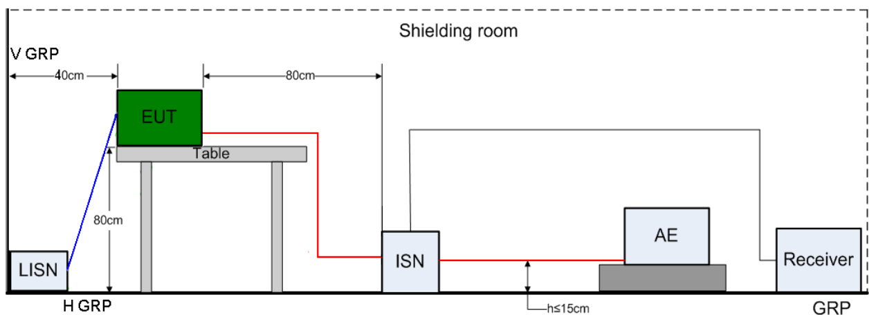
Figure 2. Test set-up of conducted disturbance for telecommunication ports
