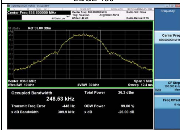
EDGE-190
