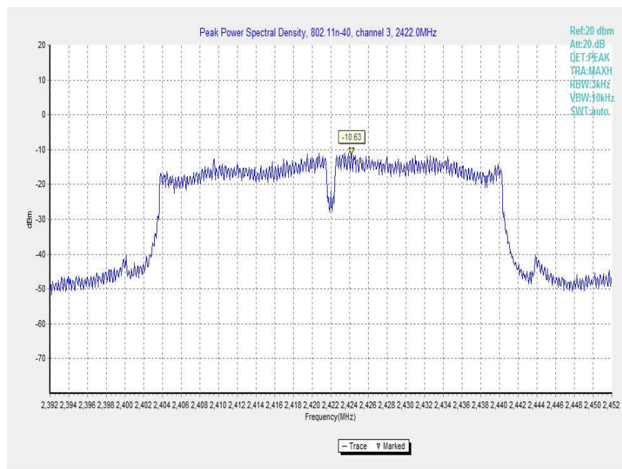
Fig.10 Power Spectral Density (802.11n-40MHz, Ch 3)
