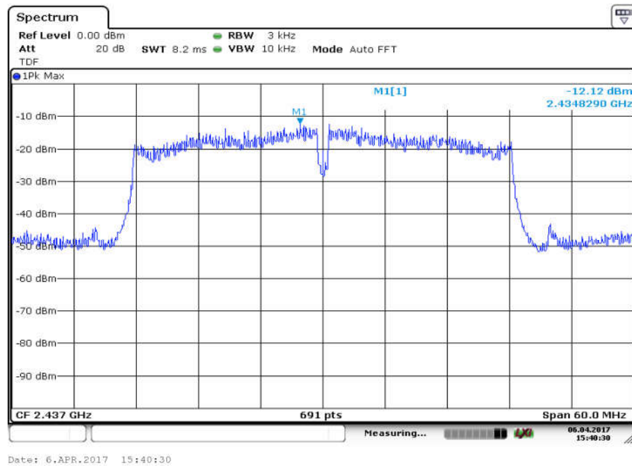
Fig.21 Power Spectral Density (802.11n-40MHz, Ch 6, MIMO Ant 1)
