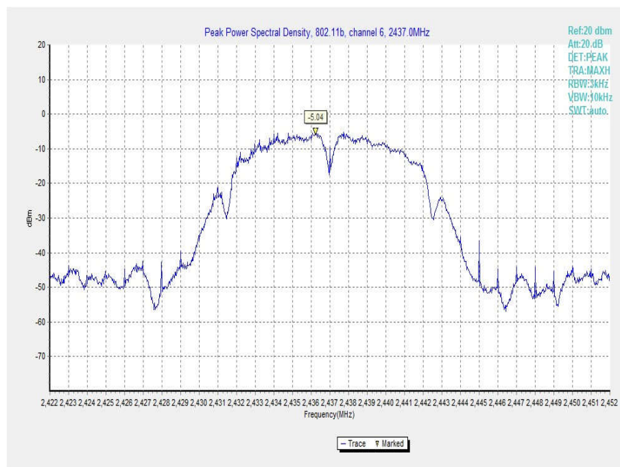
Fig.2 Power Spectral Density (802.11b, Ch 6)
