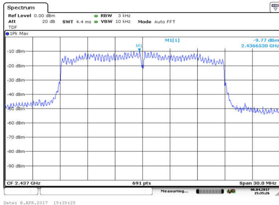
Fig.16 Power Spectral Density (802.11n-20MHz, Ch 6, MIMO Ant 2)
