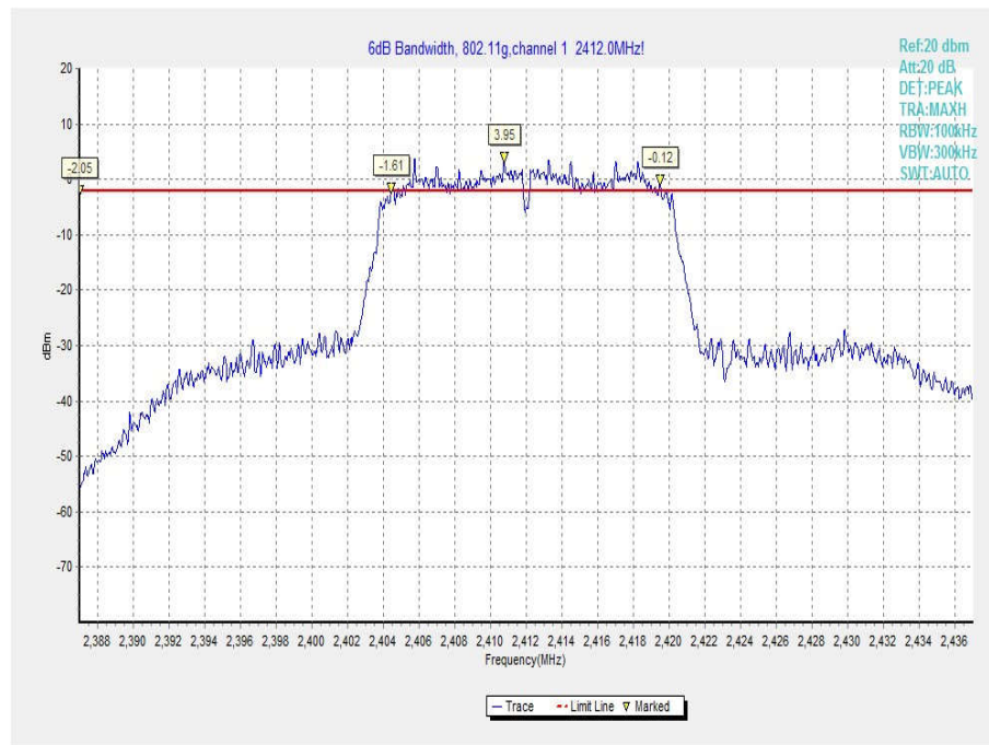
Fig.28 Occupied 6dB Bandwidth (802.11g, Ch 1)
