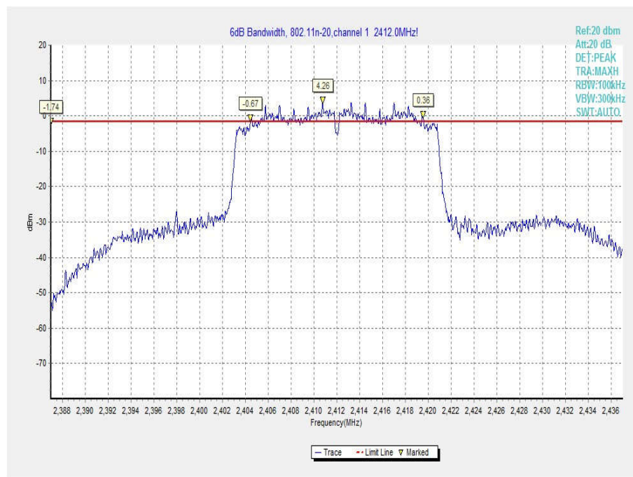
Fig.31 Occupied 6dB Bandwidth (802.11 n-20MHz, Ch 1)
