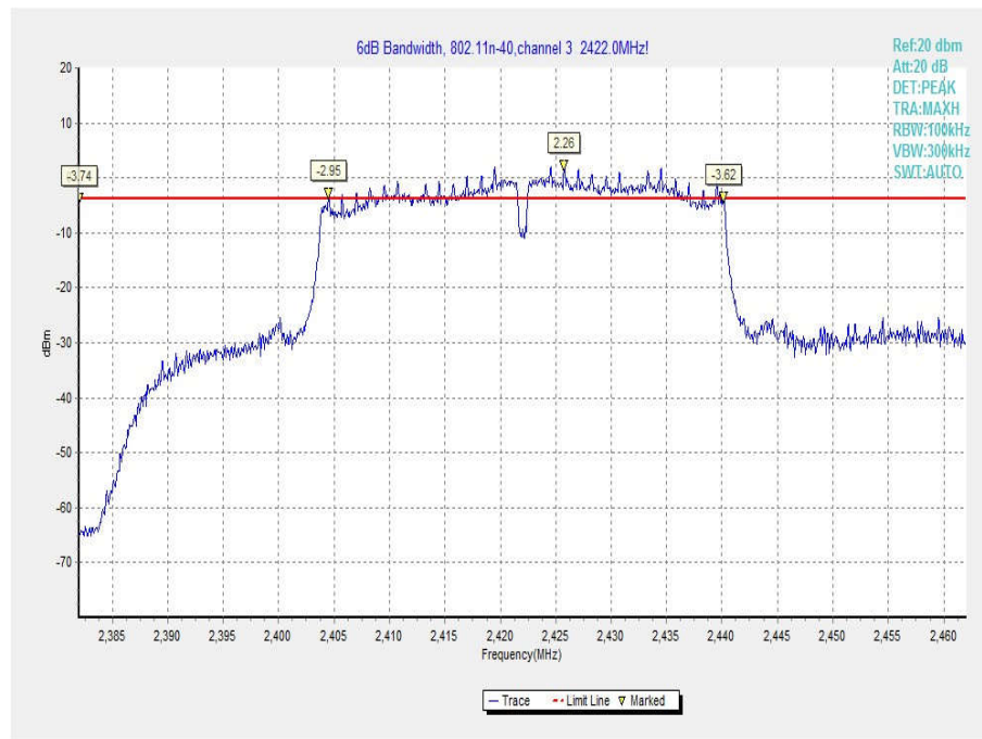
Fig.34 Occupied 6dB Bandwidth (802.11 n-40MHz, Ch 3)
