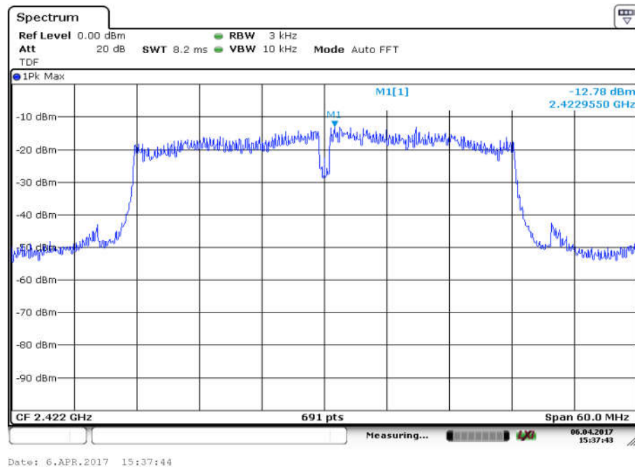
Fig.20 Power Spectral Density (802.11n-40MHz, Ch 3, MIMO Ant 2)
