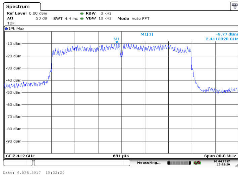
Fig.13 Power Spectral Density (802.11n-20MHz, Ch 1,MIMO Ant 1)
