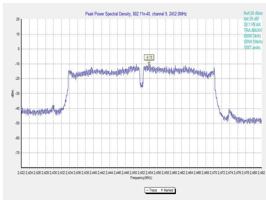
Fig.12 Power Spectral Density (802.11n-40MHz, Ch 9)
