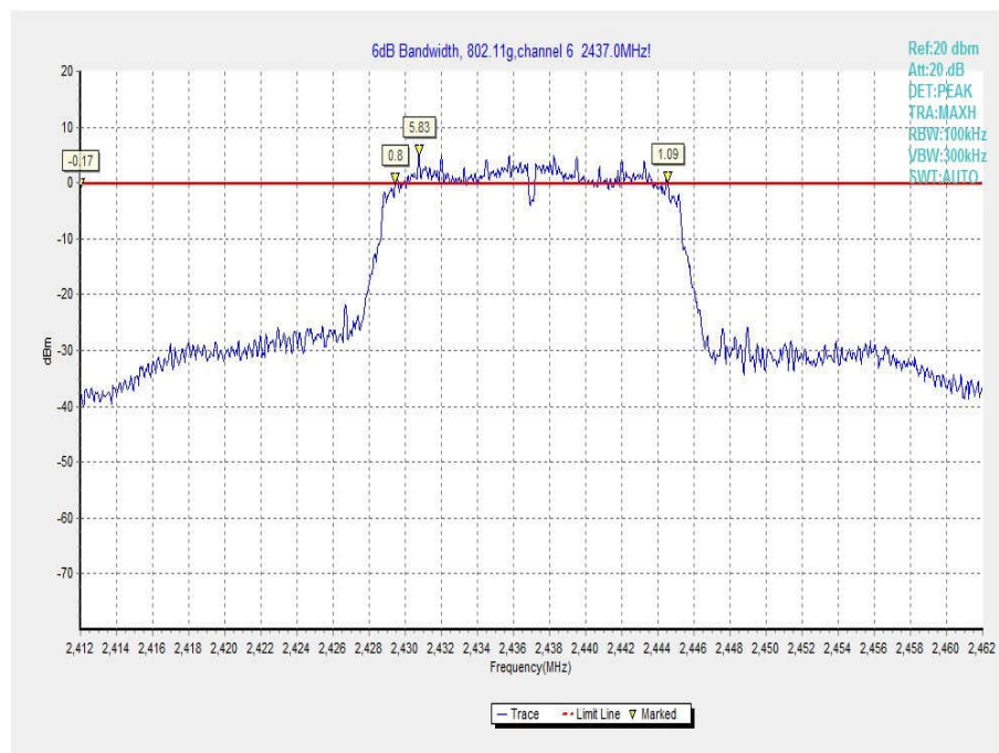
Fig.29 Occupied 6dB Bandwidth (802.11g, Ch 6)
