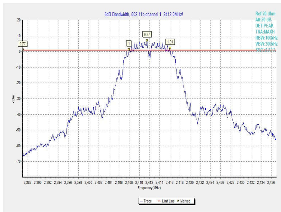
Fig.25 Occupied 6dB Bandwidth (802.11b, Ch 1)
