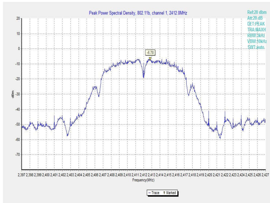
Fig.1 Power Spectral Density (802.11b, Ch 1)
