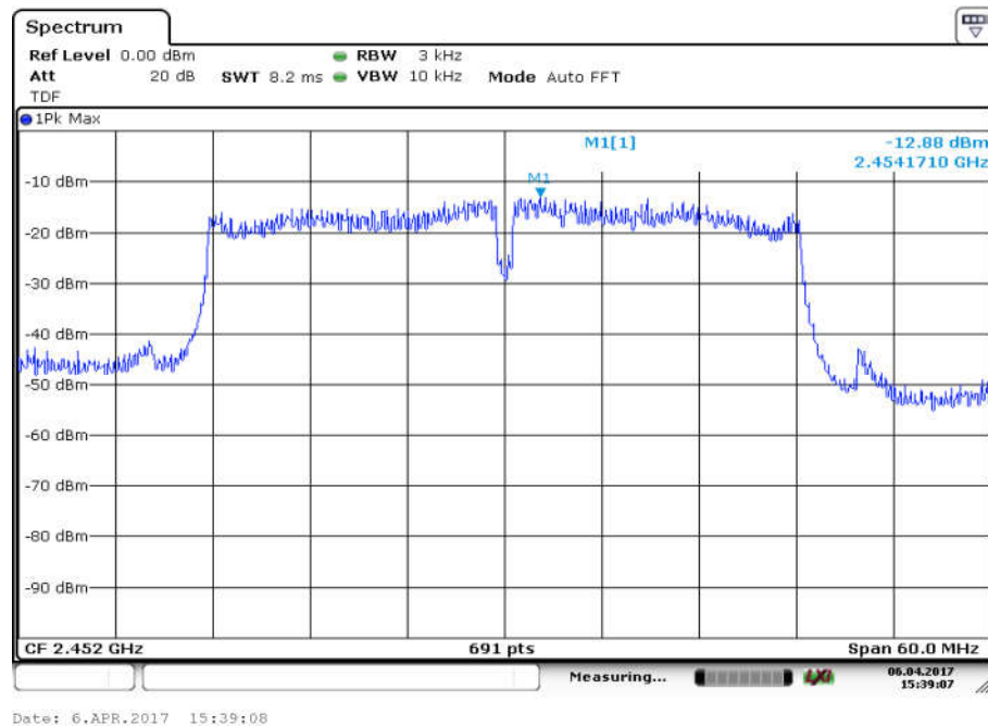
Fig.24 Power Spectral Density (802.11n-40MHz, Ch 9, MIMO Ant 2)
