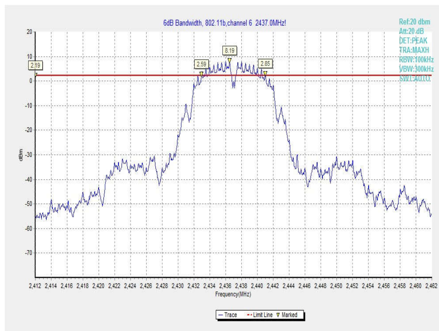
Fig.26 Occupied 6dB Bandwidth (802.11b, Ch 6)
