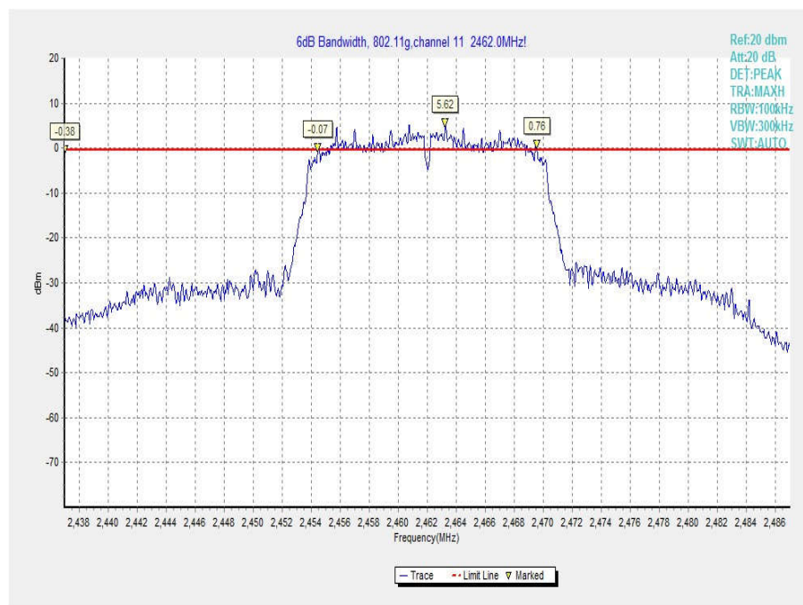
Fig.30 Occupied 6dB Bandwidth (802.11g, Ch 11)
