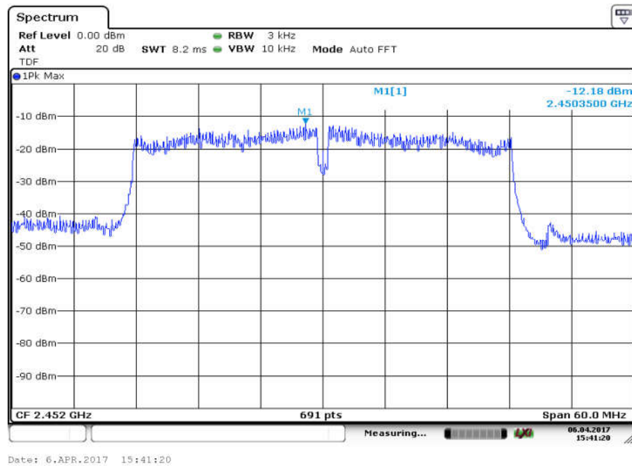
Fig.23 Power Spectral Density (802.11n-40MHz, Ch 9, MIMO Ant 1)
