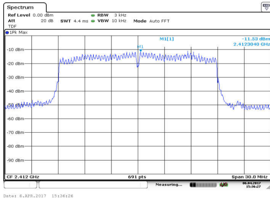
Fig.14 Power Spectral Density (802.11n-20MHz, Ch 1, MIMO Ant 2)
