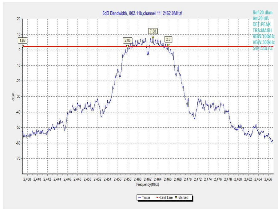
Fig.27 Occupied 6dB Bandwidth (802.11b, Ch 11)
