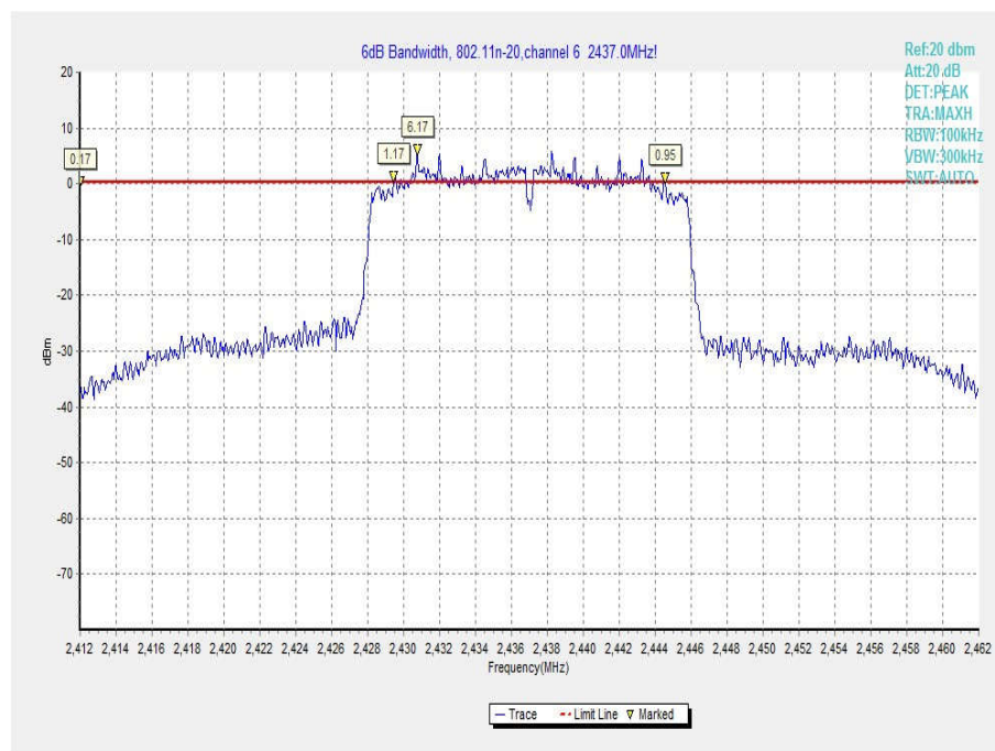
Fig.32 Occupied 6dB Bandwidth (802.11 n-20MHz, Ch 6)
