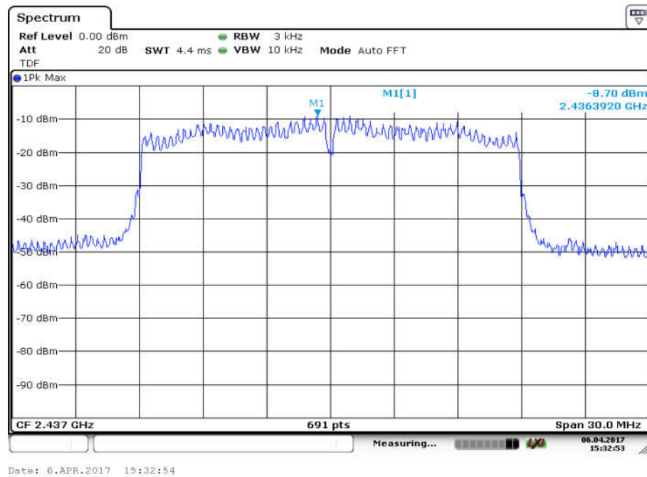
Fig.15 Power Spectral Density (802.11n-20MHz, Ch 6, MIMO Ant 1)
