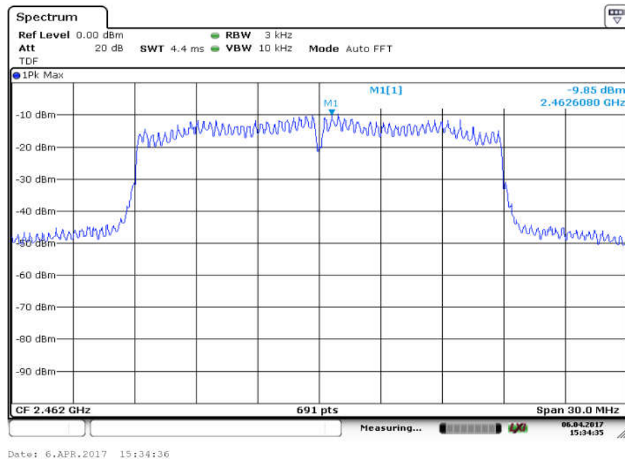
Fig.18 Power Spectral Density (802.11n-20MHz, Ch 11, MIMO Ant 2)
