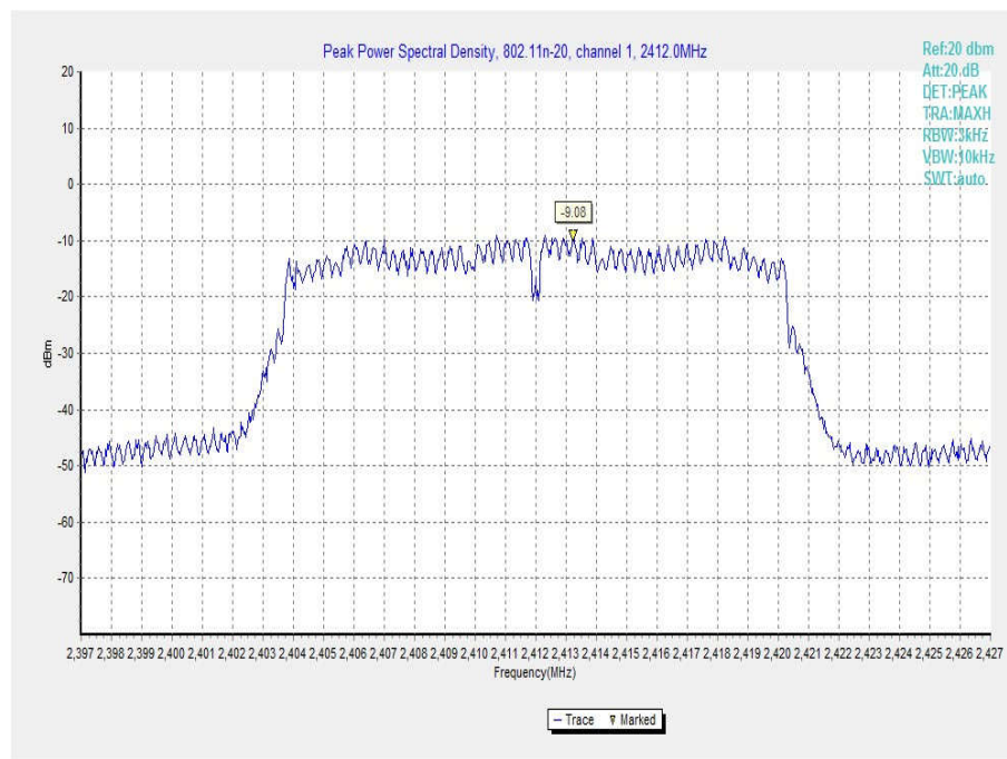
Fig.7 Power Spectral Density (802.11n-20MHz, Ch 1)
