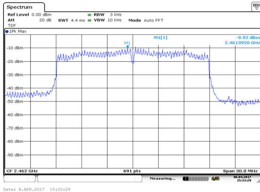
Fig.17 Power Spectral Density (802.11n-20MHz, Ch 11, MIMO Ant 1)
