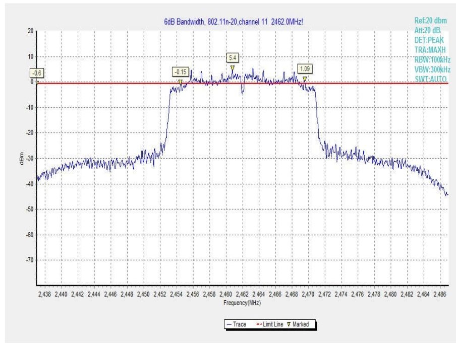
Fig.33 Occupied 6dB Bandwidth (802.11 n-20MHz, Ch 11)
