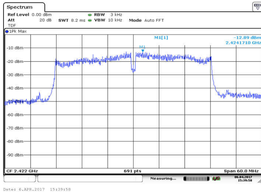
Fig.19 Power Spectral Density (802.11n-40MHz, Ch 3, MIMO Ant 1)
