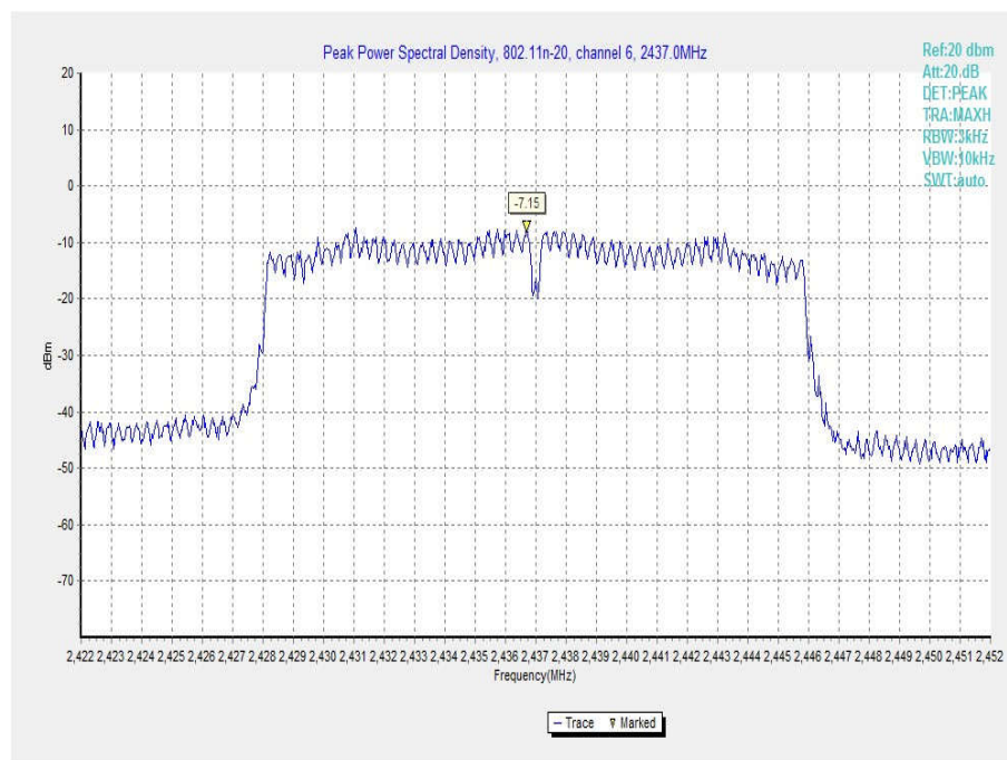
Fig.8 Power Spectral Density (802.11n-20MHz, Ch 6)
