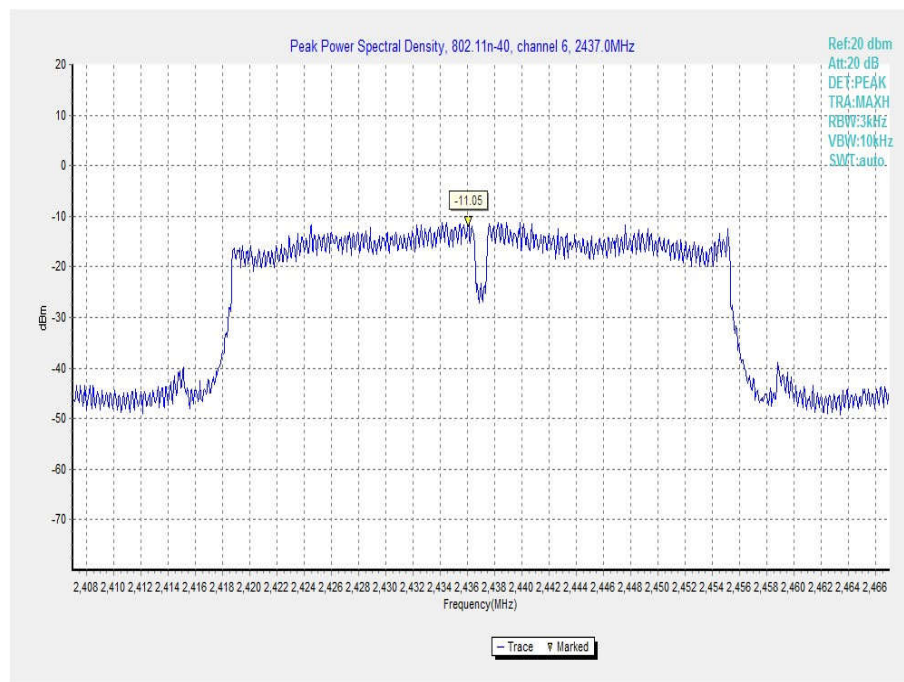
Fig.11 Power Spectral Density (802.11n-40MHz, Ch 6)
