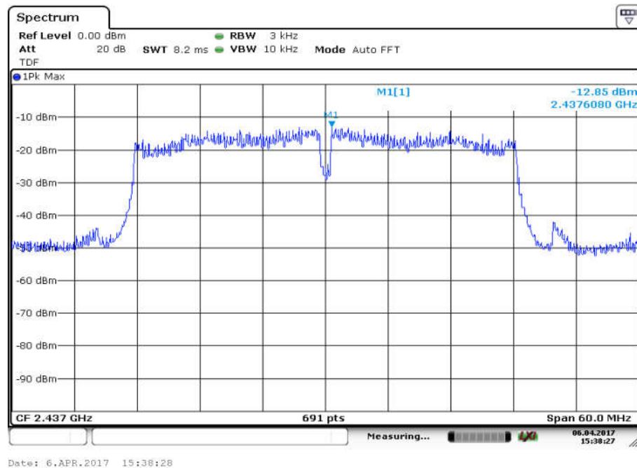
Fig.22 Power Spectral Density (802.11n-40MHz, Ch 6, MIMO Ant 2)
