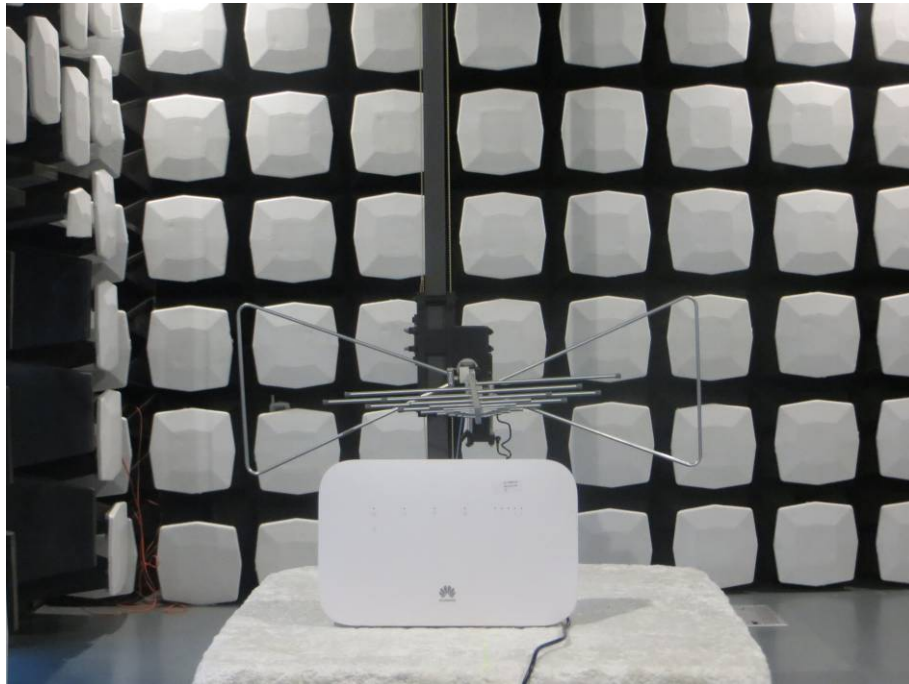
9. Radiated Emissions (Part 22/24) (below 3GHz)
