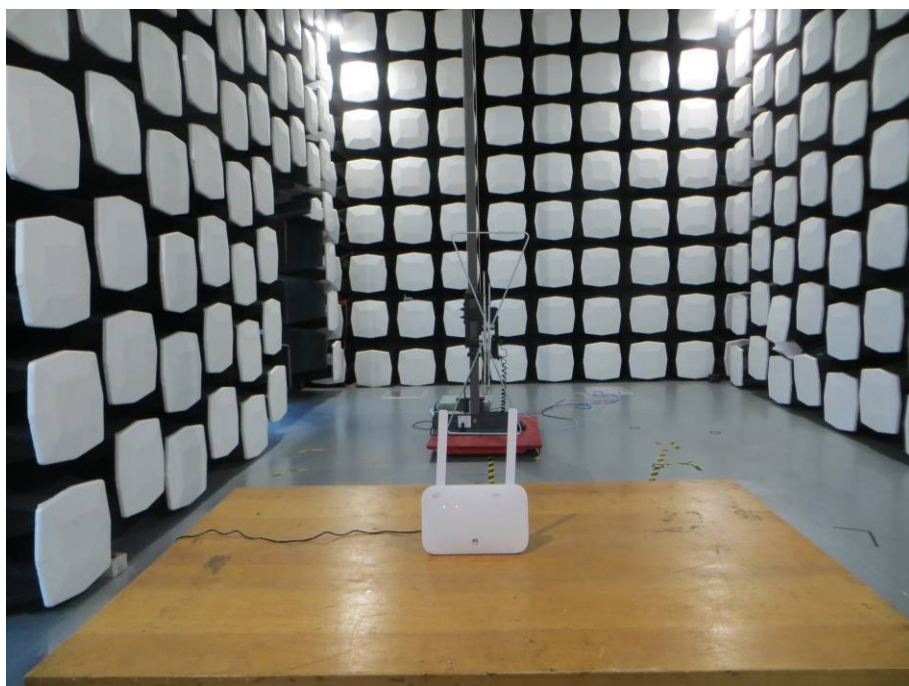
6. Radiated Emissions (Part 15C) 30M-1GHz)
