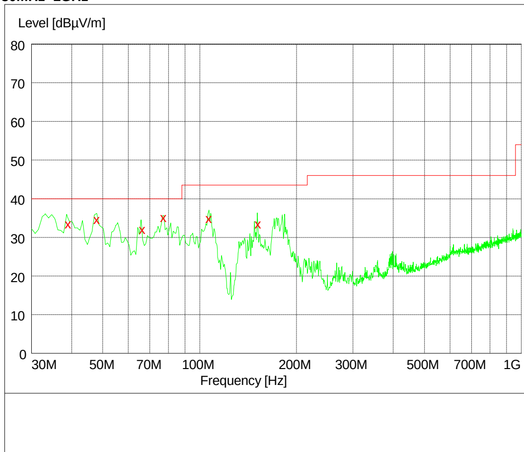
MEASUREMENT RESULT: QP Detector
