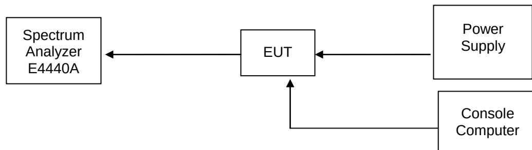
Figure 1. Test Set-up
