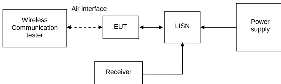
Figure 7. Test Set-up
