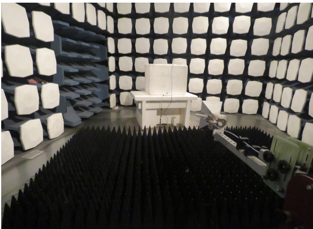
Above 1GHz
