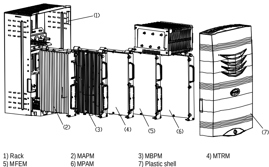
Figure 2-1 BTS structure
