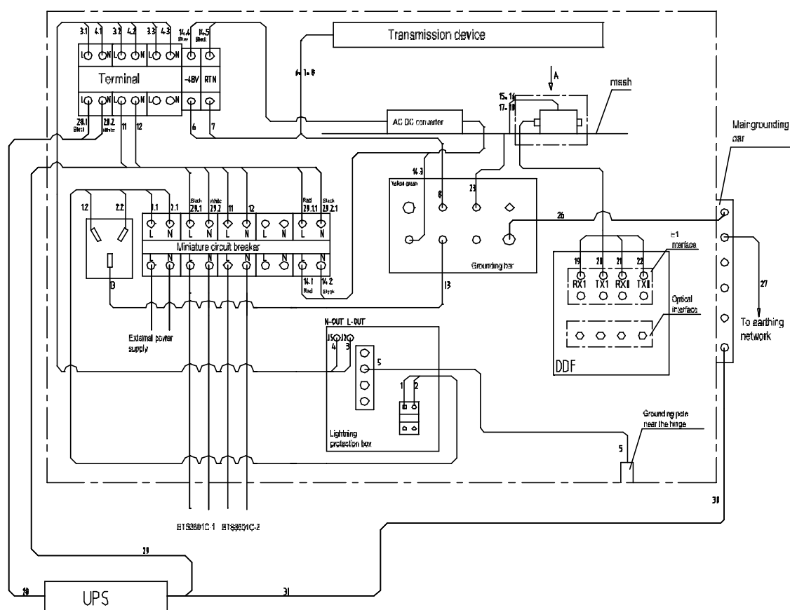
Figure 2-57 Cable distribution in IAFB networking
