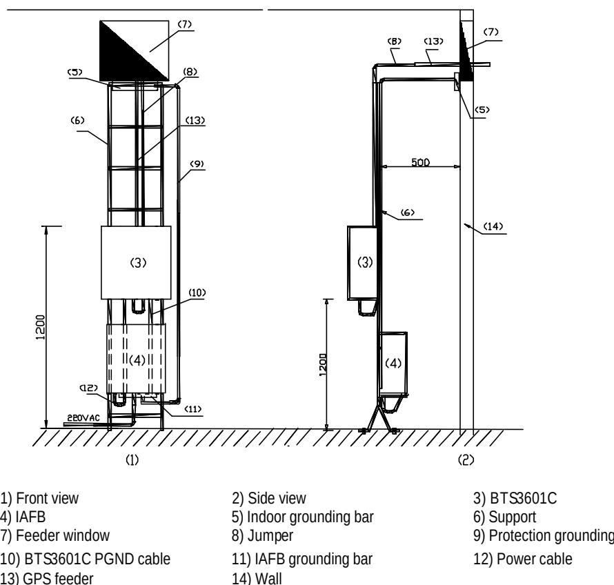
Figure 2-4 Installing BTS3601C on the plinth
