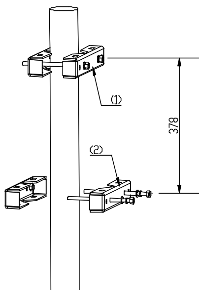
1) Fastener set 1
