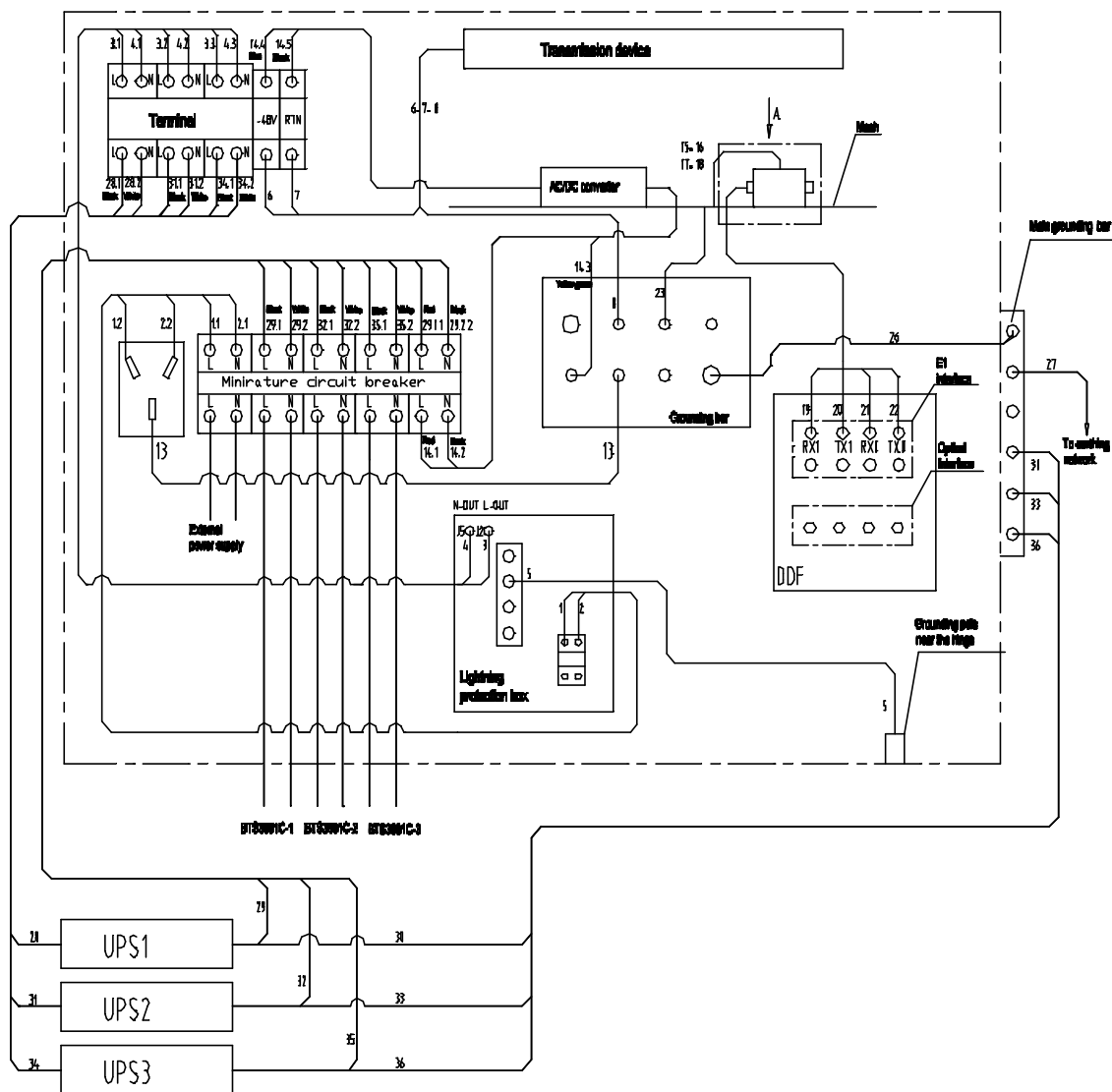
Figure 2-61 Cable distribution in IAFB networking (3 BTS3601Cs with UPS)
