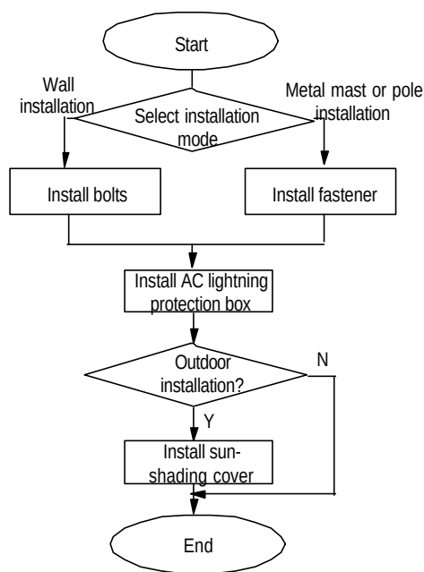
Figure 2-34 Installation flow of AC lightning protection box
