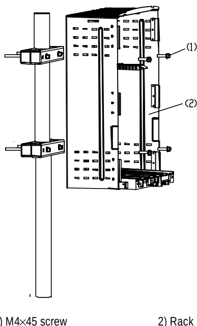
Figure 2-20 Fixing the rack
