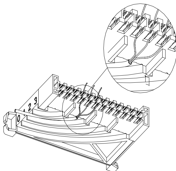
Figure 4-10 Cabling diagram after 120 \Omega DDF unit is installed (b)
