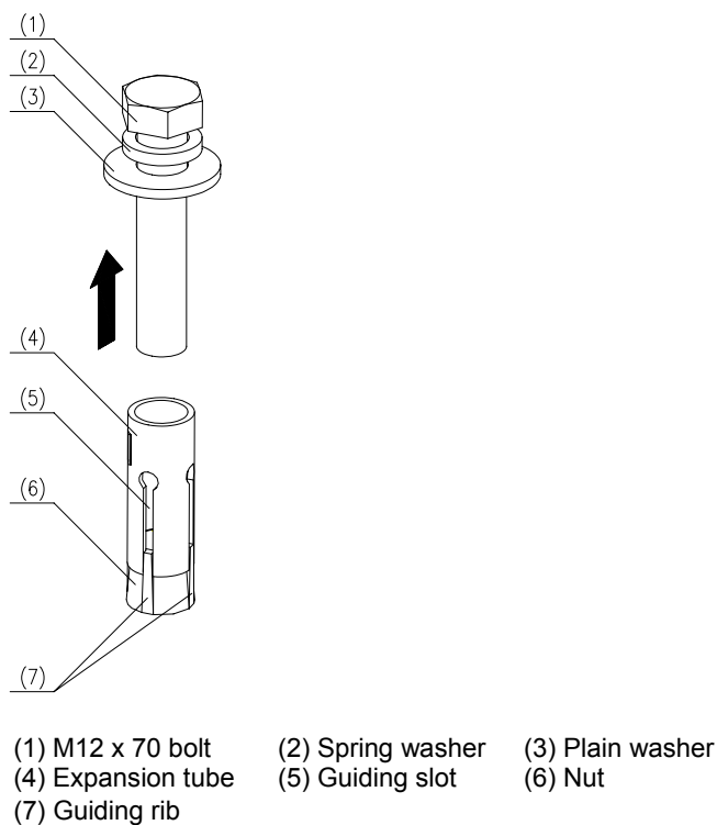
Figure 2-10 Disassembling expansion bolts
