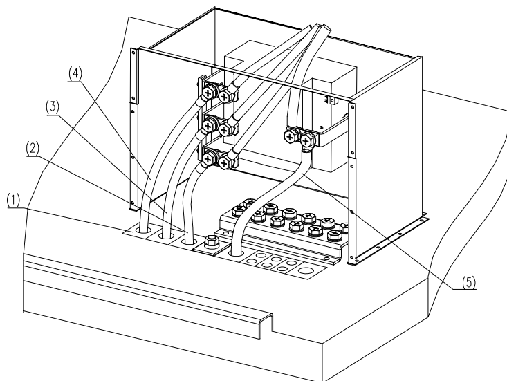
(1) Cable inlet/outlet (2) L1 line (3) L2 line (4) L3 line (5) N line
