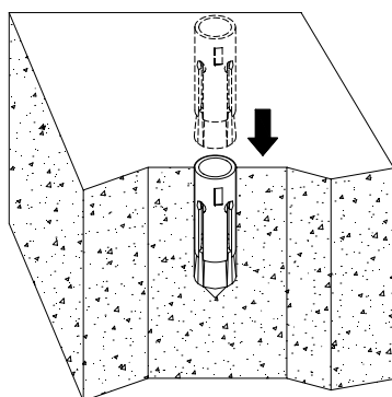
Figure 2-11 Installing the expansion bolt and expansion tube
