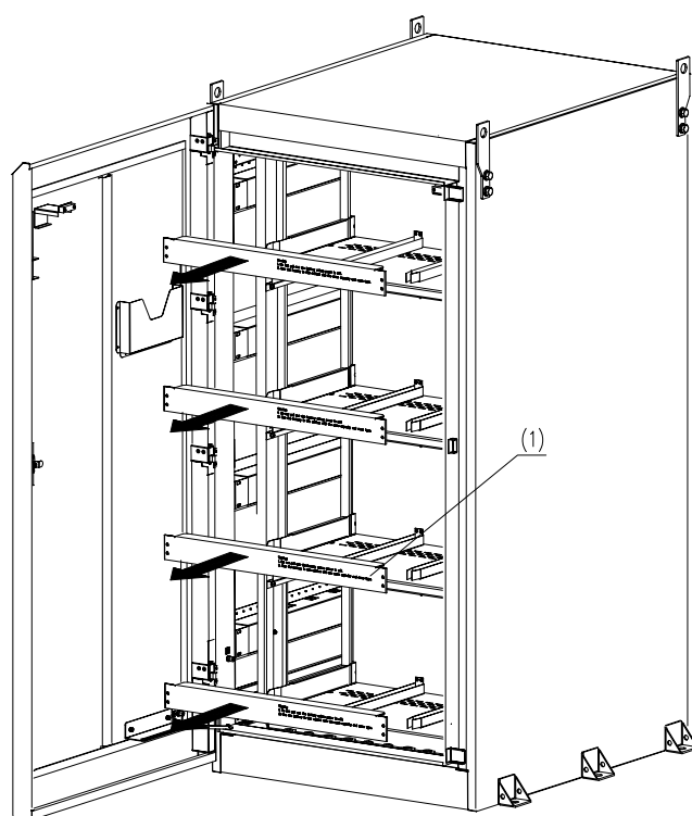
(1) Baffle plate
