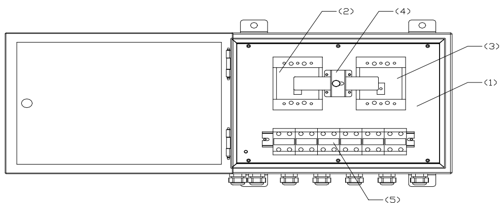
Figure 4-3 Internal structure of PSI power interface box
