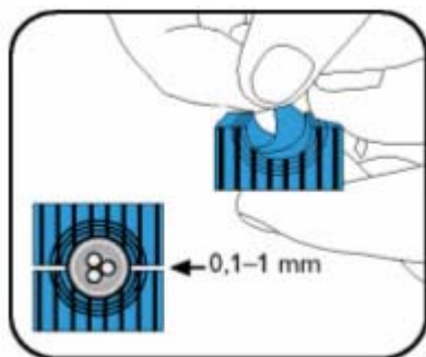
Figure 5-26 Stripping the core layer
