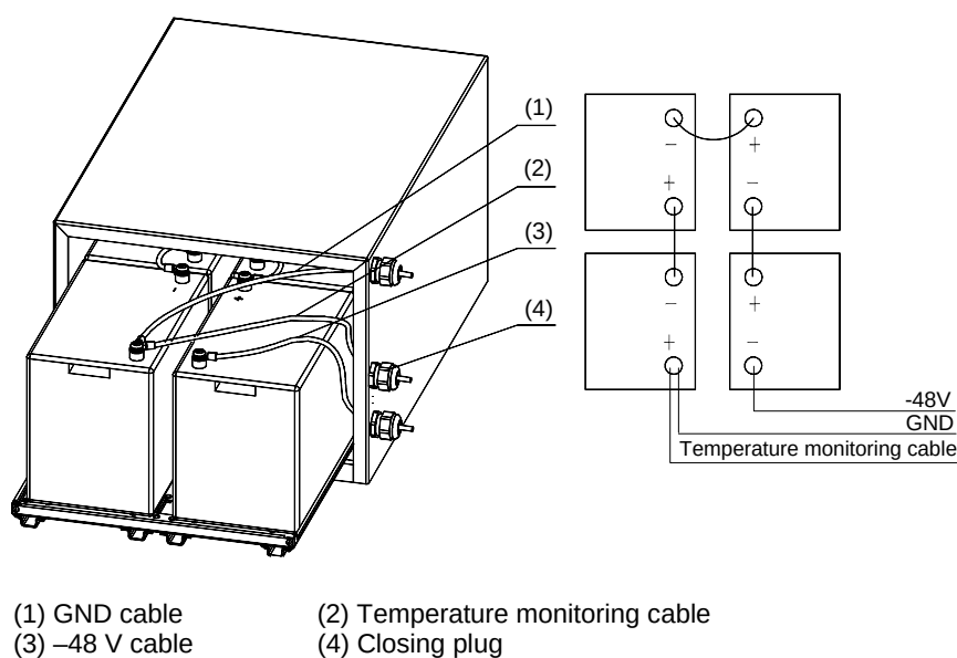
Figure 5-51 Connecting the rest cables
