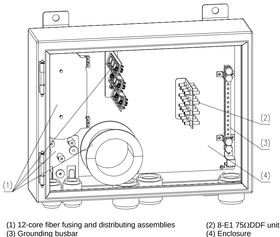
Figure 4-1 Structure of 75 \Omega transmission interface box
