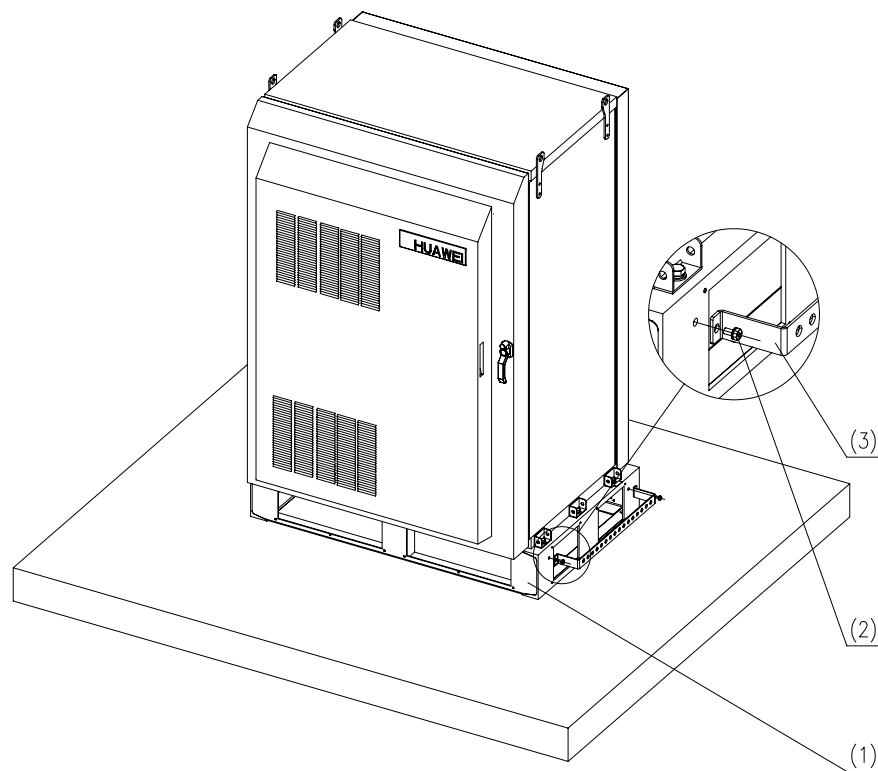
Figure 3-7 Mounting cabling rack
