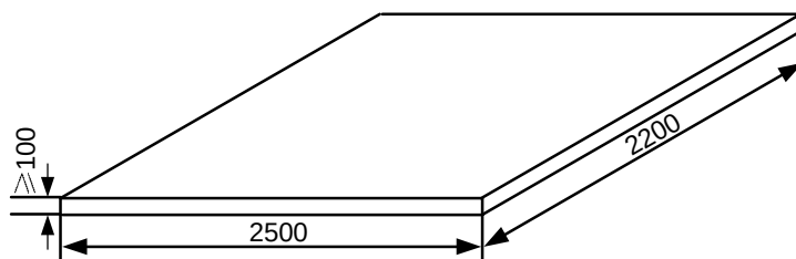
Figure 1-1 Dimensions of cement base of BTS3606A single cabinet (unit: mm)
