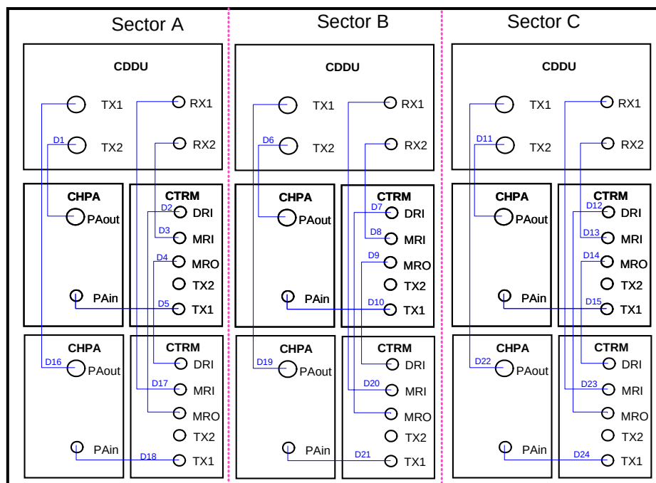
Figure 5-9 S(2/2/2) configuration
