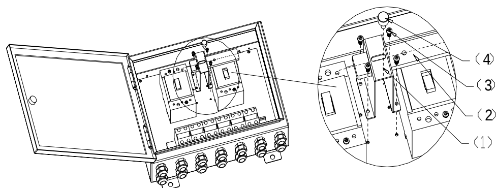
Figure 4-16 Mounting air breaker interlock device
