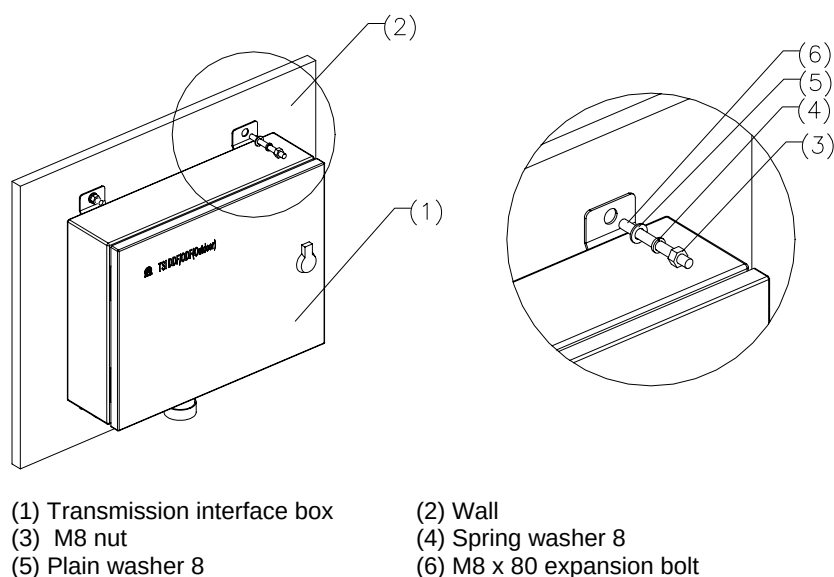
Figure 4-6 Mounting transmission interface box on the wall
