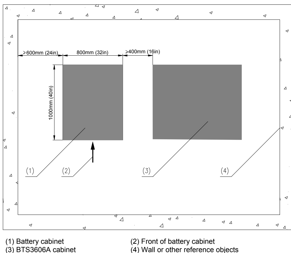
Figure 2-5 Installation position for a battery cabinet
