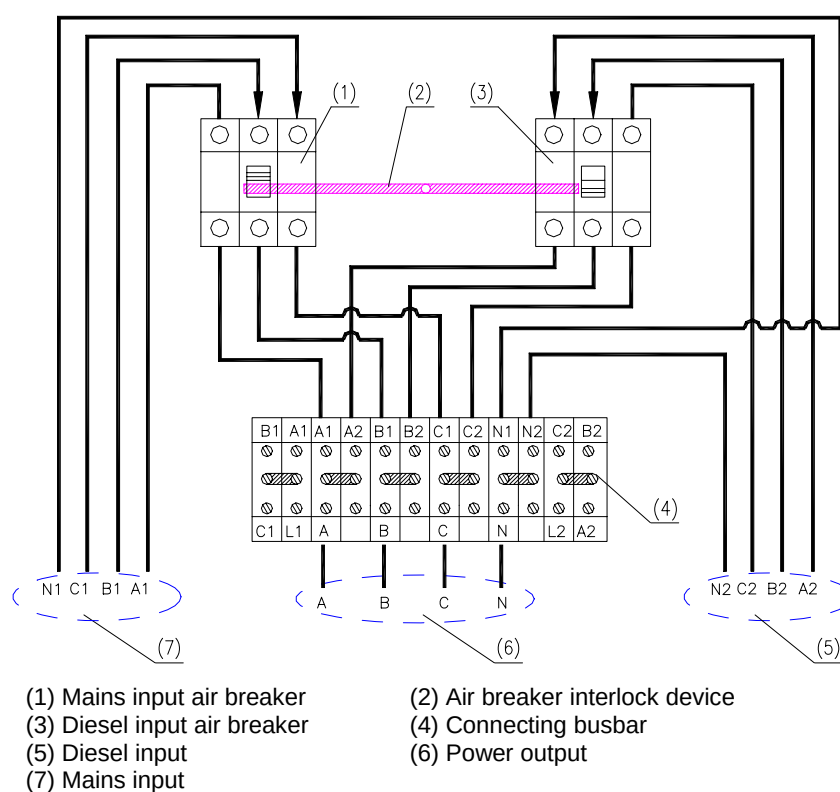
Figure 4-21 Input of three-phase mains and three-phase diesel
