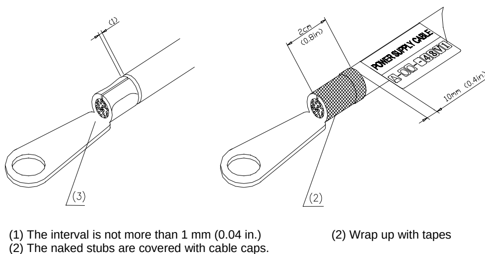
Figure 5-38 Making lugs
