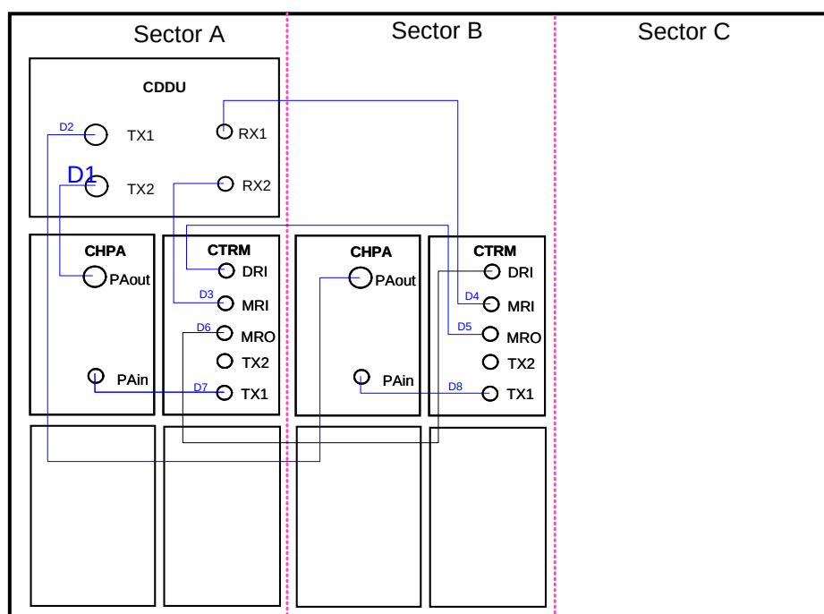
Figure 5-7 O(2) configuration
