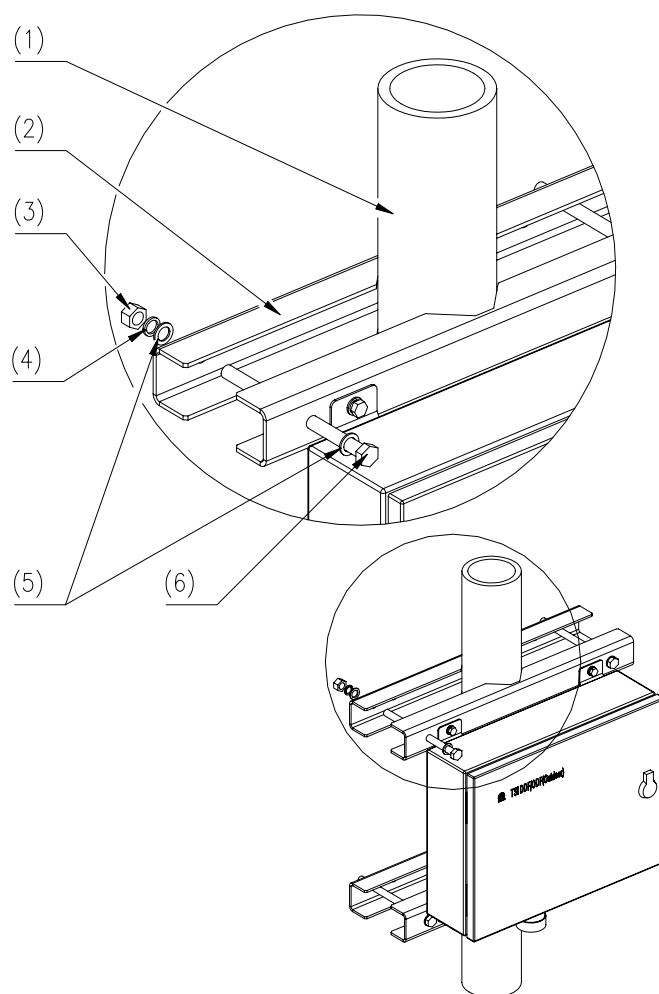
(1) Steel pole (2) Beam (3) M10 nut (4) Plain washer 10 (5) Spring washer 10 (6) Long M10 bolt
