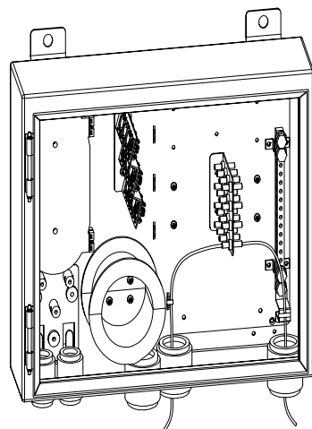
Figure 4-11 Cabling diagram after 75 \Omega DDF unit is installed
