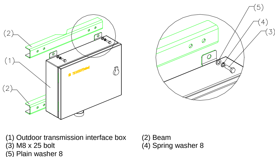
Figure 4-7 Assembling the beam
