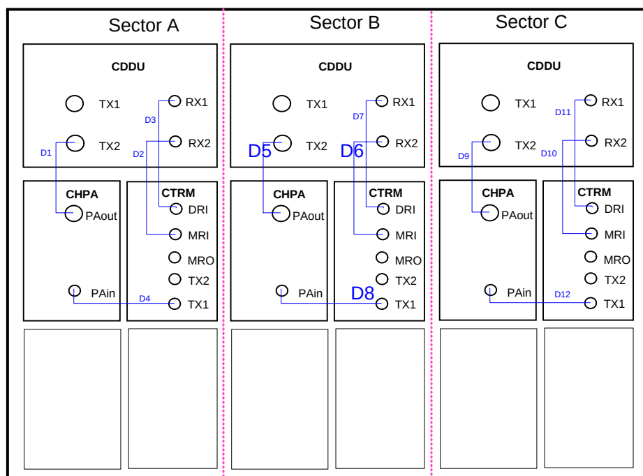
Figure 5-8 S(1/1/1) configuration
