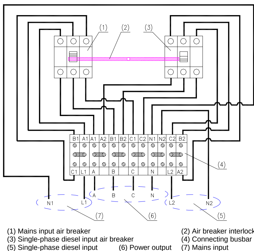
Figure 4-19 Input of single-phase mains and diesel
