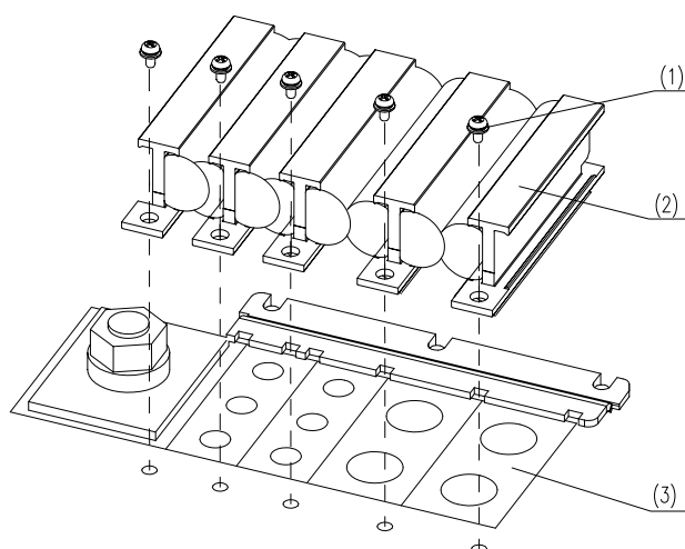
(1) M3 screw (2) Shielding clip (3) Waterproof module
