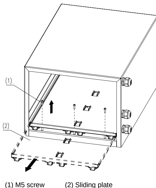
Figure 5-47 Pulling out the sliding plate
