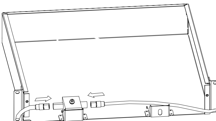
Figure 5-36 Installing GPS lightning arrester (2)
