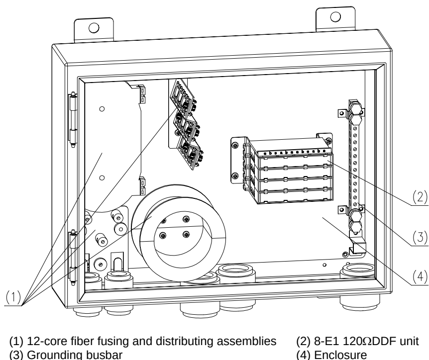
Figure 4-2 Structure of 120Ω transmission interface box
